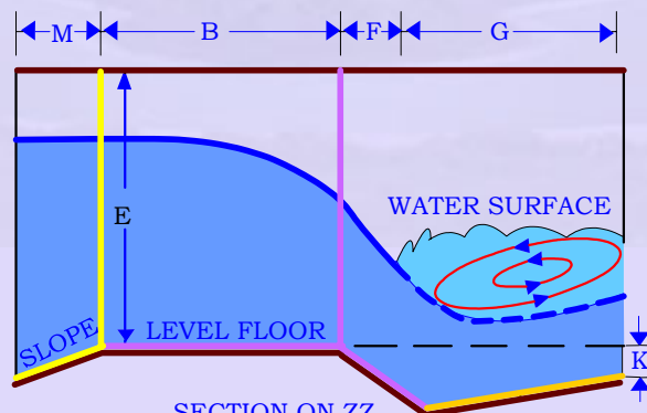
SECTION ON ZZ PARSHALL FLUME
