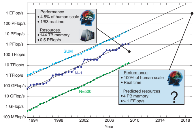
Figure 8: Growth of Top500 supercomputers [25] overlaid with our result and a projection for realtime human-scale cortical simulation.
