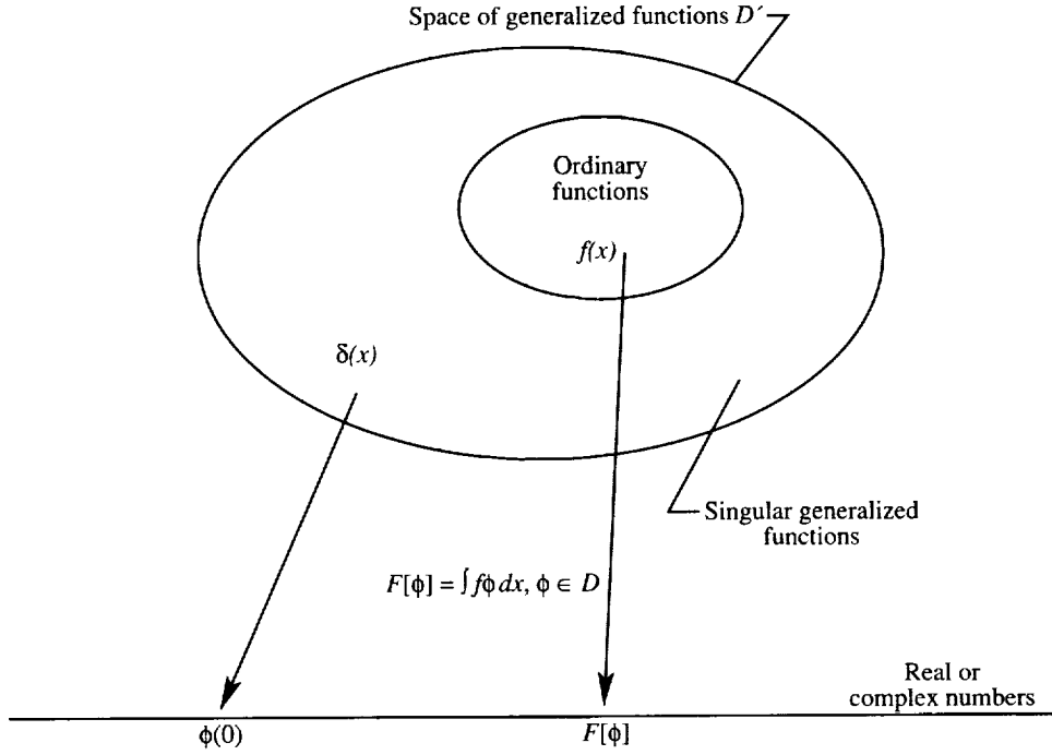
Figure 1. Generalized functions are continuous linear functionals on space D of test functions.
