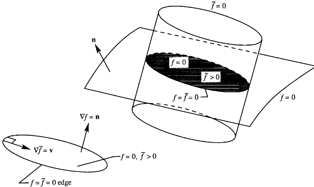
Figure 9. Definition of open surface by relations f = 0, \tilde{f} > 0 . Edge is defined by f = \tilde{f} = 0 and \nu is the unit inward geodesic normal.
