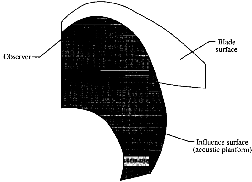
Figure 10. Influence surface for observer on propeller surface, forward Mach number = 0.334, helical Mach number = 0.880. (See ref. 44.)
