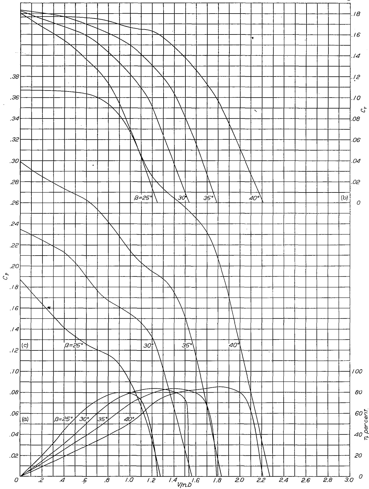
(a) Propulsive efficiency (b) Thrust coefficient (c) Power coefficient
