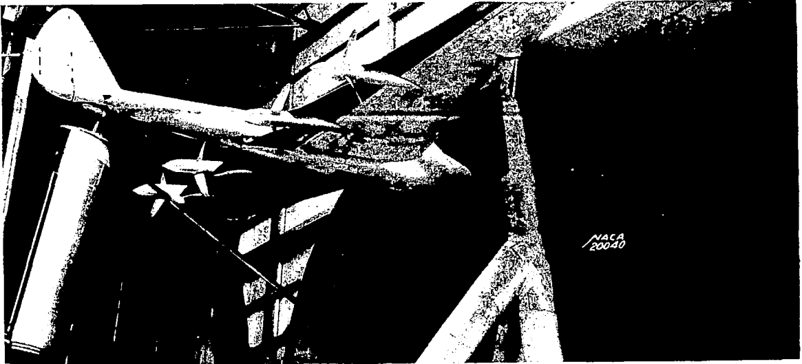
Figure 1.- The four-engine airplane model installed in the full-scale tunnel with special pusher propellers and twisted flaps.
