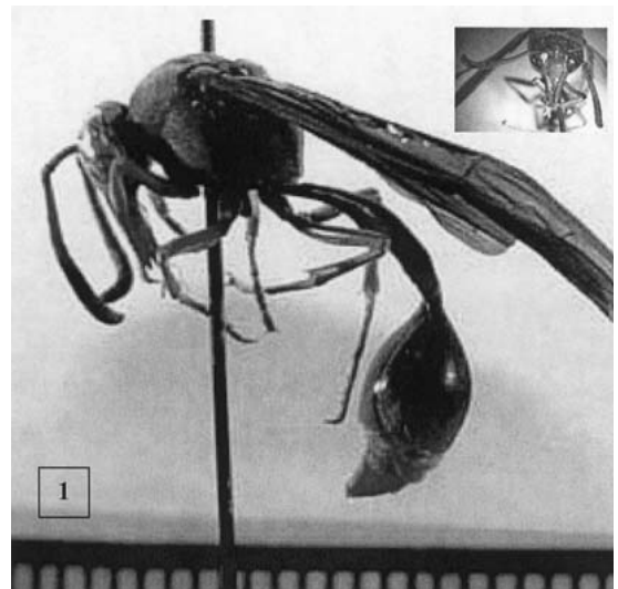
Fig. 1. Zeta argillaceum female, lateral view. Ruler marking are in mm. Inset is portrait of head, frontal view.
