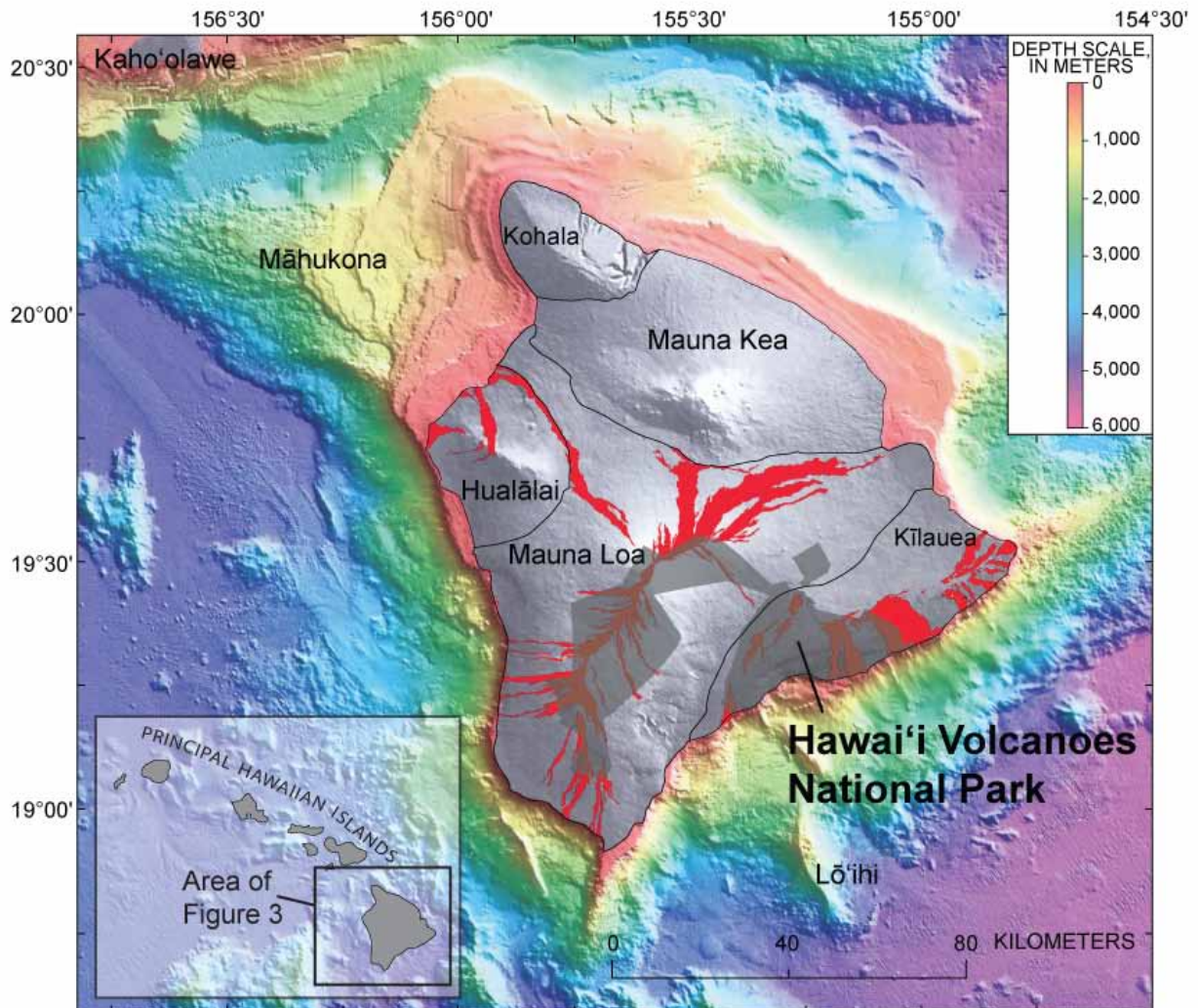
Figure 3. Map of the Island of Hawai'i and surrounding ocean floor. Note locations of the five volcanic centers on the island as well as benthic (sea floor) morphology. Gray areas are exposed land; red areas are historical lava flows. USGS graphic excerpted from map by Eakins and others (2003).
