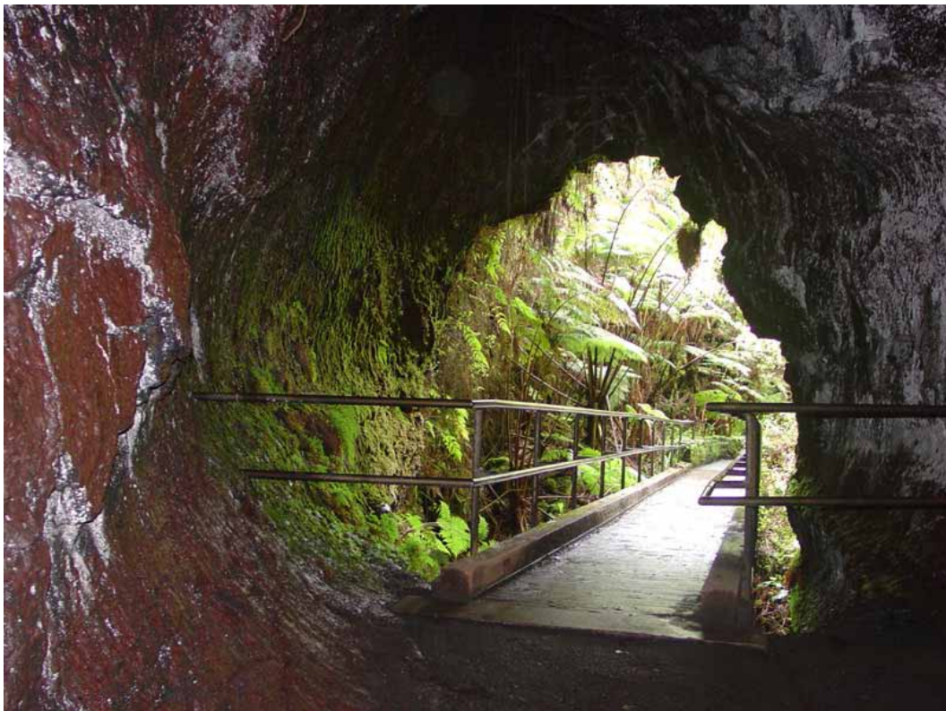
Figure 20. View out of the entrance to Thurston Lava Tube. USGS photograph available at http://3dparks.wr.usgs.gov/havo/ .
