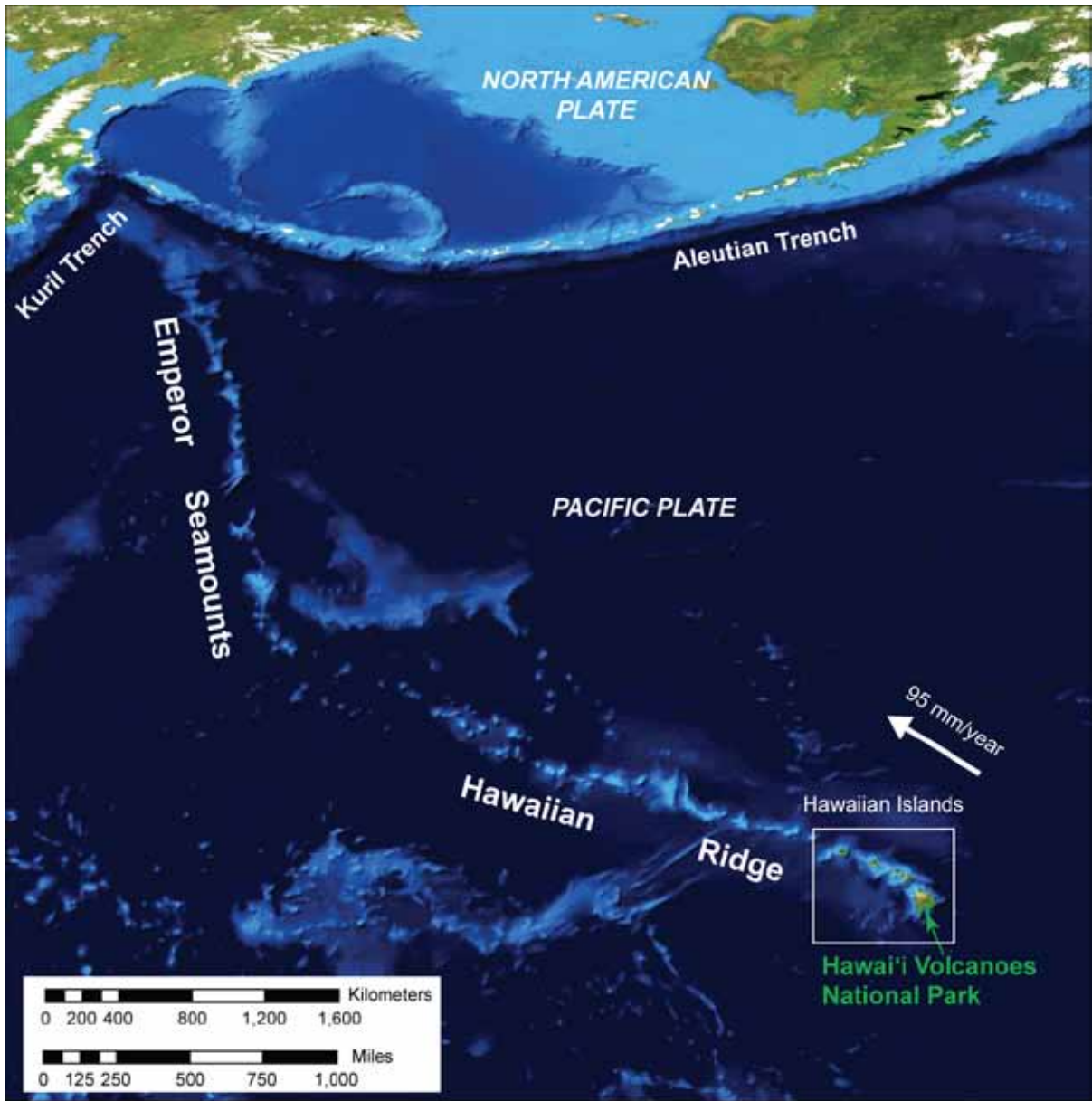
Figure 4. Aerial imagery of the northern Pacific Ocean basin, with deeper areas appearing dark blue to black and the Hawaiian-Emperor volcanic chain (and other relatively shallow areas) visible as lighter blue areas. The white box encloses the Hawaiian Islands. The white arrow indicates present motion of the Pacific plate at 95 mm/year (3.74 inches/year). Compiled by Jason Kenworthy (NPS Geologic Resources Division) from ESRI Arc Image Service, USA Prime Imagery with information from Eakins and others (2003).
