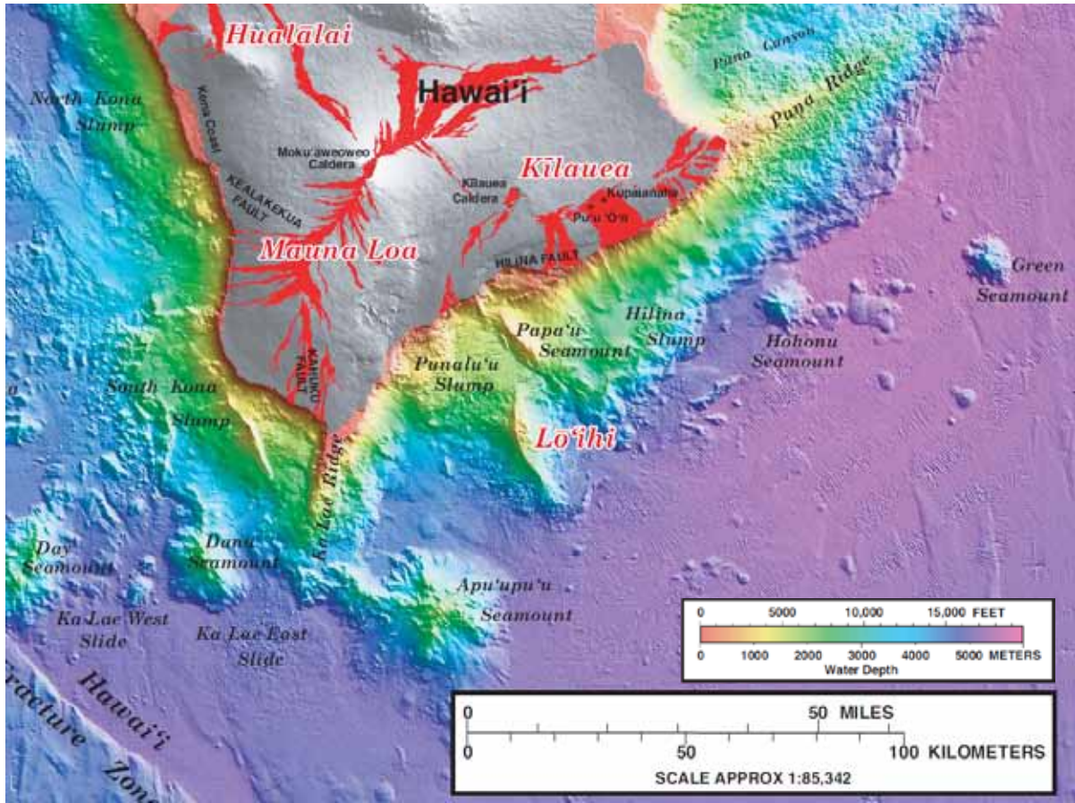
Figure 10. Bathymetric map of the south coast of Hawai'i showing the locations of the Hilina and Punalu'u slumps. USGS graphic excerpted from Eakins and others (2003).
