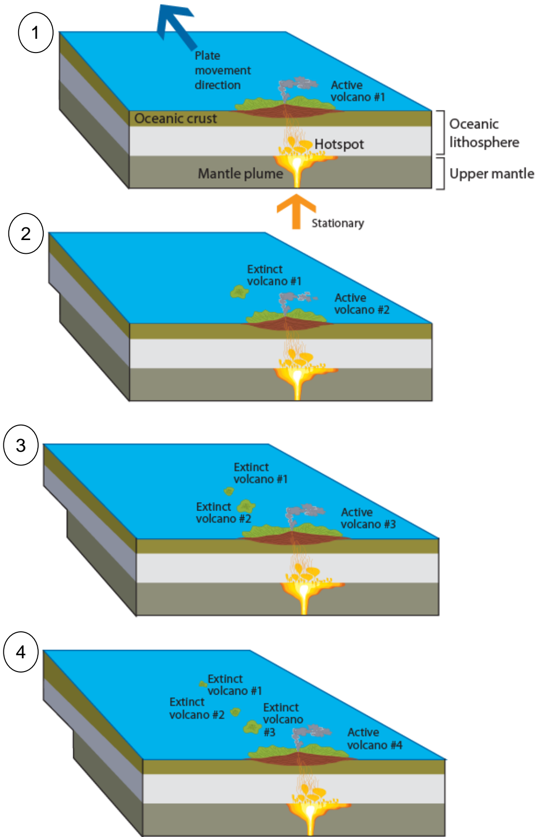
Figure 25. Evolution of a chain of islands over a stationary hotspot in Earth's crust. Graphic is by Trista L. Thornberry-Ehrlich (Colorado State University).
