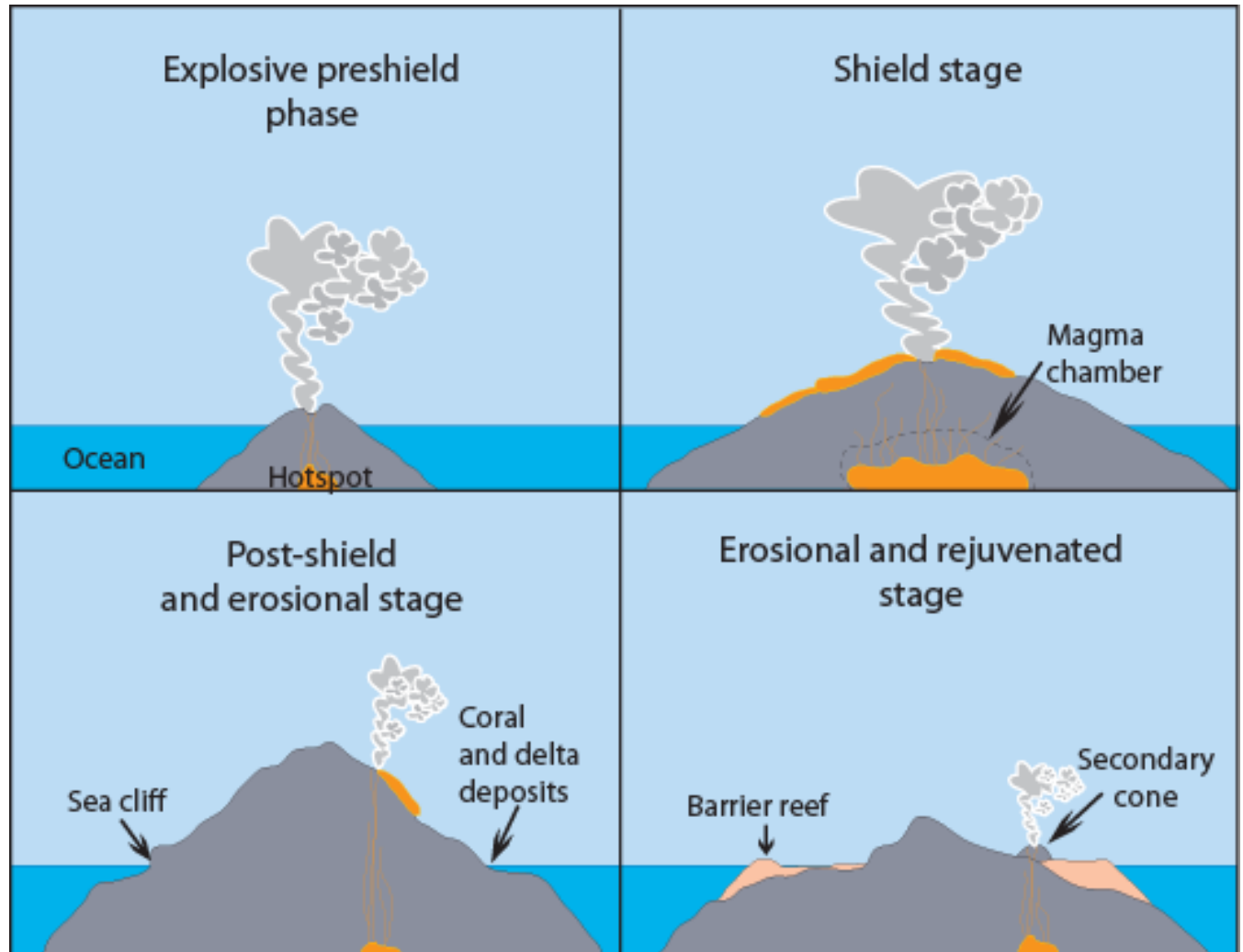
Figure 27. Simplified stages of Hawaiian hotspot island volcanism. After volcanism ceases, erosion and subsidence slowly reduce the island to a submarine stump. Graphic by Trista L. Thornberry-Ehrlich (Colorado State University), after Keating (1992, fig. 29).
