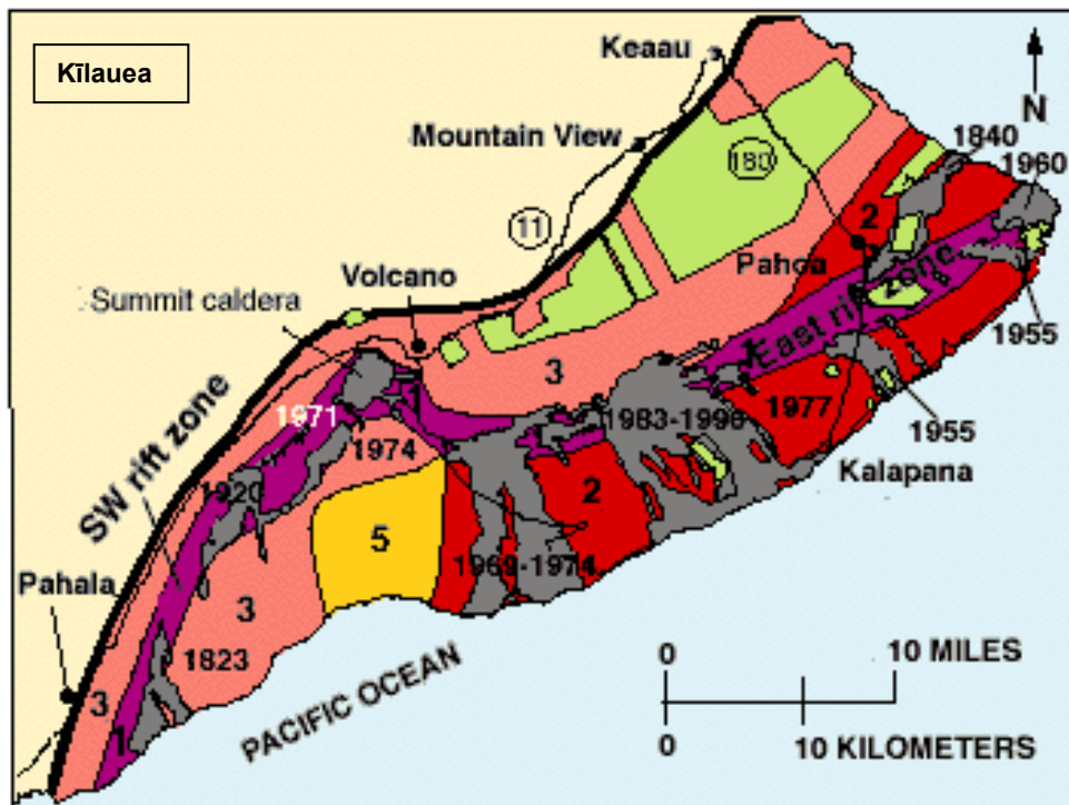
Figure 6. Maps showing volcanic-hazard zones for Mauna Loa (top) and Kilauea (bottom). The island is divided into zones 1–9 (defined in Heliker, 1990) according to the likelihood of being inundated by lava flows; higher numbers indicate less likelihood of inundation. Major housing subdivisions shown in green. USGS graphics extracted from Heliker (1990).
