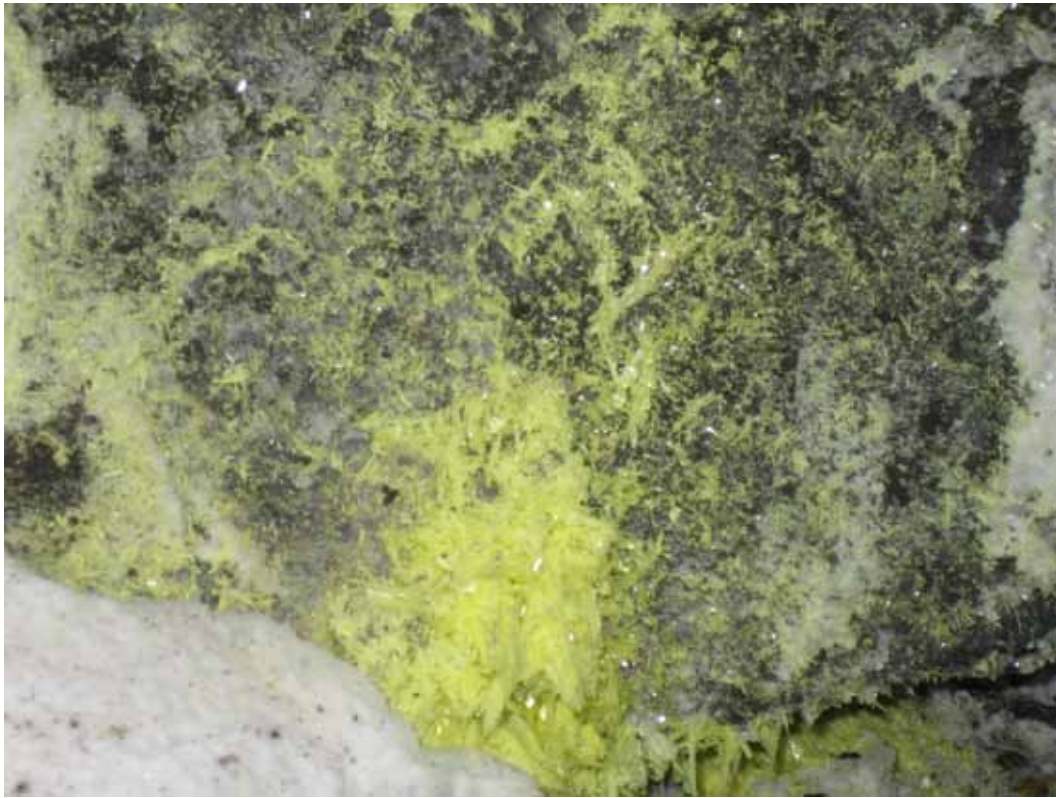
Figure 19. Secondary mineralization present as delicate sulfur crystals within a surficial cavity of a lava flow at Hawai'i Volcanoes National Park. Photograph is by Trista L. Thornberry-Ehrlich (Colorado State University), February 2007.
