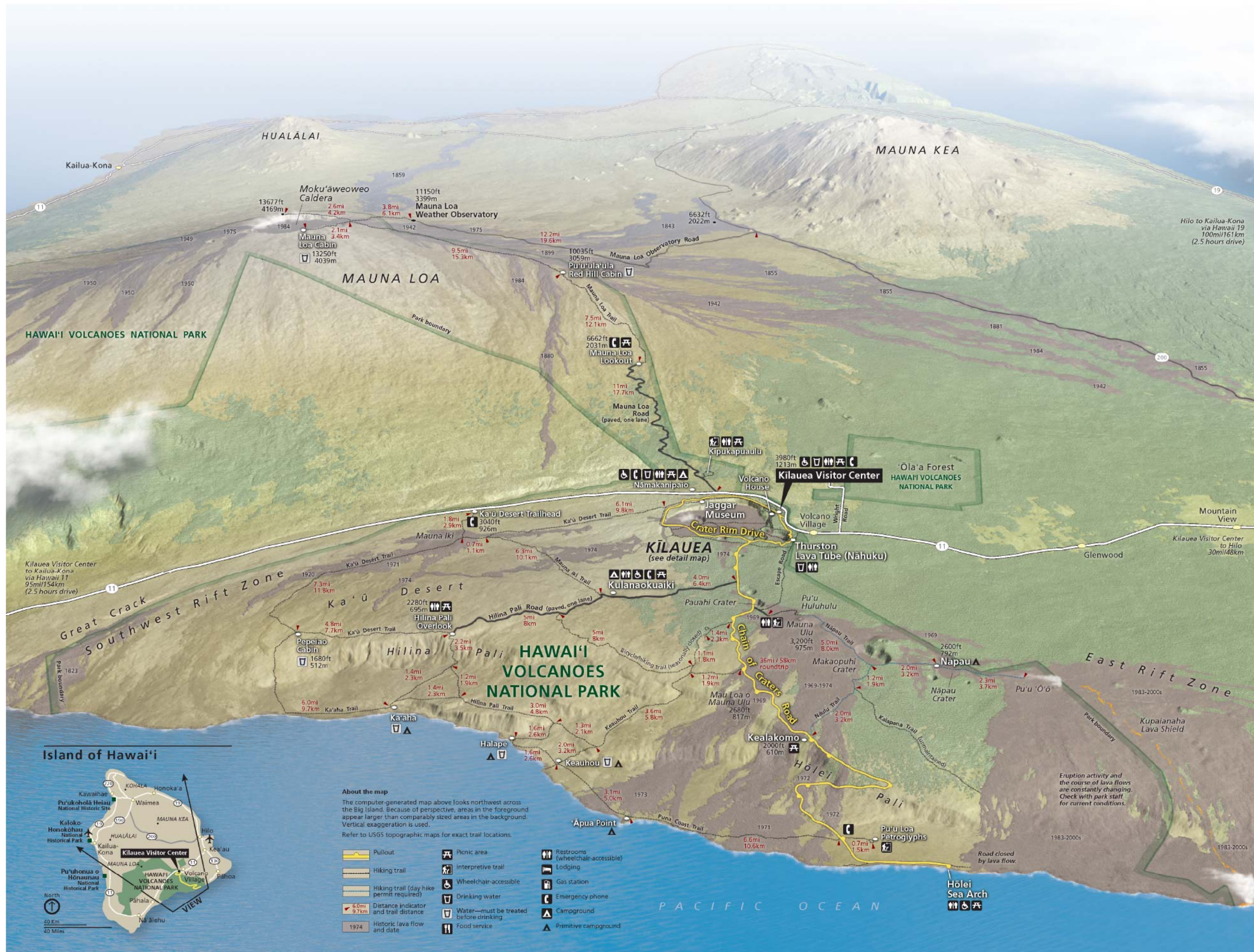
Figure 1. Map of Hawai'i Volcanoes National Park. For a map of the Kilauea area, refer to Figure 2. NPS map.
