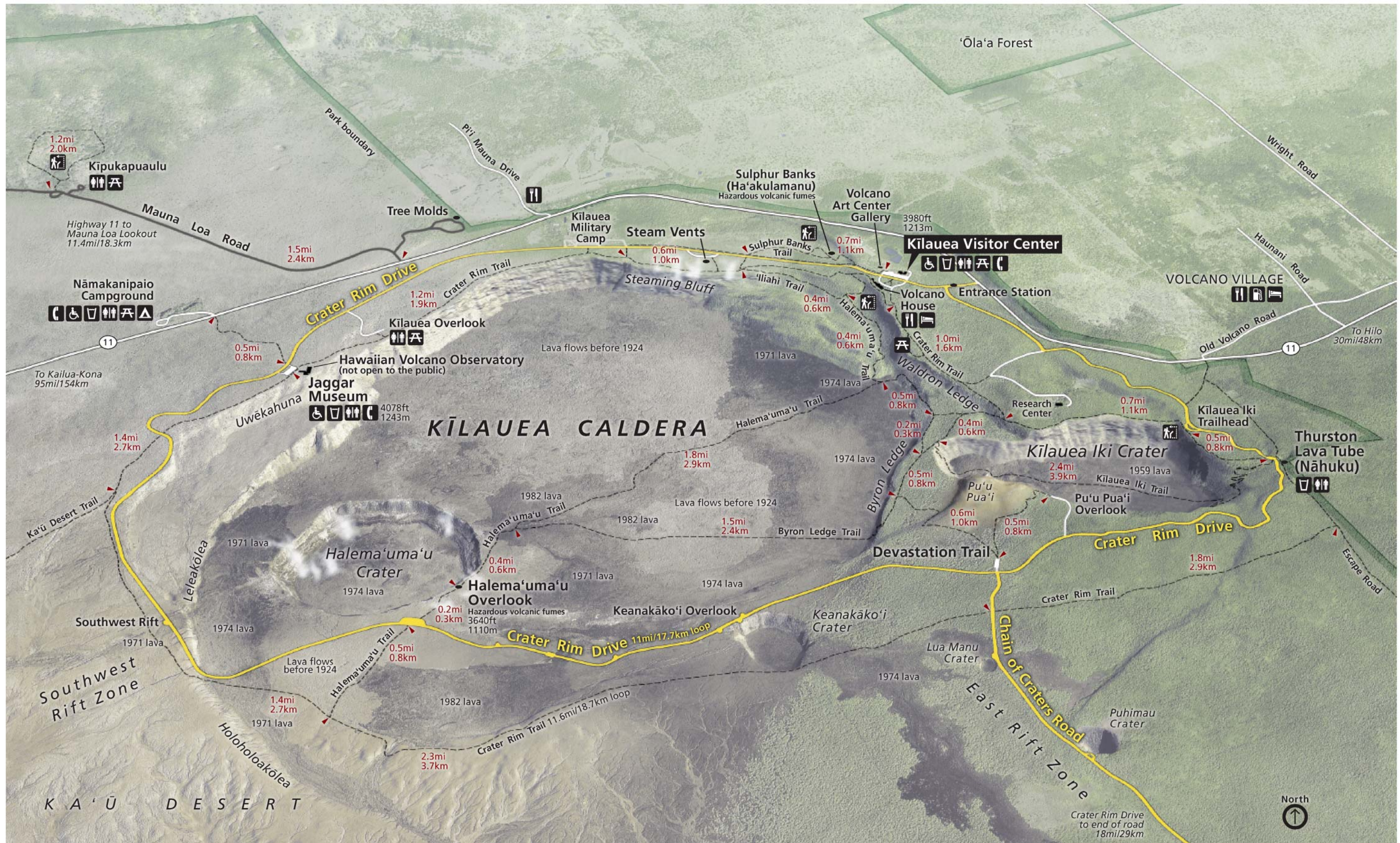
Figure 2. Map of the Kīlauea Caldera area of Hawai'i Volcanoes National Park. NPS map.
