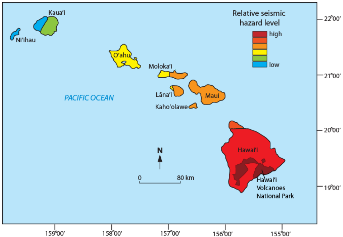
Figure 11. Map showing earthquake-hazard zones for the major Hawaiian Islands. Hawai'i Volcanoes National Park is within the area of greatest seismic hazard. Graphic was modified from Klein and others (2000) data by Rutherford and Kaye (2006) and redrafted by Trista L. Thornberry-Ehrlich (Colorado State University).
