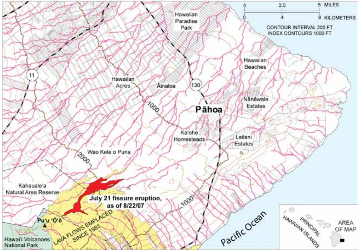
Figure 7. Map showing part of the Puna District near the Pu'u Ō'ō vent. Red area shows lava flows emplaced July–August 2007. Pink lines show modeled paths of steepest descent down topographic gulleys and valleys. Yellow area shows lava flows from Pu'u Ō'ō between 1983 and 2007. USGS graphic extracted from Kauahikaua (2007, fig. 1).
