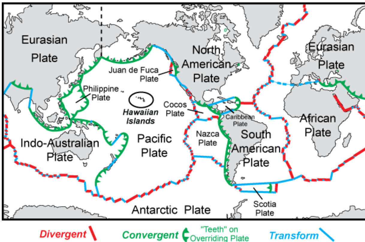
Figure 24. Map of the current tectonic plates. The Hawaiian Islands are circled. Divergent boundaries are where plates are pulling apart. Plates come together at convergent boundaries and slide past one another at transform boundaries. Graphic courtesy Robert J. Lillie (Oregon State University), modified from Lillie (2005).
