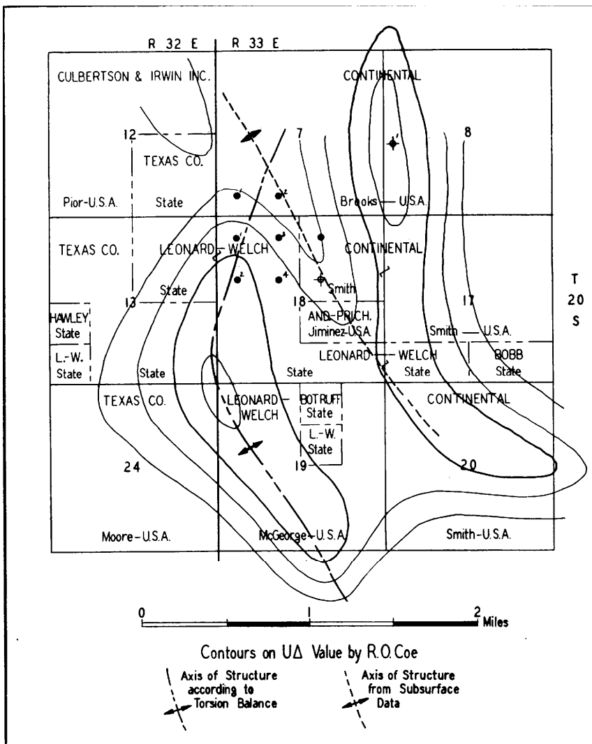
FIGURE 20.—Torsion-balance map of the Salt Lake pool, Lea County.
