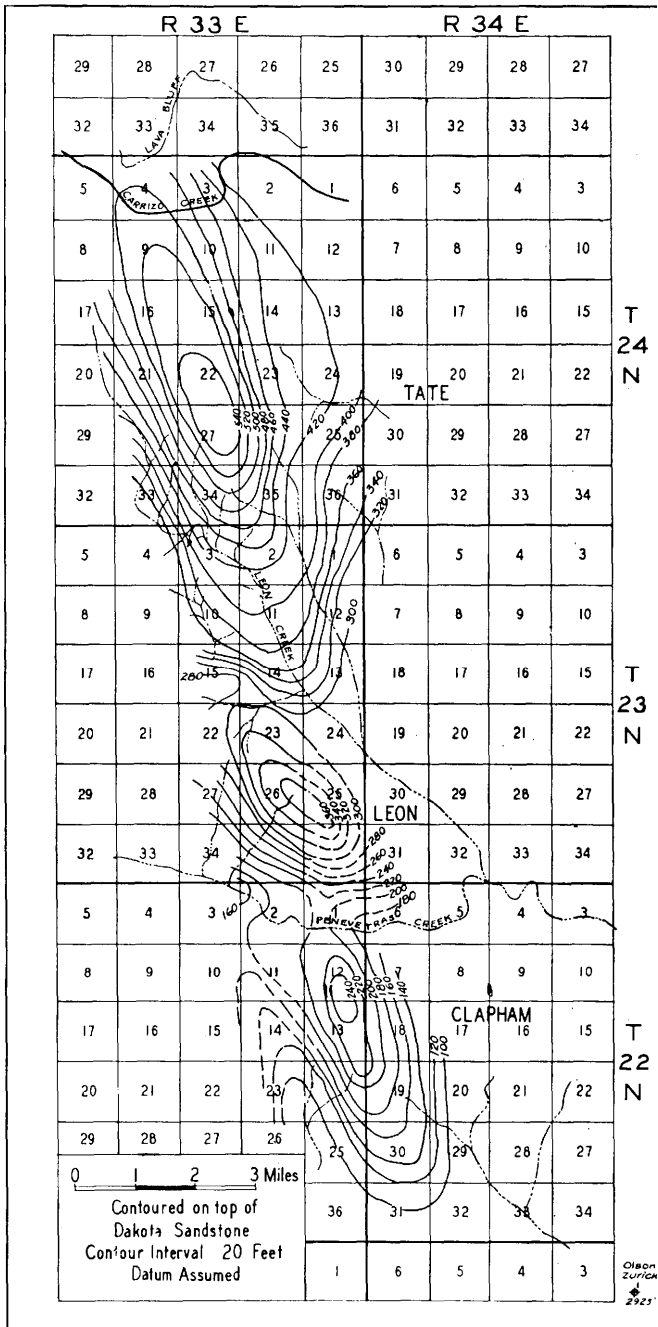
FIGURE 9.—Structure map of the Tate, Leon, and Clapham anticlines. Union County.
