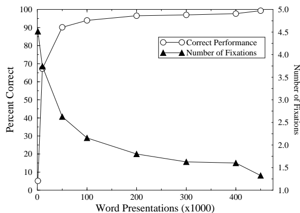
Figure 5. Percentage of words pronounced correctly by the network (top curve; left axis) and the mean number of fixations required (bottom curve, right axis) as a function of the number of words presented during training. The improvement in performance from 400,000 to 450,000 is due to a reduction in learning rate (see text).
