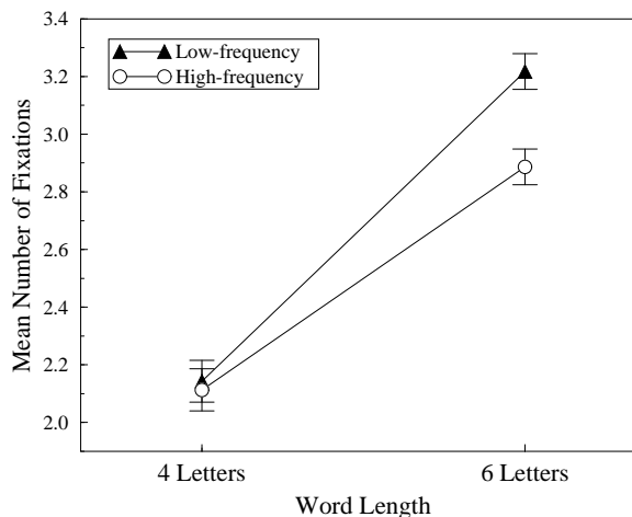
Figure 9. Mean number of fixations made by the model in pronouncing 4- and 6-letter words as a function of their frequency.
