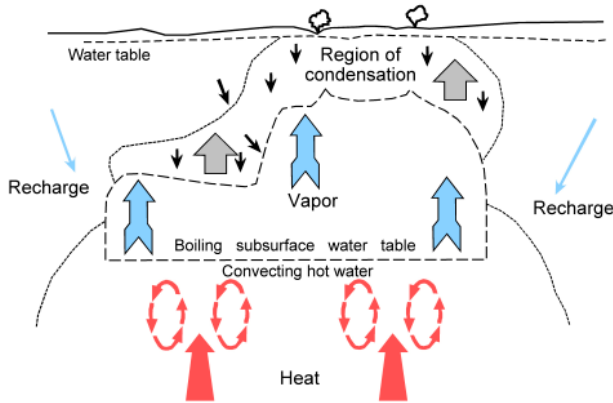
Figure 1. Vapor dominated geothermal system. (White, et al., 1971)
