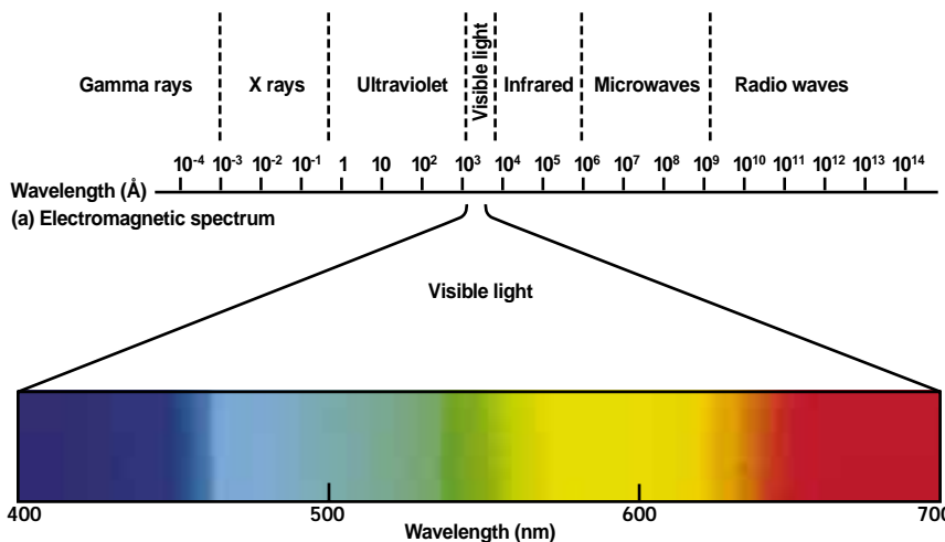
(b) Visible spectrum
