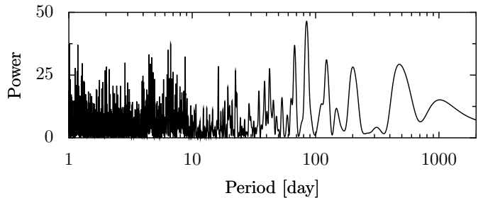
Fig. 2. Periodogram of the radial-velocity residuals around the 2-planet Keplerian model for Gl 581. Some power is visible at P = 84 d.
