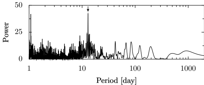
Fig. 1. Lomb-Scargle periodogram of the radial-velocity residuals around the 1-planet solution, clearly showing a peak close to 13 days. (Power in arbitrary units, normalized by the velocity dispersion.)
