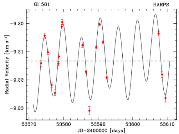
Fig. 4. Temporal display of the 3-planet Keplerian model of Gl 581, on a short time interval with dense observational sampling.
