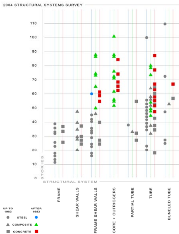
Figure 1. Survey of Structural Systems in Tall Buildings
