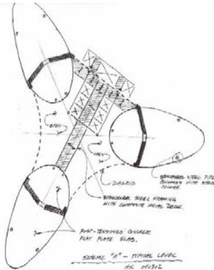
Figure 5. Plan (Halvorson and Partners, 2004)
