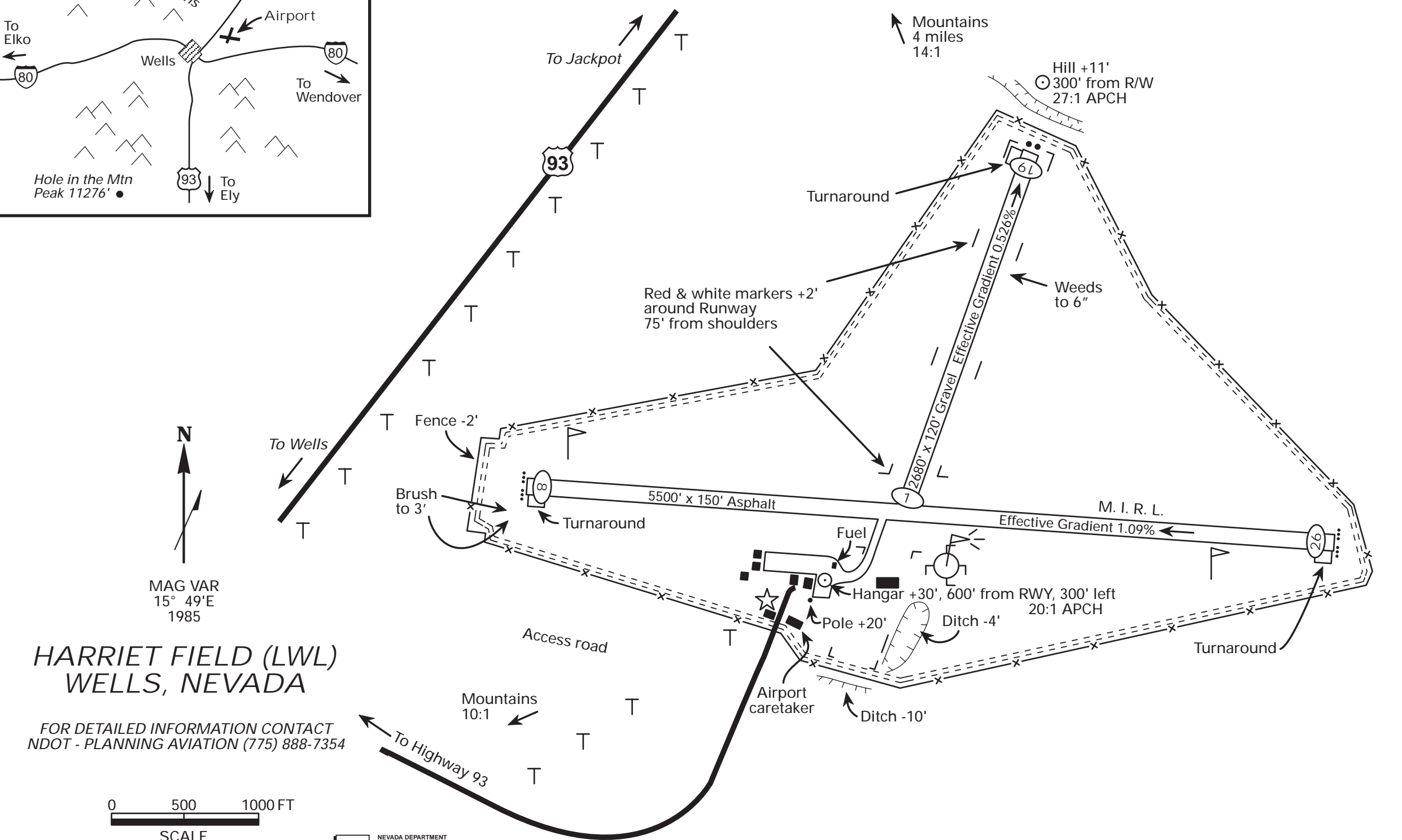
AIRPORT LAYOUT
