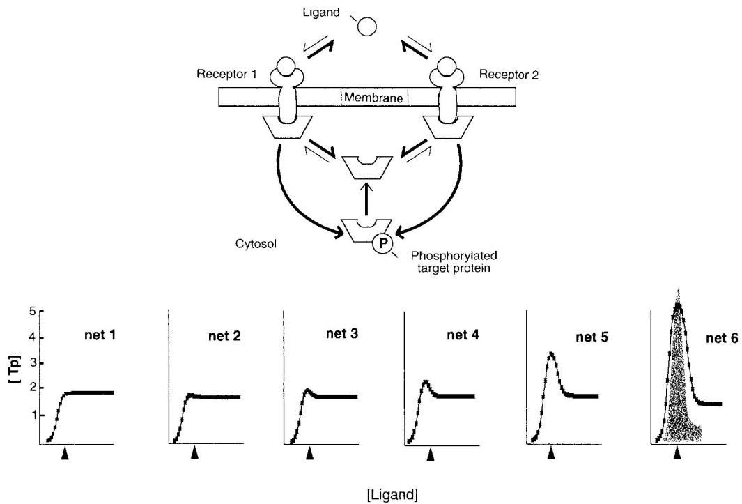
FIG. 3 Training a protein circuit by simulated evolution 25 . a , Model circuit built from two membrane receptors and an intracellular target protein. The two receptors, initially identical, have a binding site for the same extracellular ligand. When complexed with the ligand, the receptors bind to the target protein in the cytoplasm and phosphorylate it. The performance of the circuit, modelled by computer simulation, is specified by the seven rate constants shown as bold arrows. b , Optimization of the protein circuit to produce a specified input/output relationship. The circuit shown in a was assigned starting values of rate constants and the amount of phosphorylated target protein (output) measured for a range of ligand concentrations. This gave the dose-response curve net 1. Random changes in the rate constants were then made after which the response of the new circuit was again tested over a range of ligand concentrations. If the new circuit gave a dose-
