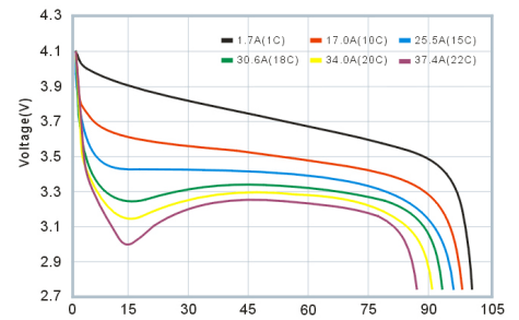
Discharge Capacity(%)
