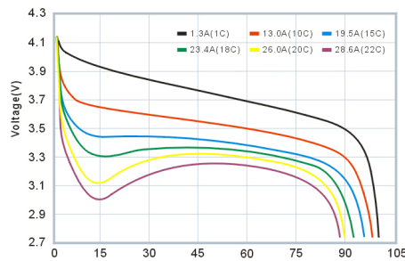
Discharge Capacity(%)
