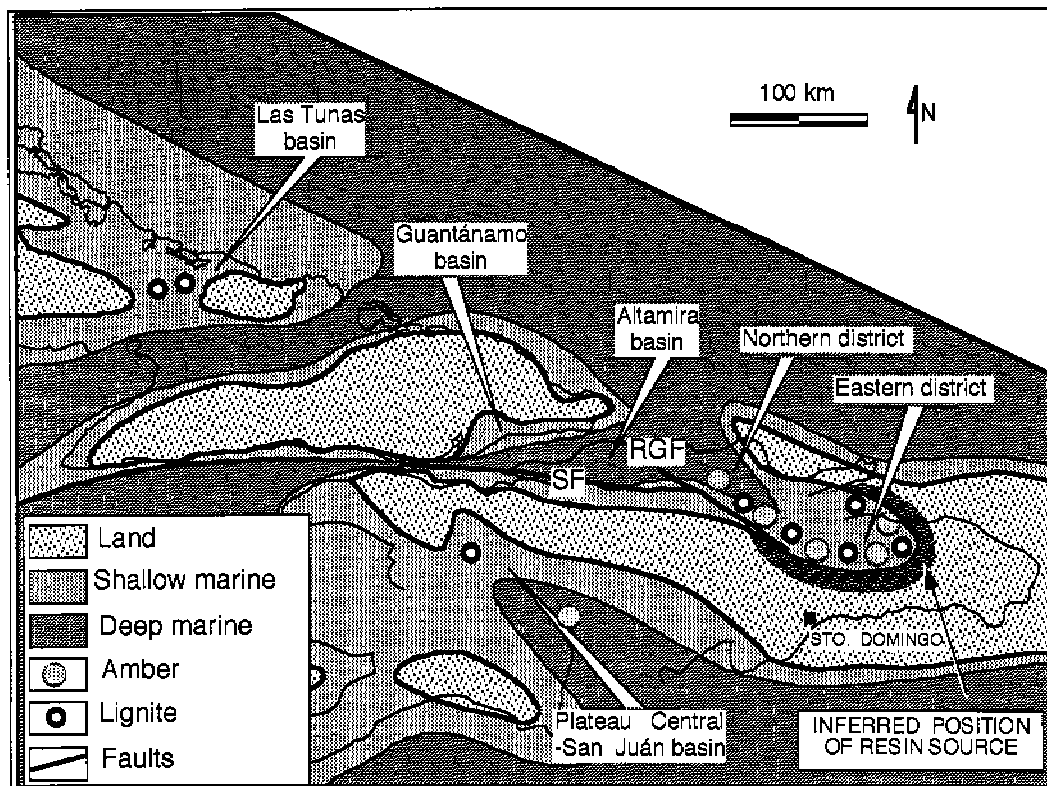
FIG. 9. Paleogeographic map of eastern Hispaniola during the deposition of copal in the Comatillo basin (marine embayment embracing the northern and eastern mining districts restored to their Miocene -16-14 m.y.-paleogeographic position). SF Septentrional fault, RGF Río Grande fault. Modified from Iturralde-Vinent and MacPhee, 1996.
