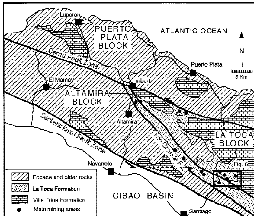
FIG. 5. Simplified geologic map of the northern mining district of the Dominican Republic. Adapted from several sources.
