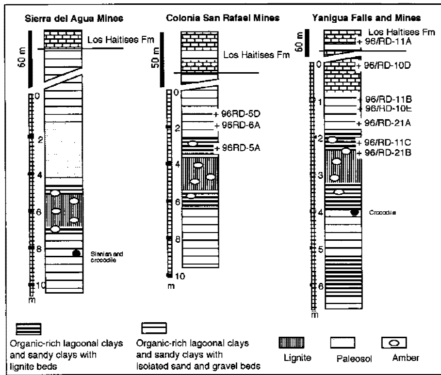
FIG. 4. Selected lithologic sections of the Yanigua Formation.
