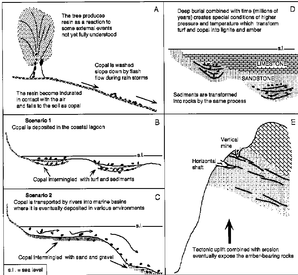
FIG. 10. Formation of the amber/lignitic deposits in the Comatillo basin, Dominican Republic.
