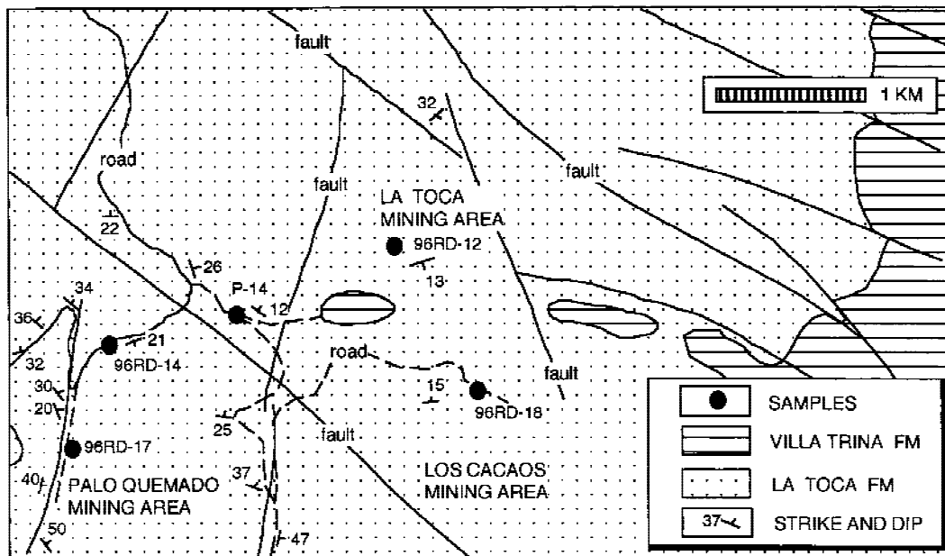
FIG. 6. Detailed geologic map of the La Toca, Palo Quemado, and Los Cacaos mining areas. Location in figure 5. Modified from de Zoeten (1988).
