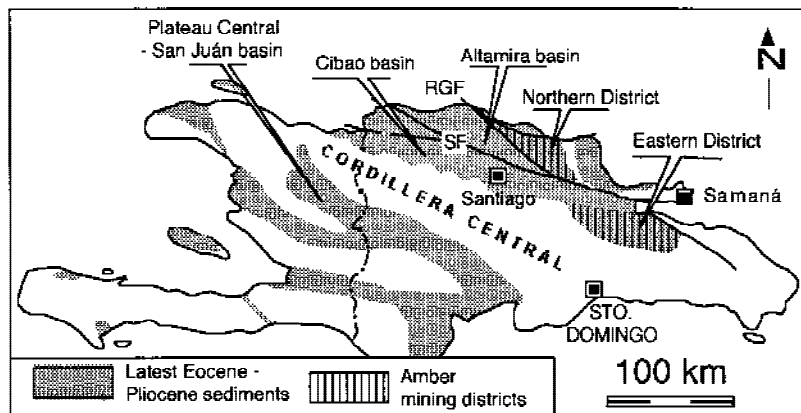
FIG. 2. Generalized geological map of Hispaniola showing the amber-bearing areas. Adapted from Iturralde-Vinent and MacPhee, 1996.
