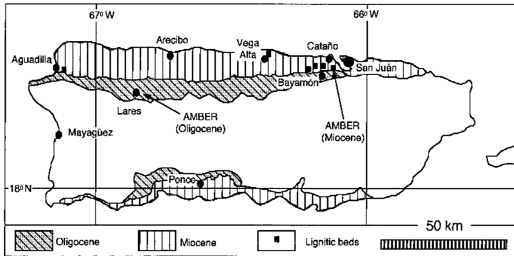
FIG. 7. Generalized geologic map of Puerto Rico showing lignitic and amber occurrences. Updated from Iturralde-Vinent and Hartstein, 1998.
