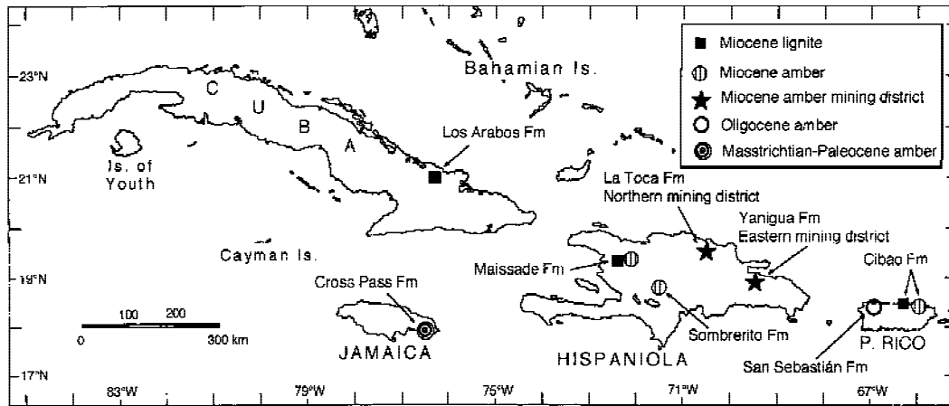
FIG. 1. Amber and lignite occurrences in the Greater Antilles. Lignite is not always associated with amber, but the opposite is true.
