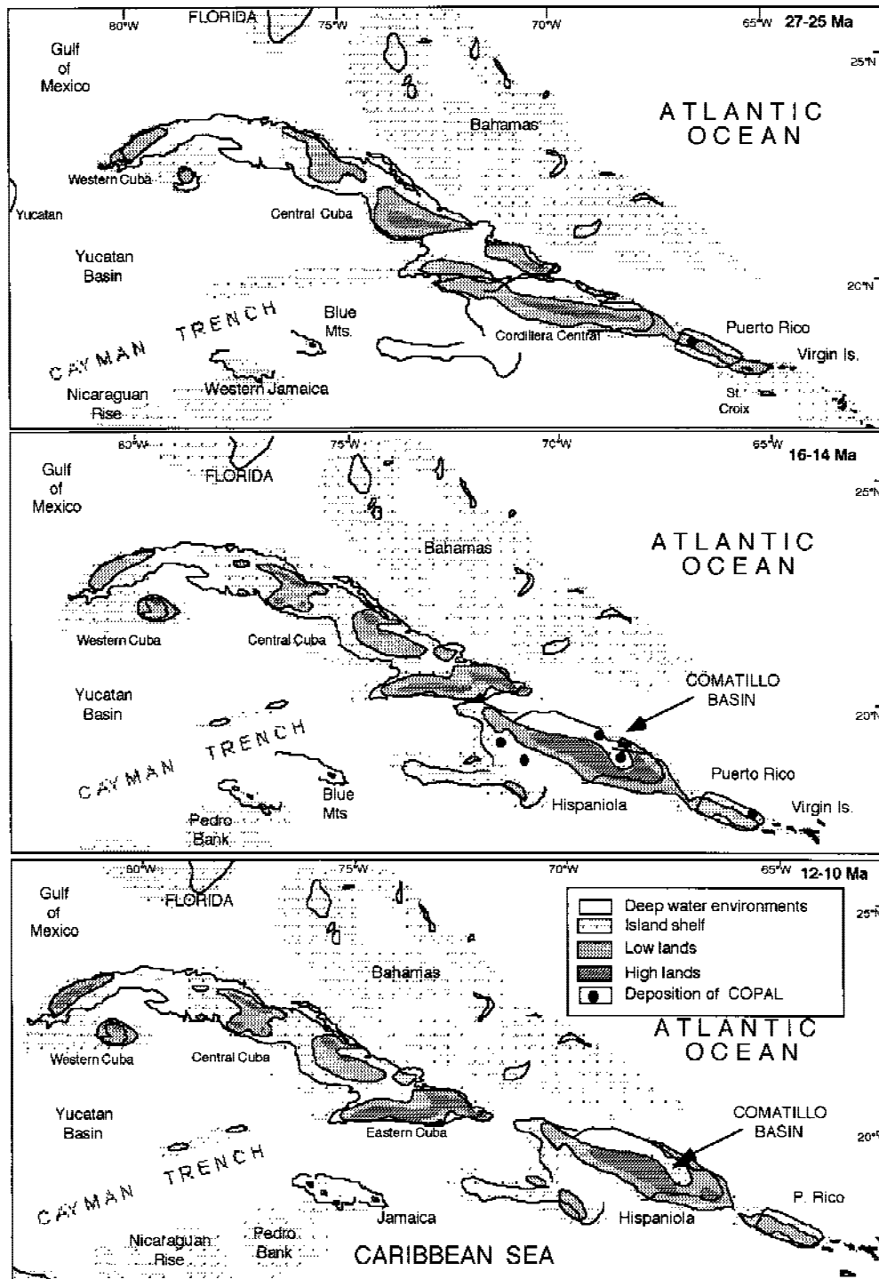
FIG. 8. Paleogeographic maps of the Greater Antilles for the Late Oligocene (27-25 m.y.), Lower Miocene (16-14 m.y.) and Middle Miocene (12-10 m.y.). Updated from Iturralde-Vinent and MacPhee (1999) including a new map.
