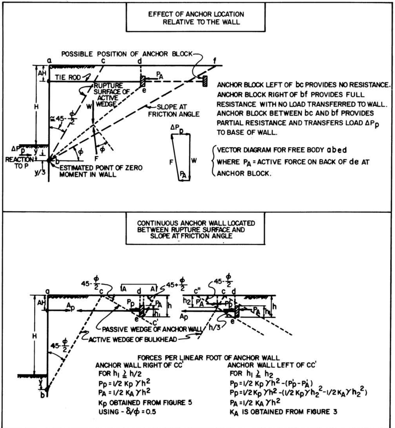
FIGURE 20 Design Criteria for Deadman Anchorage
