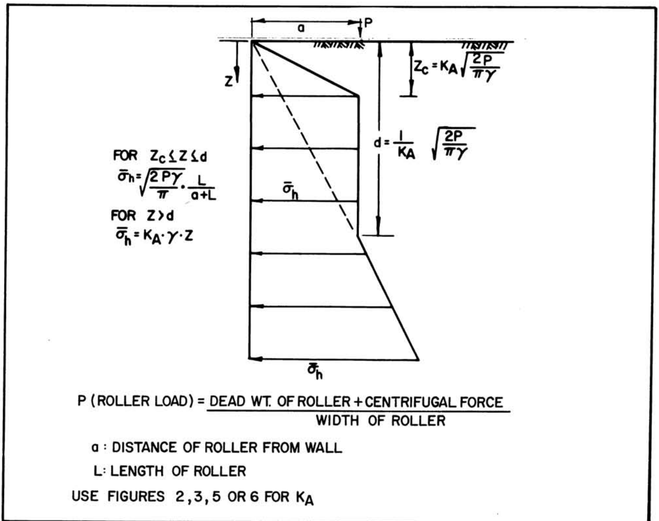
FIGURE 13 Horizontal Pressure on Walls from Compaction Effort
