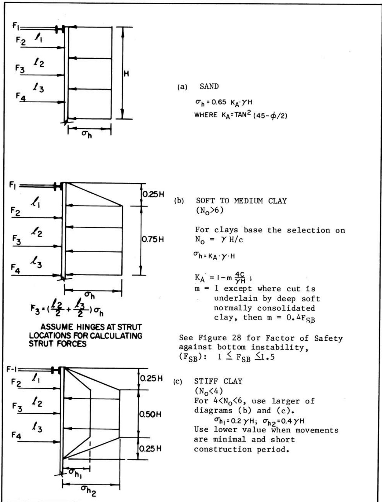
FIGURE 26 Pressure Distribution for Brace Loads in Internally Braced Flexible Walls
