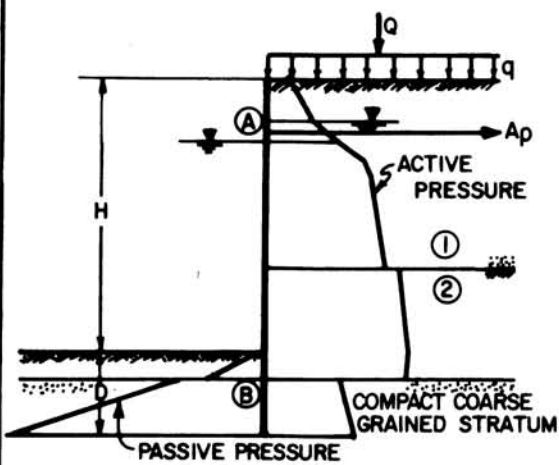
PENETRATION IN COMPACT COARSE GRAINED STRATUM
