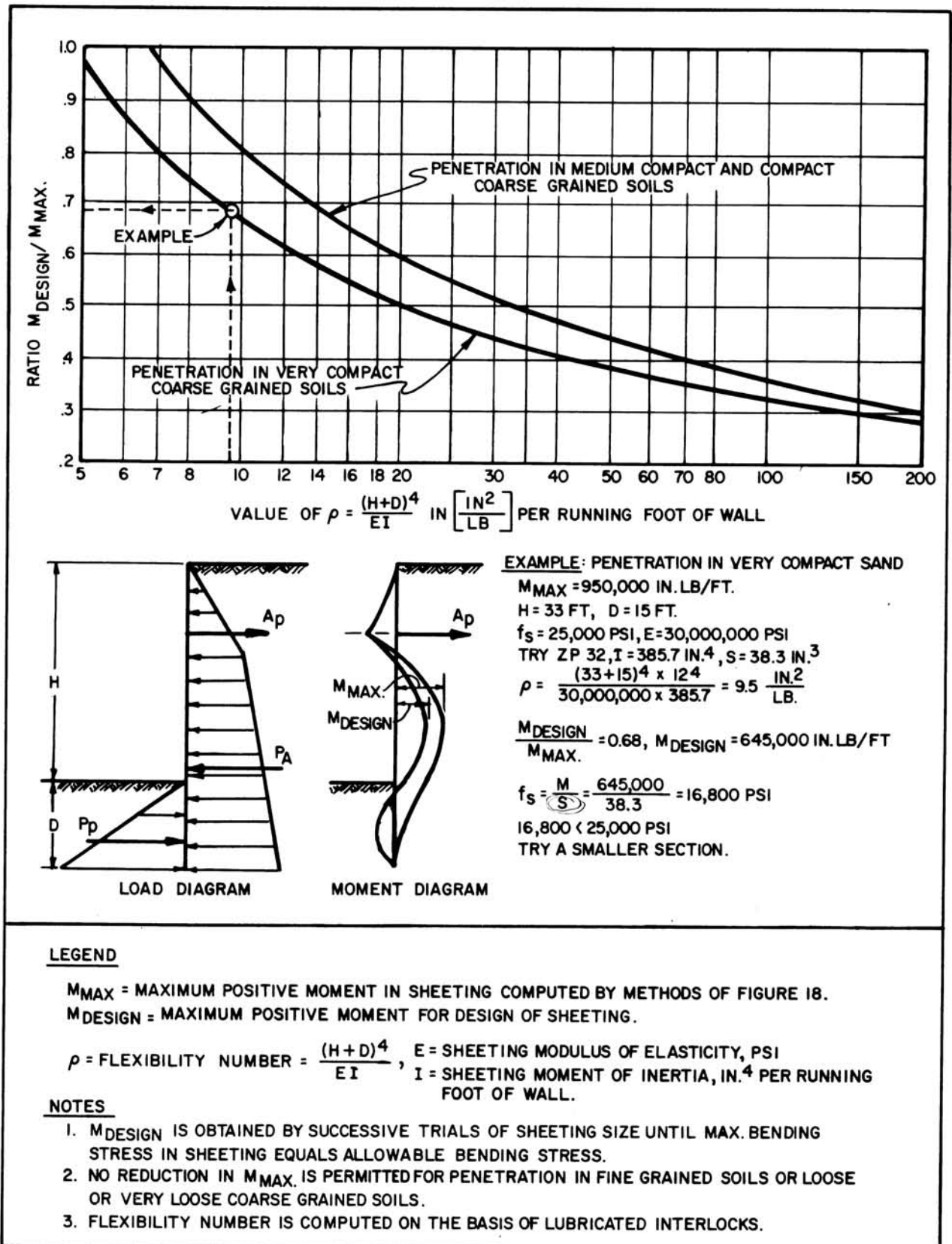
FIGURE 19 Reduction in Bending Moments in Anchored Bulkhead from Wall Flexibility
