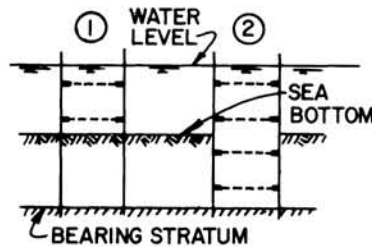
COFFERDAM EXCAVATED UNDER WATER
