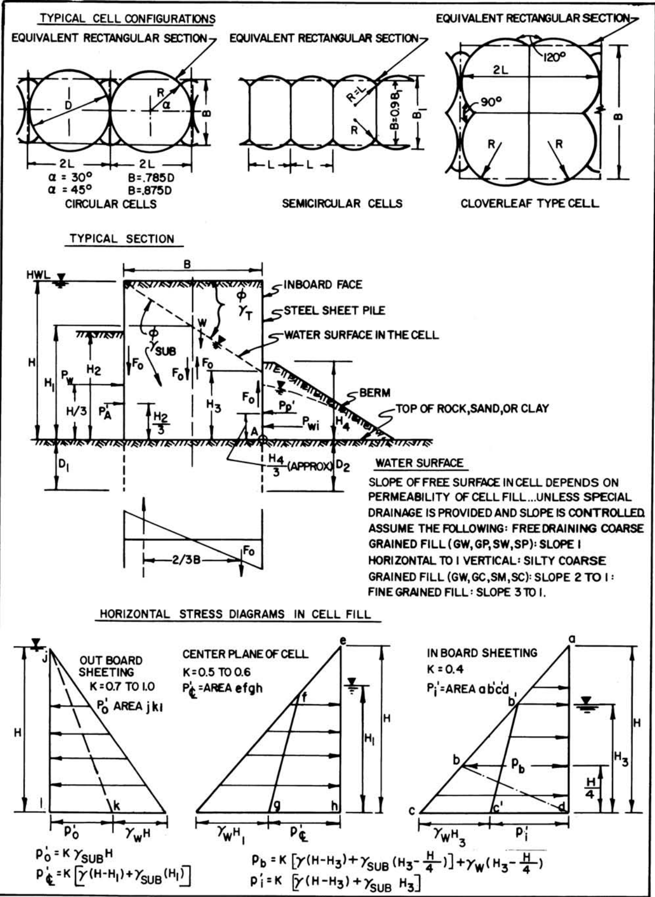
FIGURE 37 Design Criteria for Cellular Cofferdams 7.2-119
