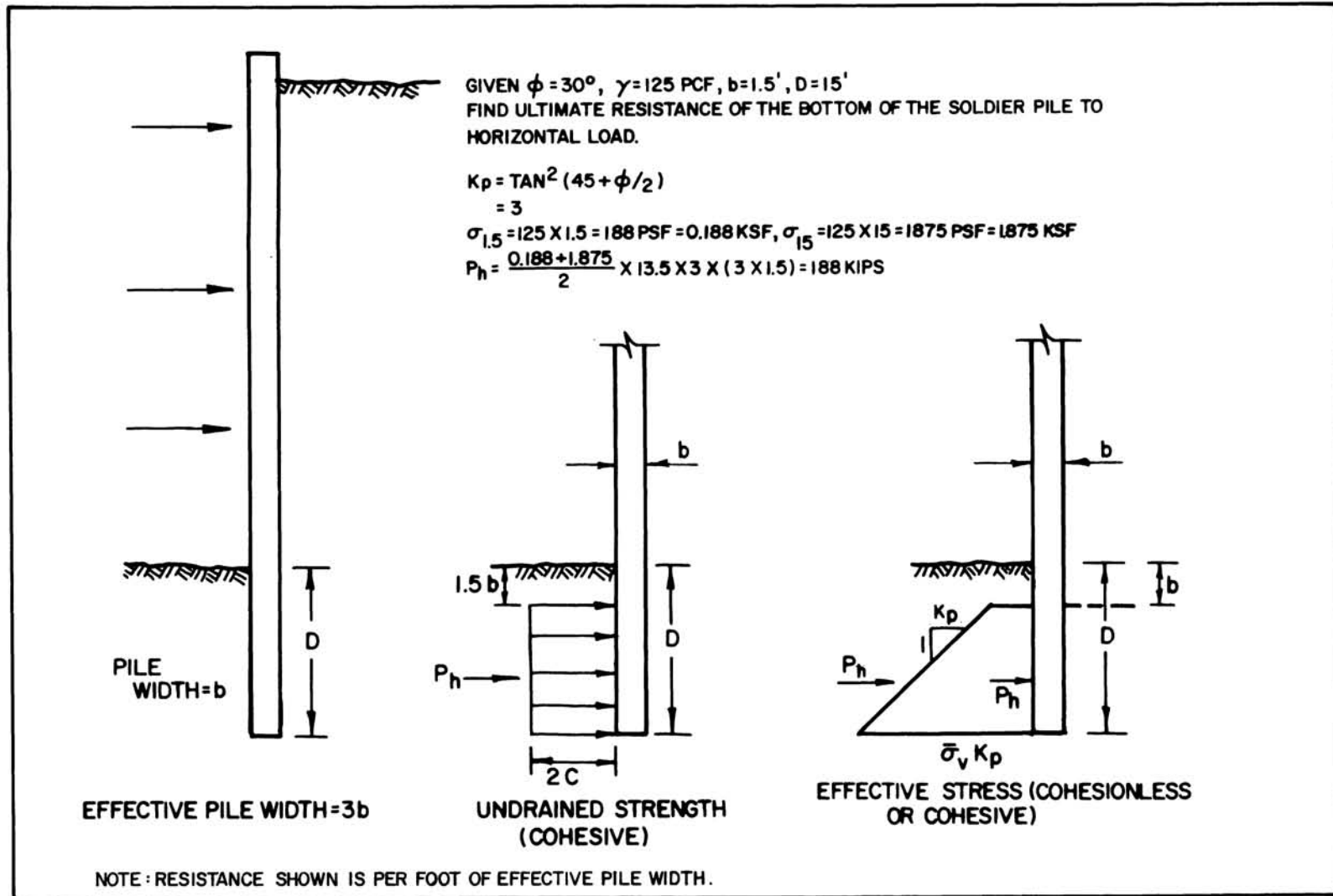
FIGURE 33 Passive Pressure Distribution for Soldier Piles
