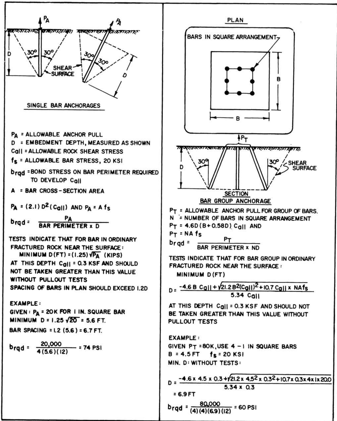
FIGURE 16 Capacity of Anchor Rods in Fractured Rock
