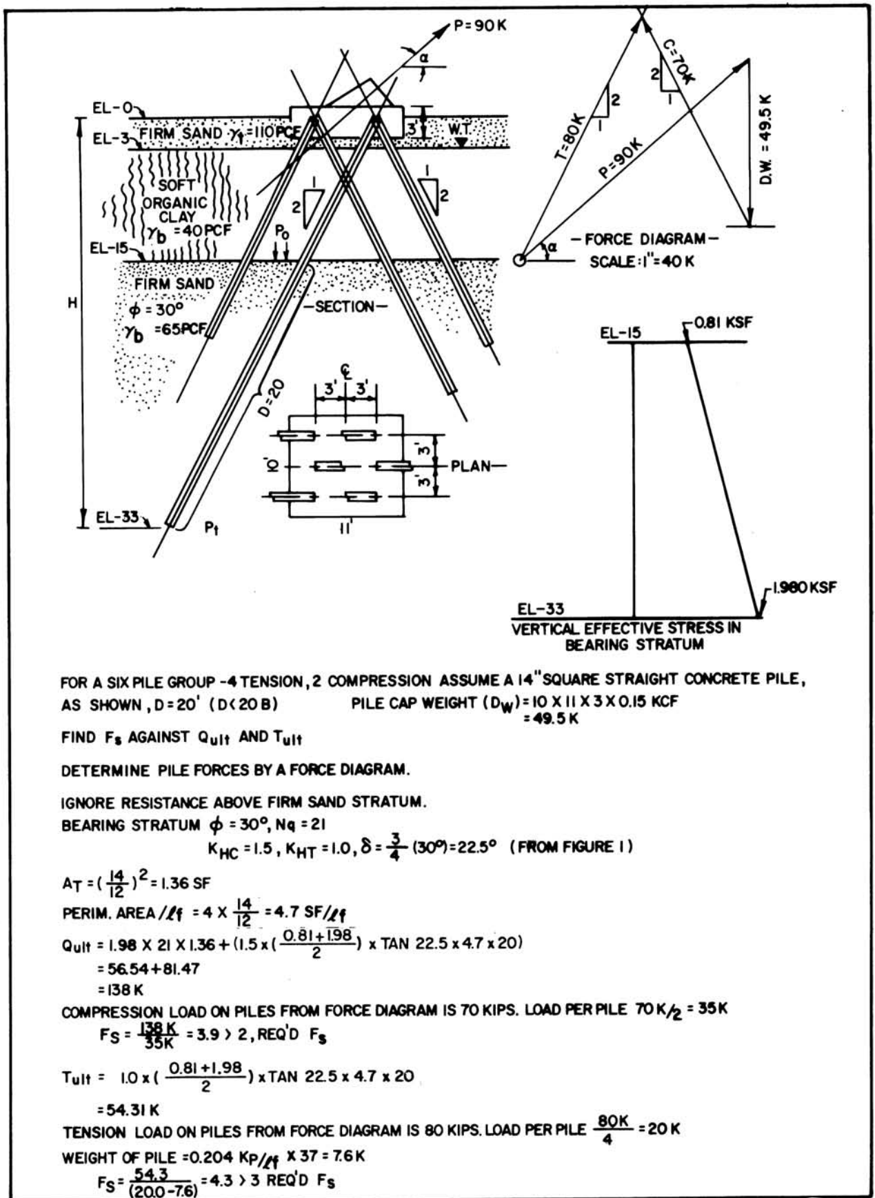
FIGURE 8 Example Problem - Batter Pile Group as Guy Anchorage 7.2-233
