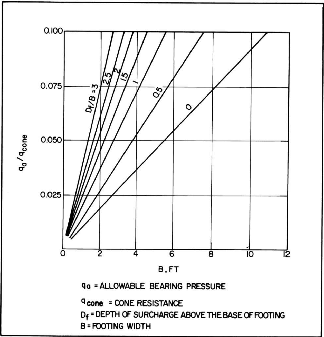
FIGURE 8 Allowable Bearing Pressure for Sand From Static Cone Penetration Tests
