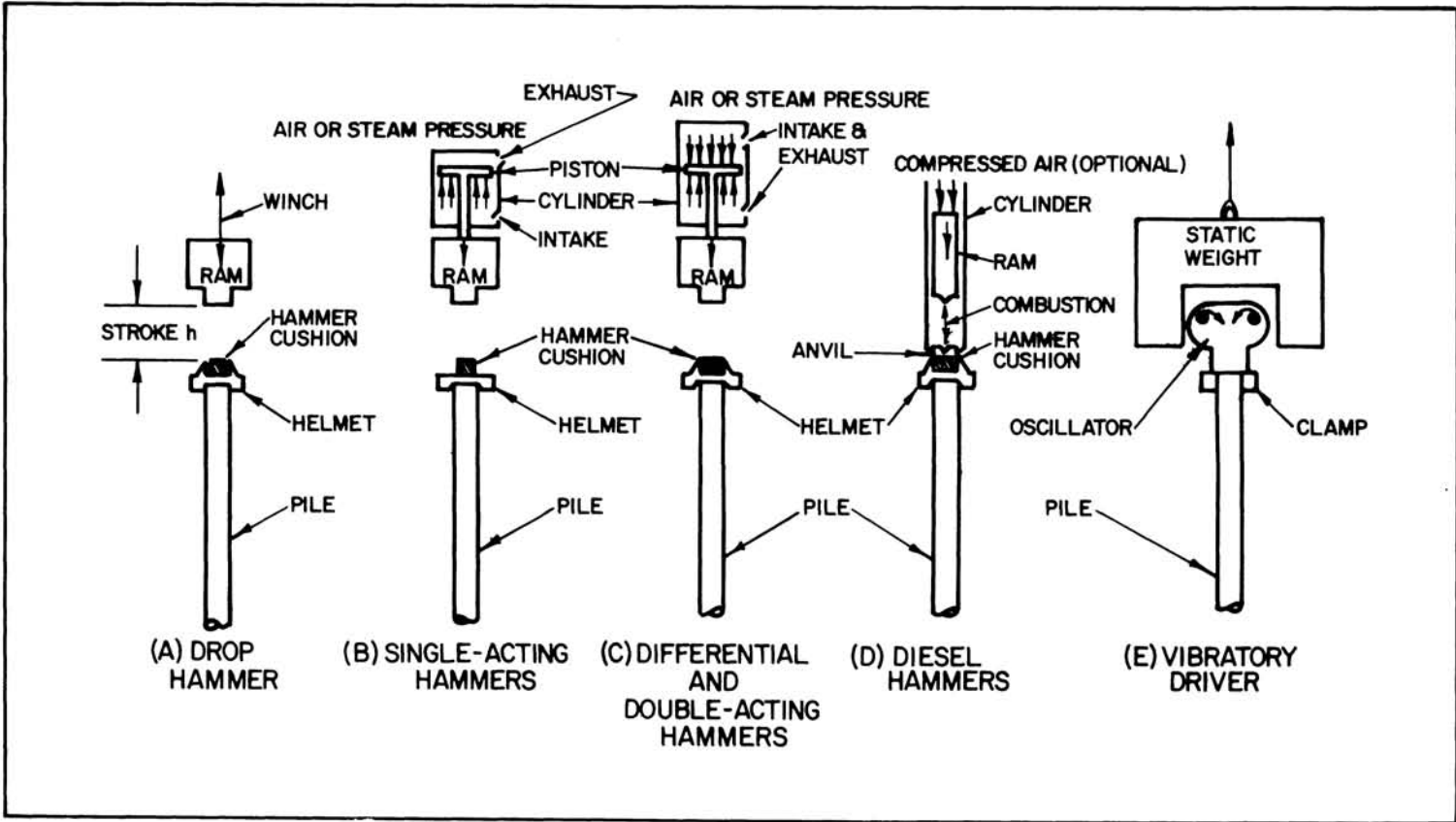
FIGURE 5 Principles of Operation of Pile Drivers
