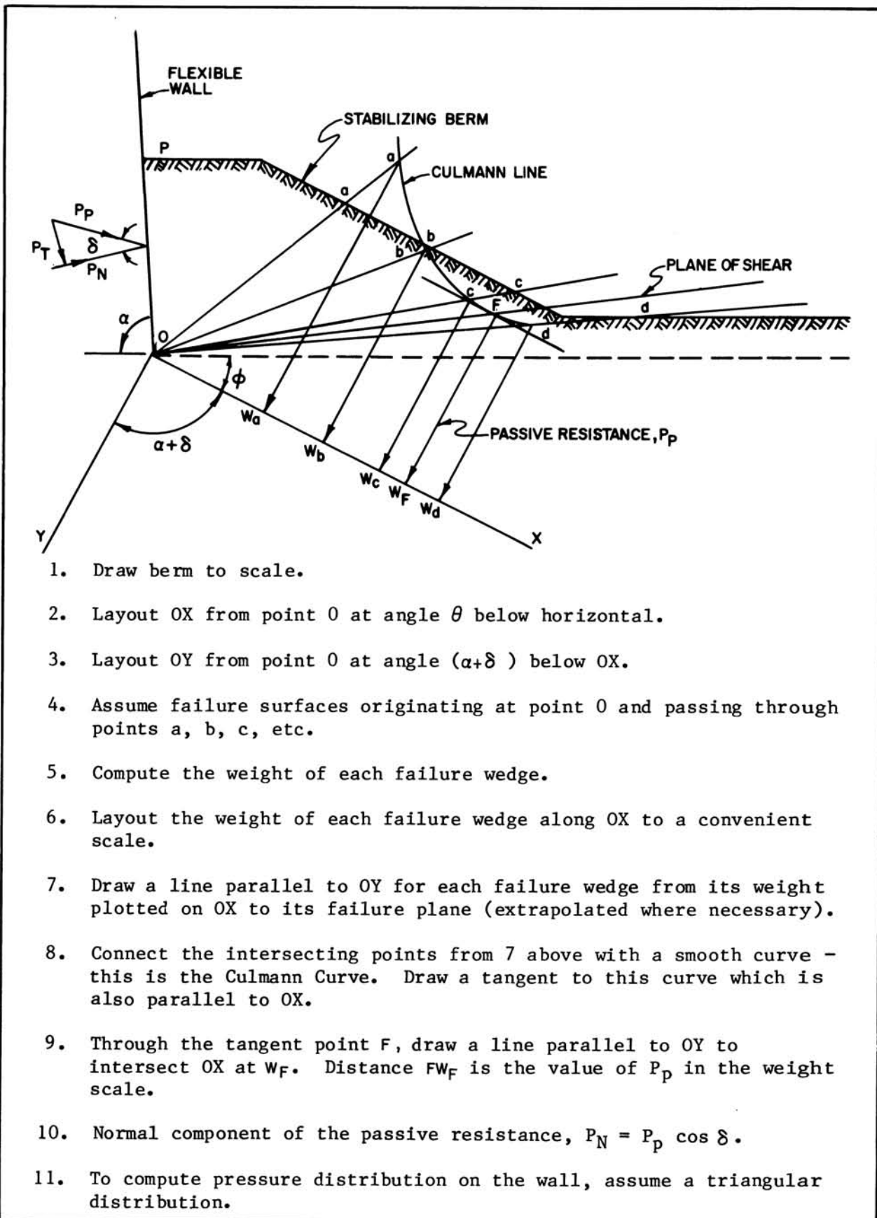
Figure 32 Culmann Method for Determining Passive Resistance of Earth Berm (Granular Soil) 7.2-113
