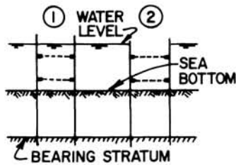
COFFERDAM EXCAVATED IN DRY
