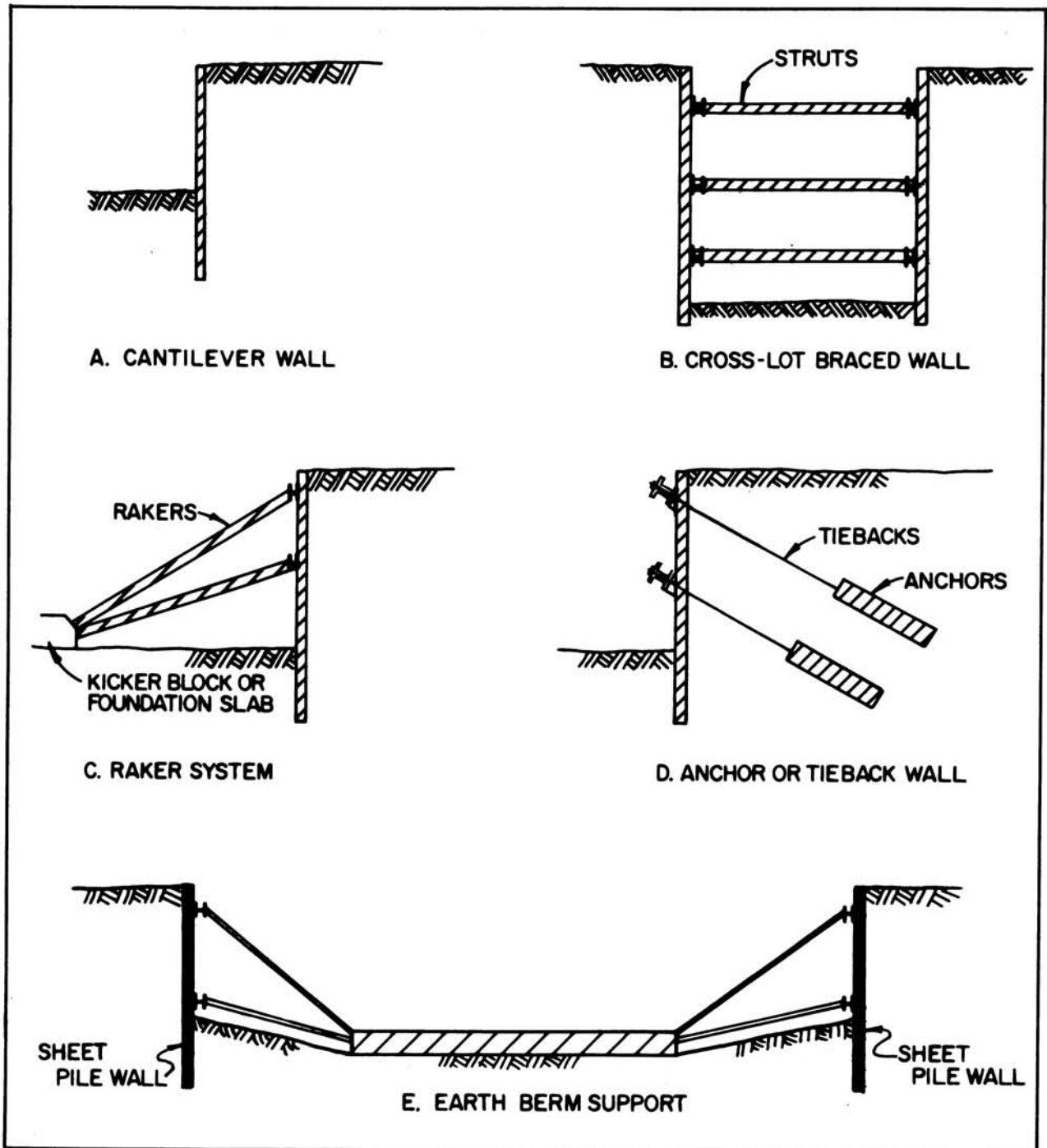
FIGURE 6 Support System - Walled Excavation
