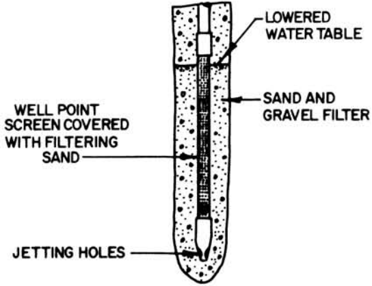
(C) DETAILS OF WELLPPOINT SYSTEM
