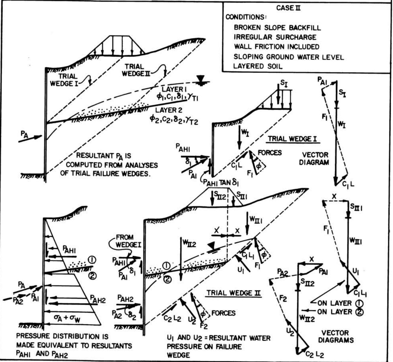
FIGURE 7 Computation of General Active Pressures 7.2-68
