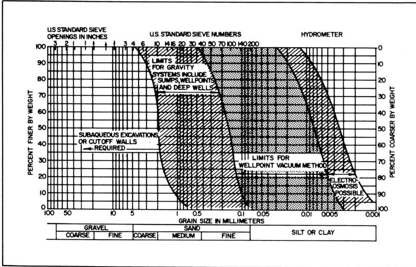
FIGURE 14 Limits of Dewatering Methods Applicable to Different Soils
