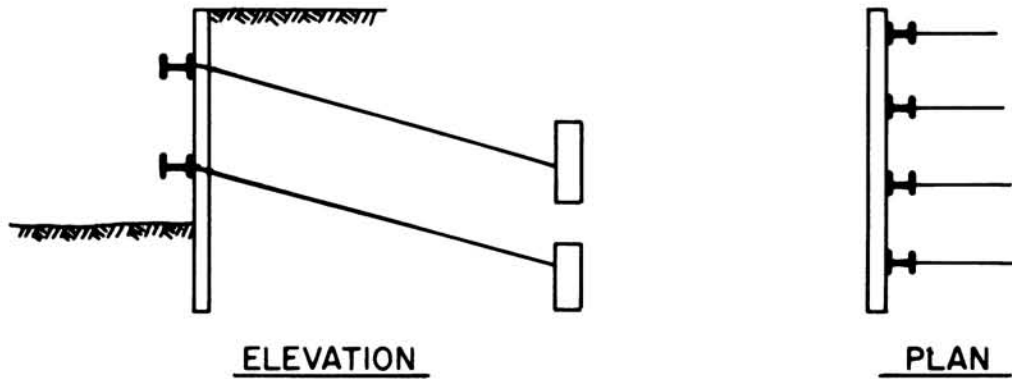
FIGURE 29 Pressure Distribution for Tied-Back Walls
