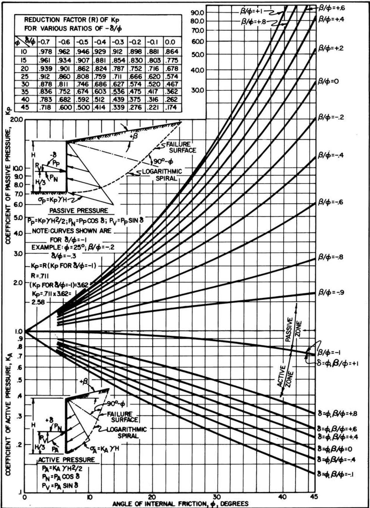
FIGURE 6 Active and Passive Coefficients with Wall Friction (Sloping Backfill)
