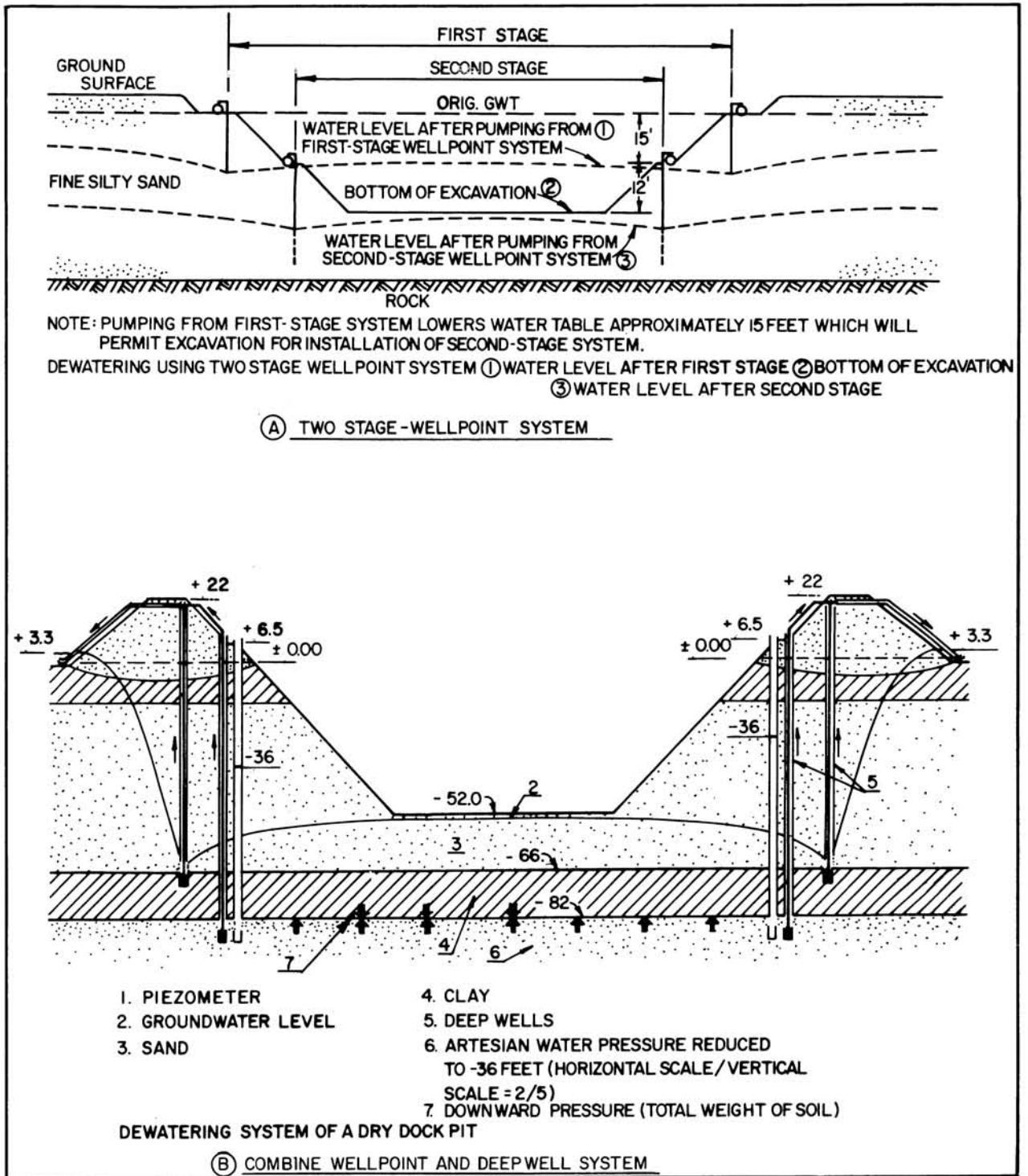
FIGURE 13 Methods of Construction Dewatering
