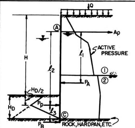
PENETRATION TO TOP OF HARD UNYIELDING STRATUM
