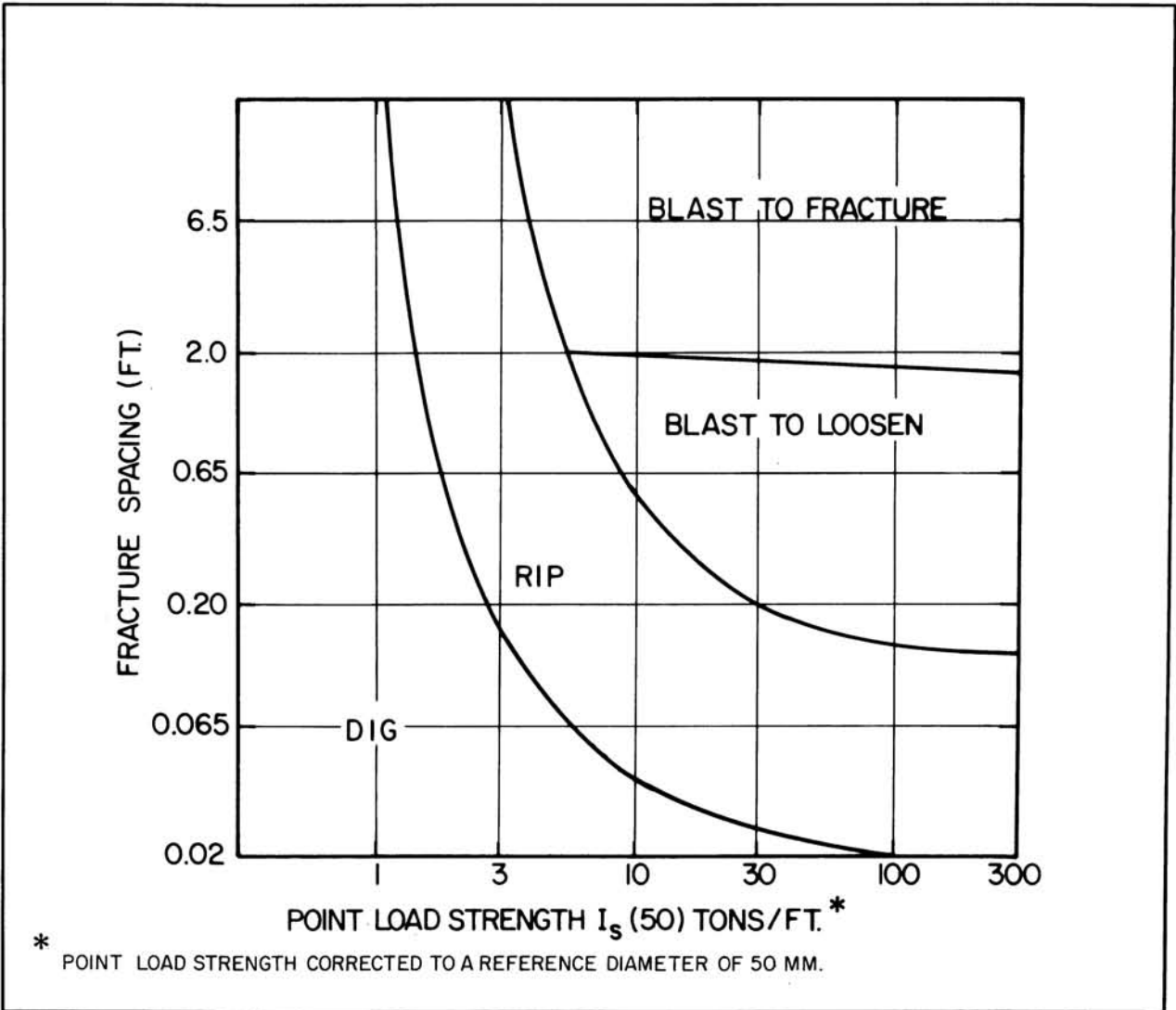
FIGURE 9 Suggested Guide for Ease of Excavation
