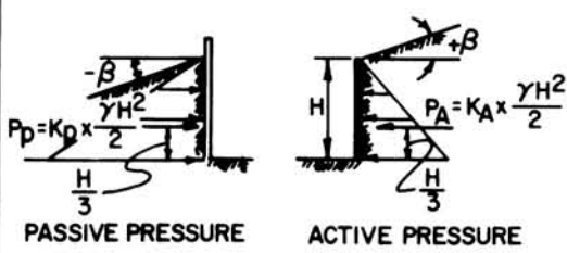
FIGURE 3 Active and Passive Coefficients, Sloping Backfill (Granular Soils)
