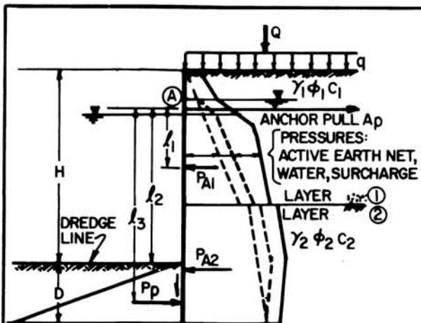
FREE EARTH SUPPORT - GENERAL CASE
