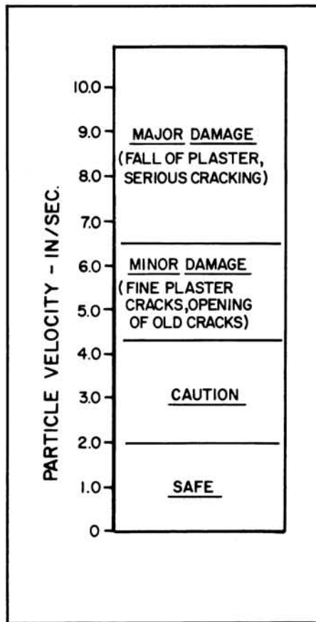
FIGURE 11 Guideline for Assessing Potential for Damage Induced by Blasting Vibration to Residential Structure Founded on Dense Soil or Rock
