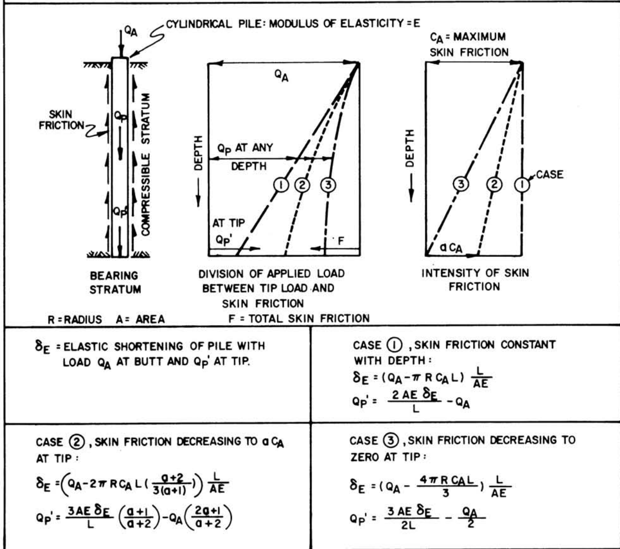
FIGURE 7 Load Test Analysis Where Downdrag Acts on Pile
