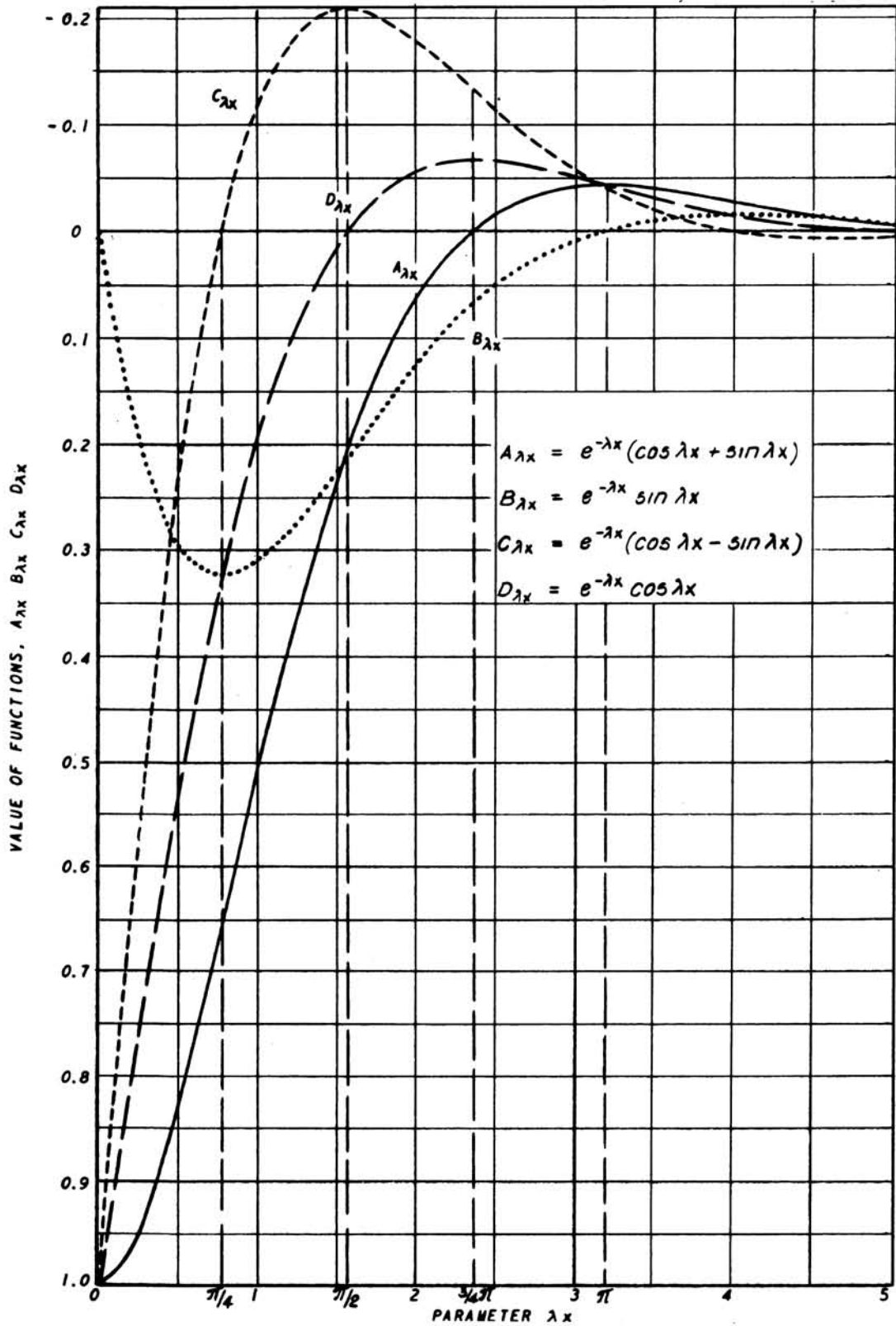
FIGURE 11 Functions for Shear, Moment, and Deflection, Beams on Elastic Foundations
