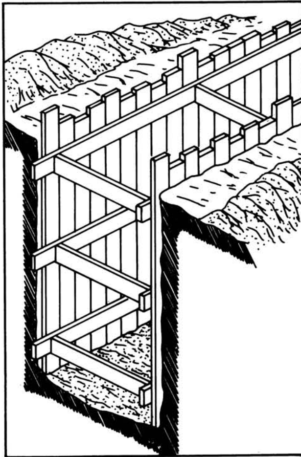
Requirements for Close Sheetting
