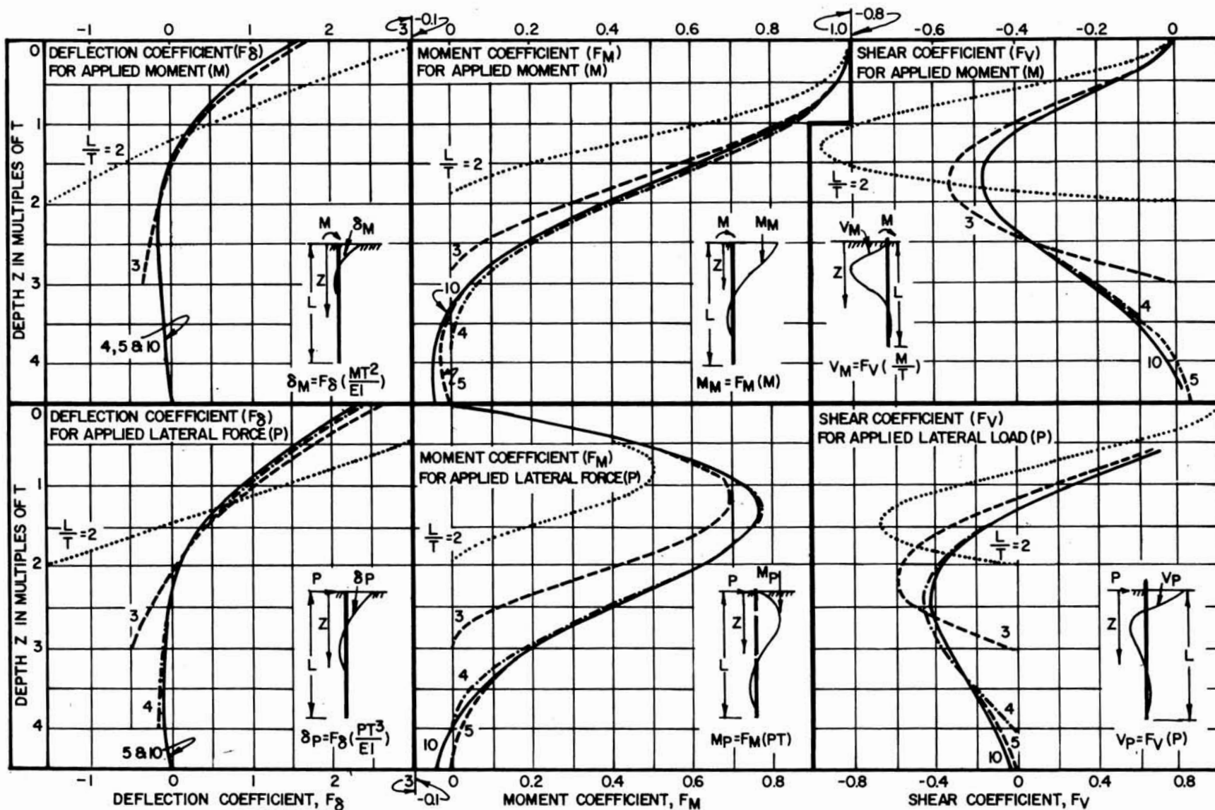
FIGURE 11 Influence Values for Pile with Applied Lateral Load and Moment (Case I. Flexible Cap or Hinged End Condition)
