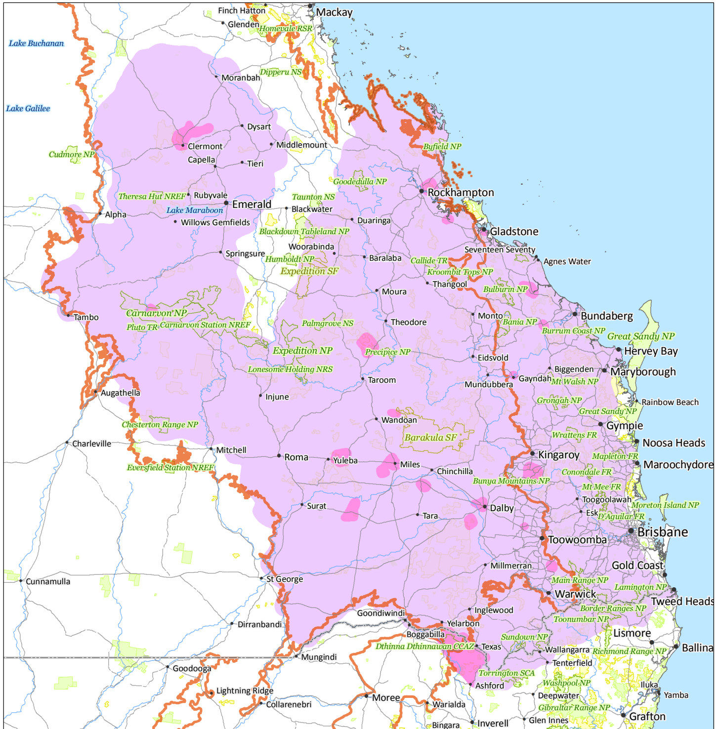
Map 10: The modelled distribution of Dunmall's snake ( Furina dunmali )
