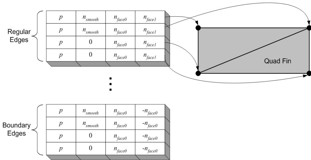
Figure 2 – Vertex buffer organization for silhouette edge rendering
