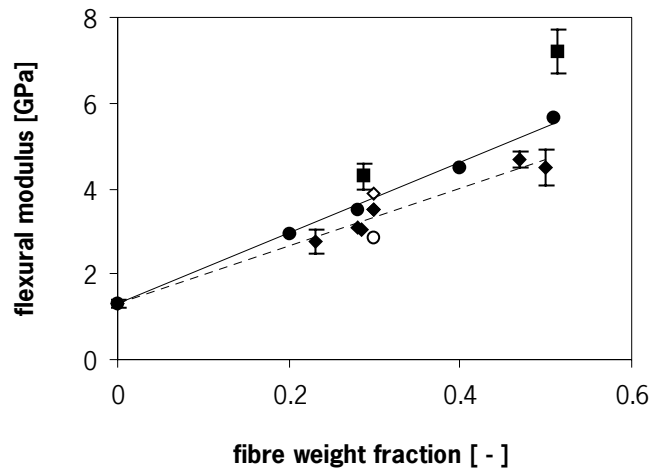
Figure 6.2. Flexural modulus of ● kneaded flax/PP/MAPP and ○ kneaded flax/PP, and ◆ extruded flax/PP/MAPP and ◇ extruded flax/PP compounds, compared with ■ hackled flax/PP/MAPP NMTs, versus fibre weight fraction. The fitted lines are: ——— kneaded and - - - - - extruded flax/PP/MAPP. Error bars smaller than the marker size are not shown.
