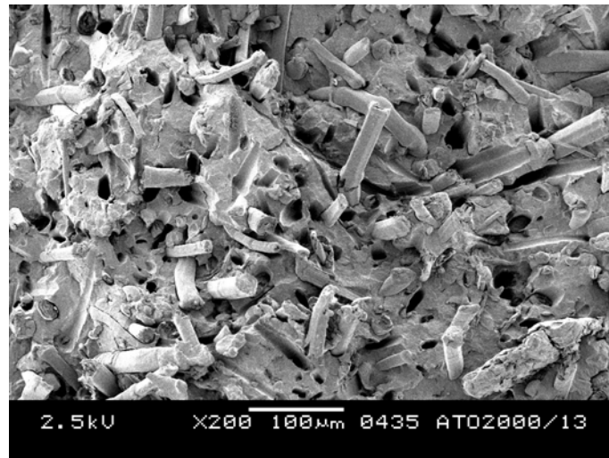
Figure 6.10. SEM micrograph of an uncompatibilised extrusion compound of 30 wt% flax/PP. Note the many deep holes where fibres have been pulled out.
