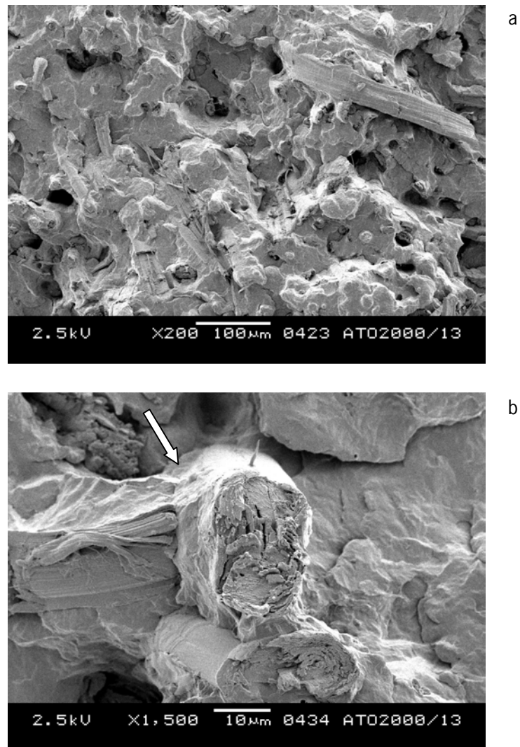
Figure 6.11. SEM micrograph of 30 wt% flax/PP/MAPP extrusion compound. (a) Note the undep holes and the short fibre pull out length. (b) The matrix is adhered very well to the primary cell wall (arrow). Note also that the lumen is closed, due to the extrusion and/or injection moulding process.
