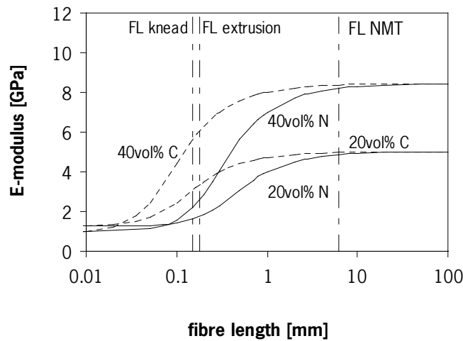
Figure 6.8. Young's modulus as a function of fibre length for 20 vol% and 40 vol% materials, following Cox-Krenchel, ——— NMTs (N), - - - - - compounds (C), - · - · - · - · - actual mean fibre length (FL) in the kneaded and extruded compounds and the NMTs. The E-modulus of both elementary and hackled fibres is taken as 50 GPa.
