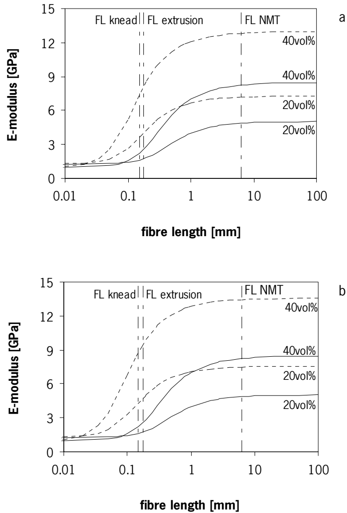
Figure 6.9. Young's modulus as a function of fibre length for 20 vol% and 40 vol% materials, following Cox-Krenchel, — NMTs, ---- compounds, - - - - - actual mean fibre length (FL) in the kneaded and extruded compounds and the NMTs. (a) The Young's modulus of the hackled fibres is taken as 50 GPa, of the elementary fibres as 80 GPa. (b) The orientation factor \eta_0 is taken as 0.375 for the NMTs and as 0.63 for the compounds.
