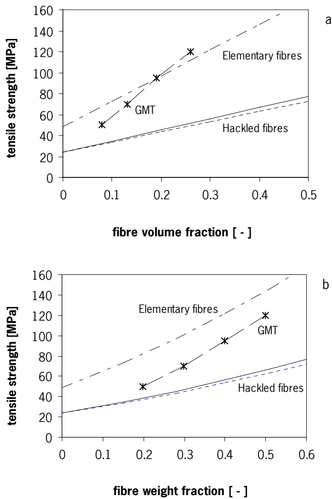
Figure 5.8. Kelly-Tyson predictions of the tensile strength of: ——— hackled flax/PP/MAPP, ······ hackled flax/PP, -·-·-· elementary flax fibre/PP/MAPP, compared with -*--*-- commercial GMT values [89], versus (a) fibre volume fraction and (b) fibre weight fraction.
