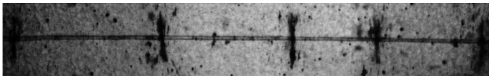
Figure A.2. Photograph of a fragmented elementary flax fibre in PP/MAPP; the fibre diameter is about 10 \mu\text{m} .
