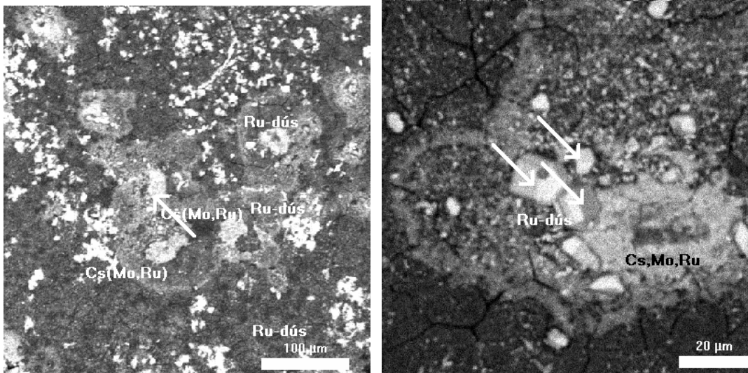
Figure 18: Deposits rich in Cs-Mo-Ru and in Ru, respectively on the surface of rod No. 4
