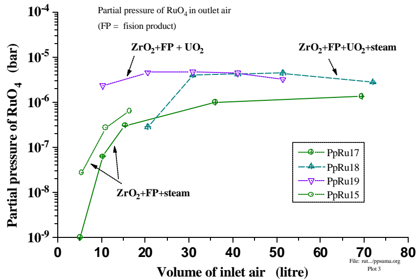
Figure 35. Partial pressure of \text{RuO}_4 in outflow air at experiments with charge \text{Ru} + \text{ZrO}_2 + \text{fission products} and also with \text{UO}_2 .
