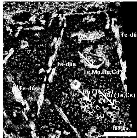
Figure 15: Deposits typical for rod No. 1 on BE image with 220 times of magnification
