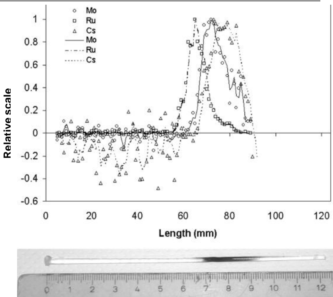
Figure 13. Deposits in quartz rod in case of FP-s in ZrO_2 matrix. (Sample Ru16-2, dry air, 1100°C, XRF capillary method)
