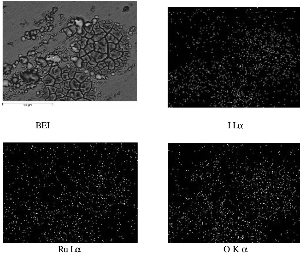
Figure 24: Digital BE image and the corresponding X-ray images of I, O and Ru for deposit with I content
