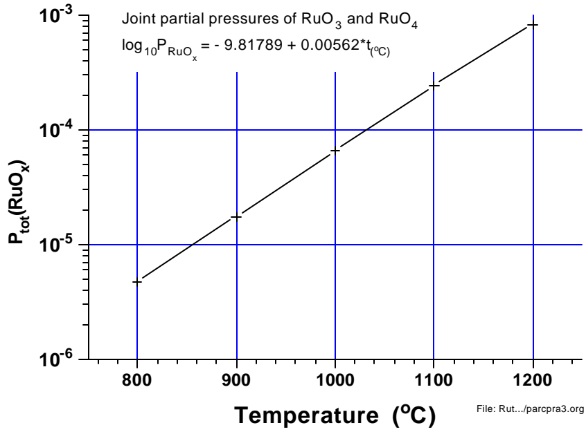
Figure 2. Joint partial pressure of RuO 3 and RuO 4 over RuO 2 at 1 bar air.
