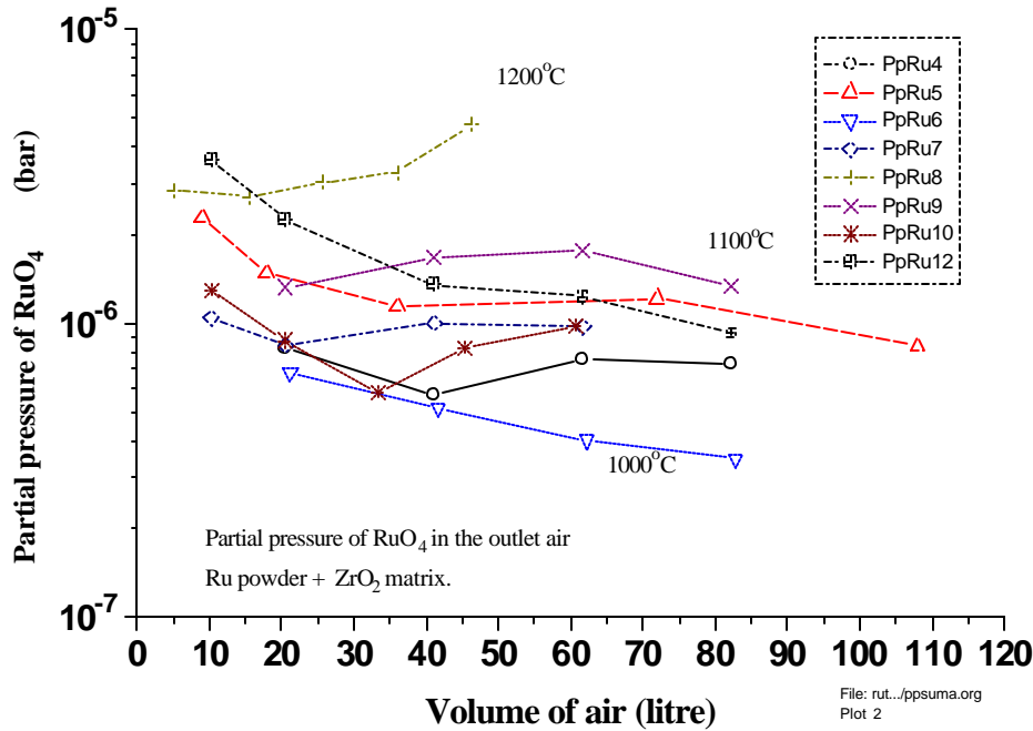
Figure 34. Partial pressure of RuO 4 in outflow air at Ru + ZrO 2 experiments
