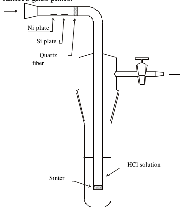
Figure 6. Scheme of sampling device
