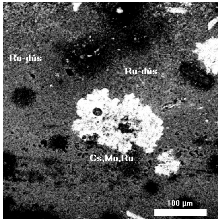
Figure 17: Deposits typical to rod No. 3
