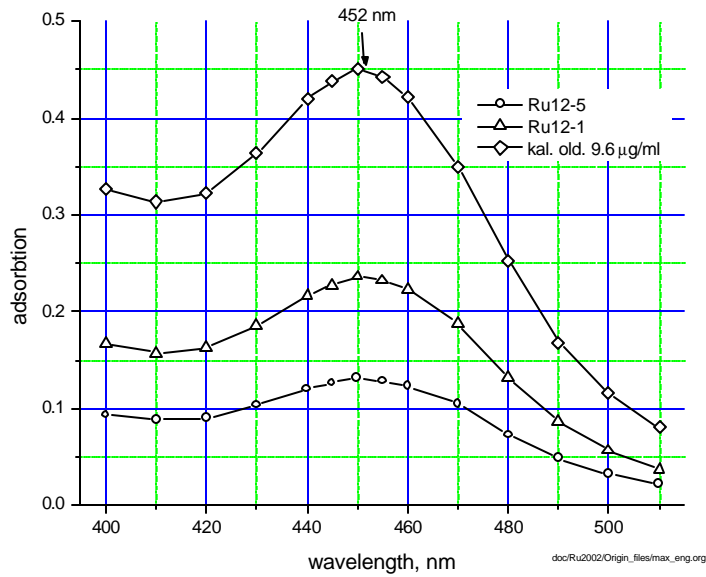
Figure 9. Light adsorption in function of wavelength of RuCl_3.nH_2O in 1 n HCl and absorber solutions from Ru12 test.
