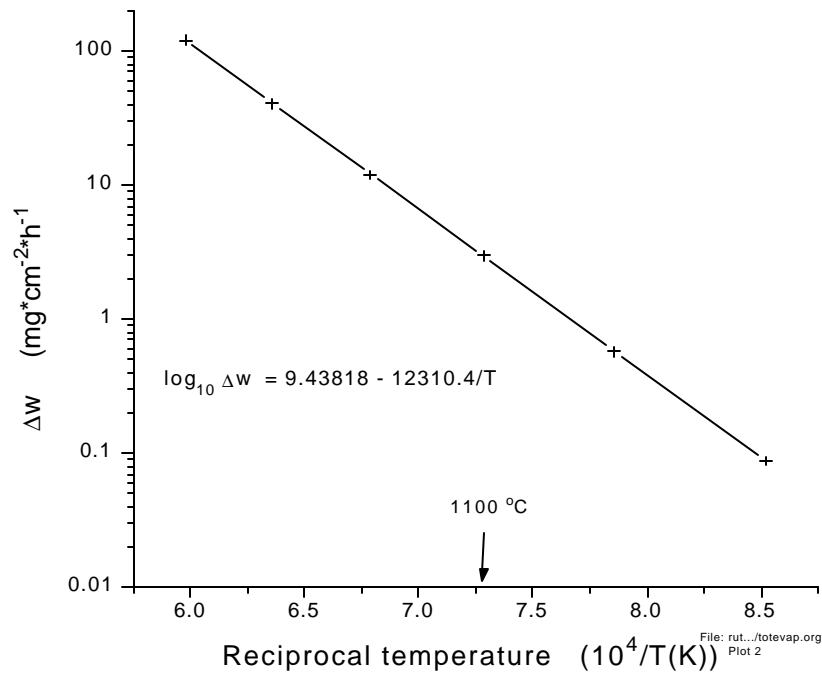
Figure 3. Evaporation rate of Ru in air (weight loss)
