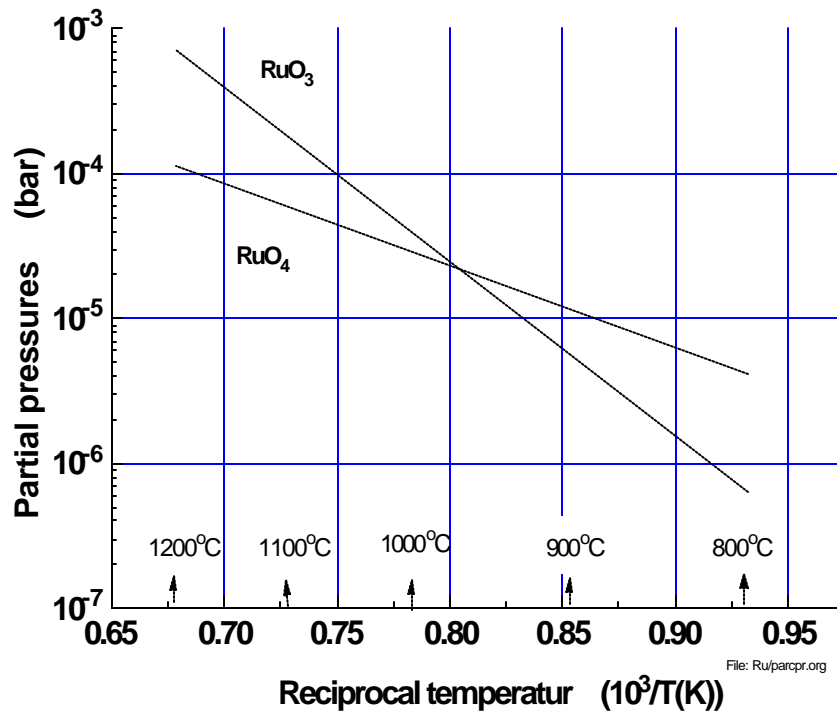
Figure 1. Partial pressures of \text{RuO}_3 and \text{RuO}_4 over \text{RuO}_2 in 1 bar air
