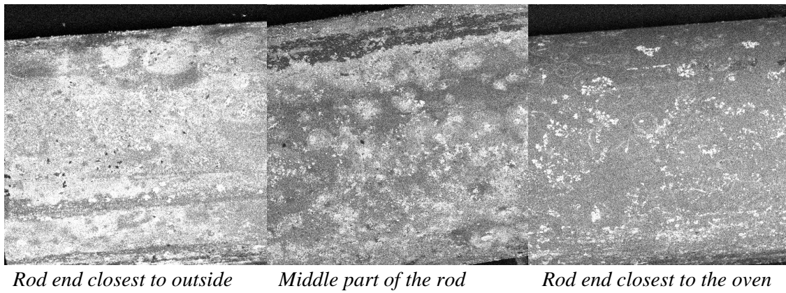
Figure 19: Small magnification image series of rod No. 5
