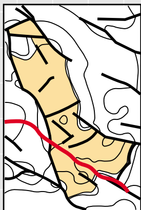
PEDL 048 - West Compton - 1 Well location and structural detail
