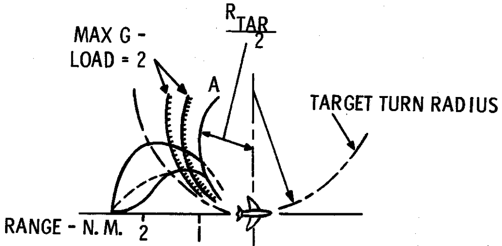
EFFECT OF SPEED RATIO ON CONDITIONS WHEN ATTACKING A MANEUVERING TARGET
