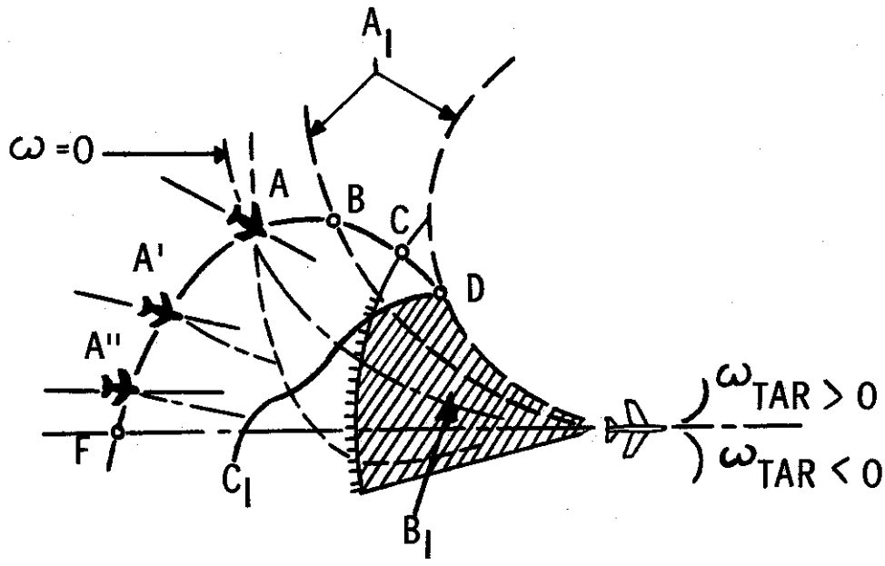
PURSUIT CURVES VS VARIOUS TARGET MANEUVERS
