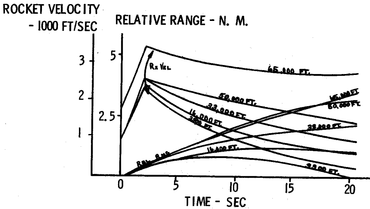
BALLISTIC CHARACTERISTICS OF R-3TYPE ROCKET
