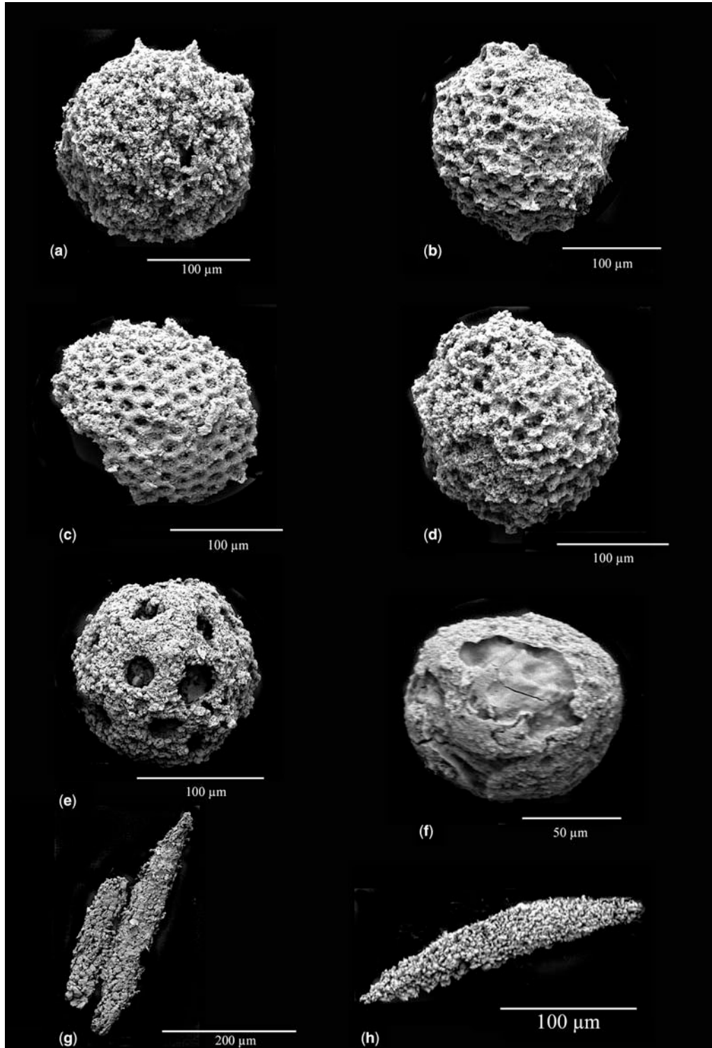
Fig. 4. Siliceous microfossils from HF acid residues of black cherts, locality Ninqiang, S. Shaanxi, Kuanchuanpu Formation. (a, b, c, d) Spherical radiolarian skeletons with lattice spheres (b, c, d) and short, triangular spines (a). Residue and matrix of the rock is strongly dominated by monaxon sponge spicules (g, h), along with silica spherules, probably representing radiolarian Steinkerns (e, f).
