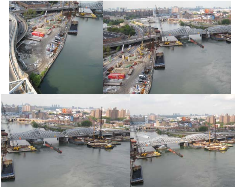
Shield Removal in September 2008 as Seen From the RFK Bridge.
