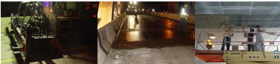
Contract #6 in 2006: Microsurfacing the North Upper Roadway. Repairing the 59 th Street Overpass.
