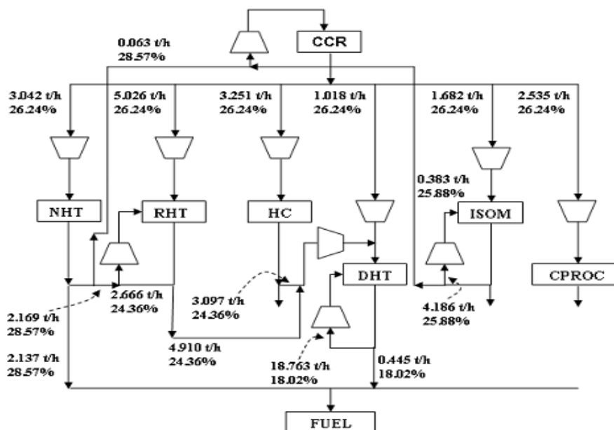
Figure 1 Flexible hydrogen network design obtained using multi-period hydrogen management.
