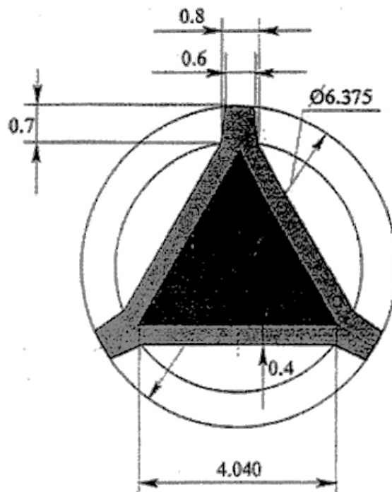
Figure 12. Triangular fuel element configuration.
