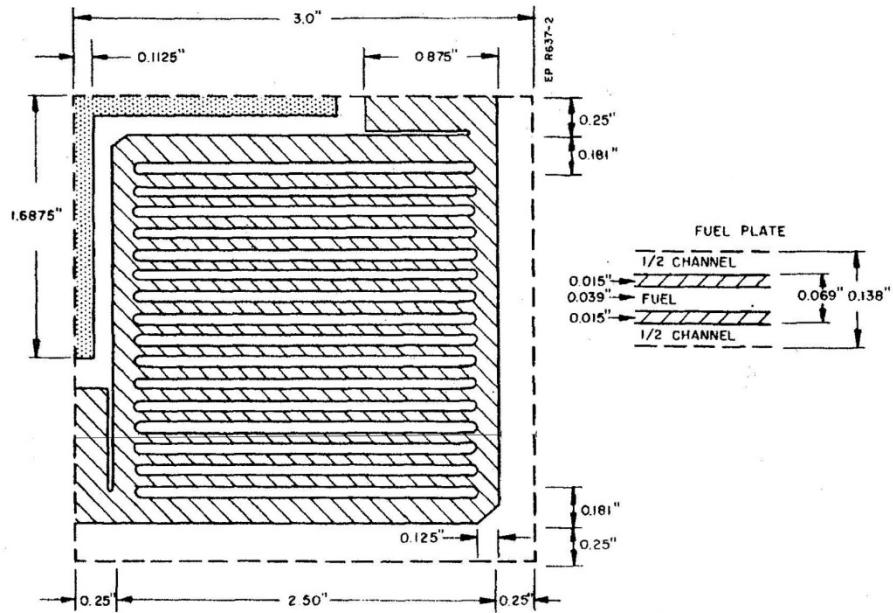
Figure 13. Plate fuel element configuration.
