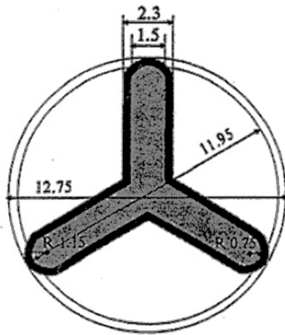
Figure 11. Spiral fuel element configuration.
