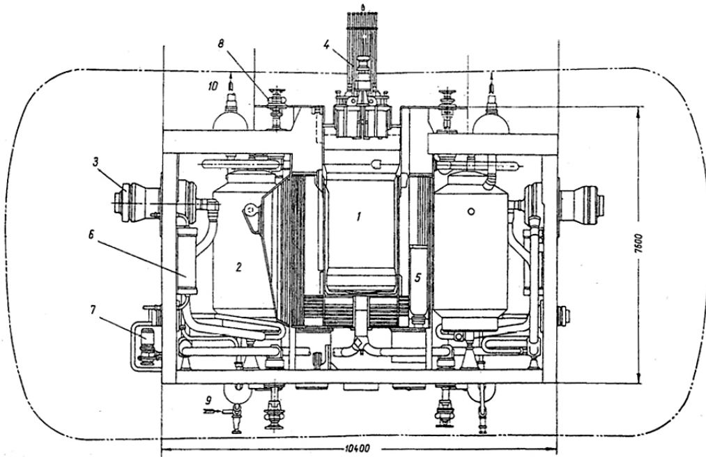
Figure 8. Components of OK-150 plant. 1: Reactor, 2: Steam generator, 3: Main circulation pumps, 4: Emergency cooling pump, 5: Pressurizers, 6: Filter, 7: Filter cooler.
