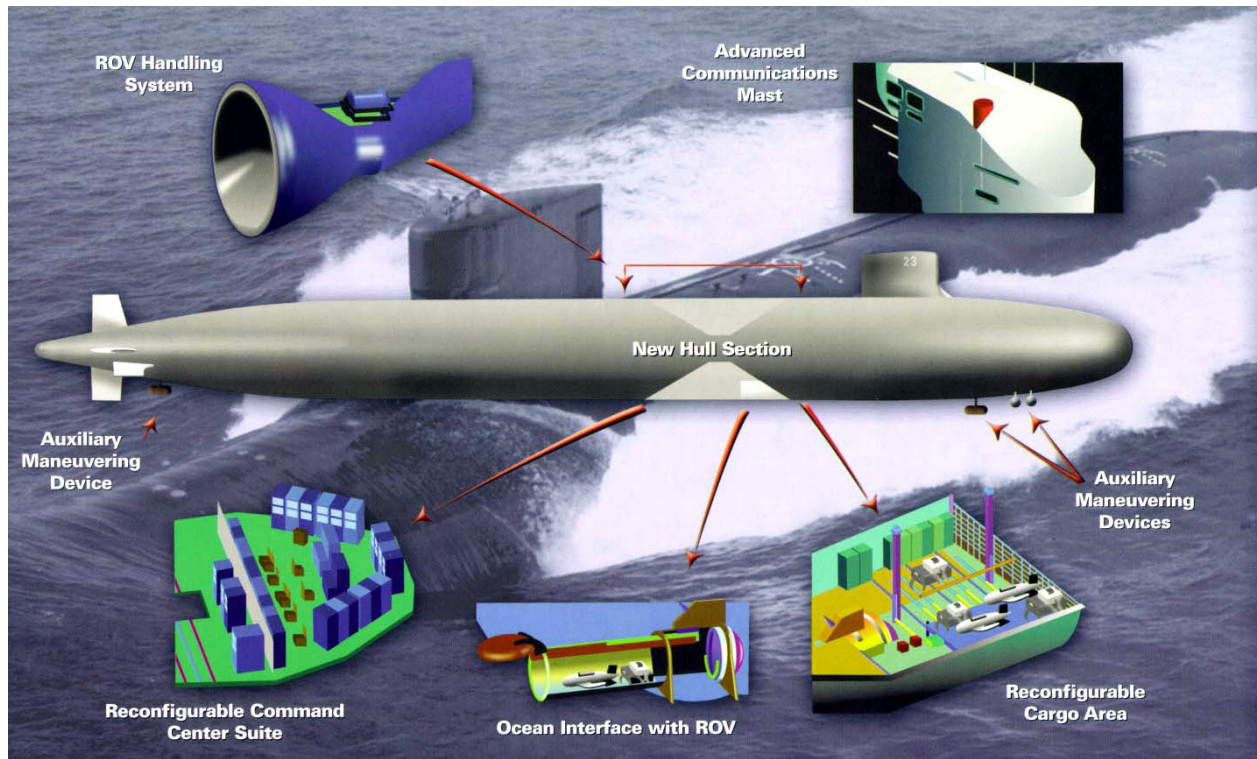
Figure 26. Special features of the SSN 23 Jimmy Carter.
