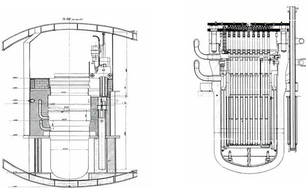
Figure 9. Layout of OK-150 plant. 1: Reactor, 2: Steam generator, 3: Main circulation pumps, 4: Control rod drives mechanism, 5: Filter, 6: Cooler, 7: Emergency cooling pump, 8: Primary circuit pressure relief valve, 9: Feedwater inlet, 10: Steam outlet.
