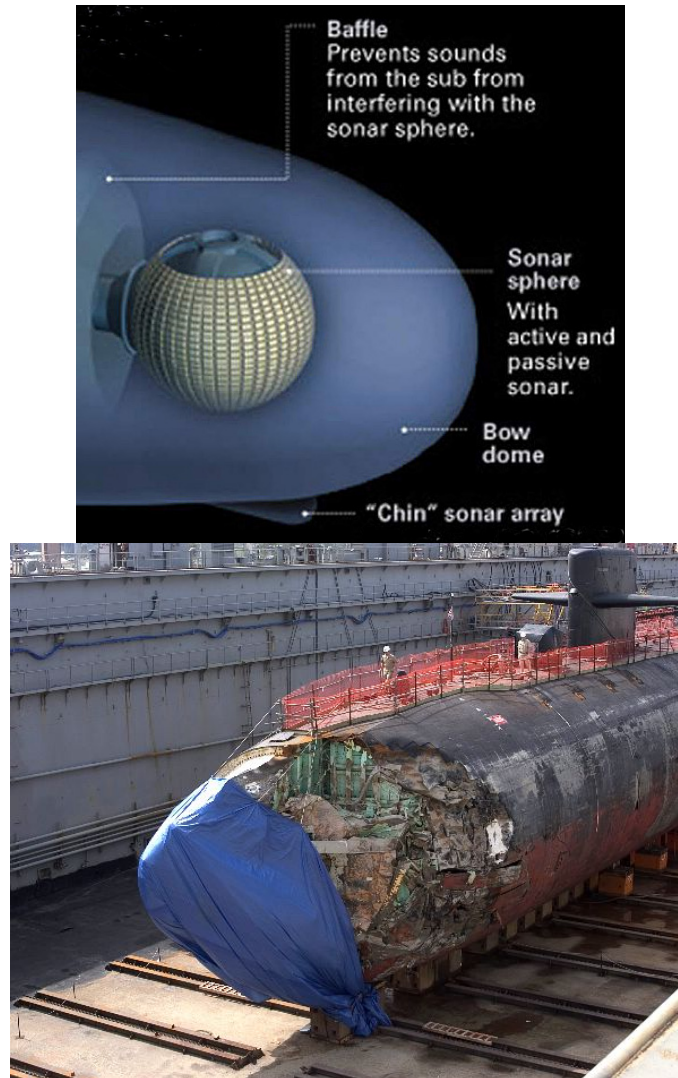
Figure 36. USS San Francisco accident, January 8, 2005. Damage from the glancing collision to the bow dome and to the double hull structure can be observed. A bulge over the hull can also be noticed.
