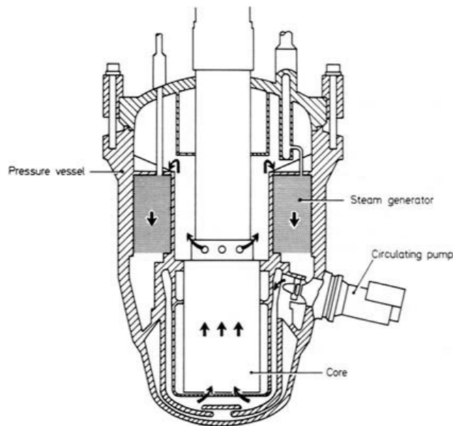
Figure 7. Integral type of naval reactor vessel [4].
