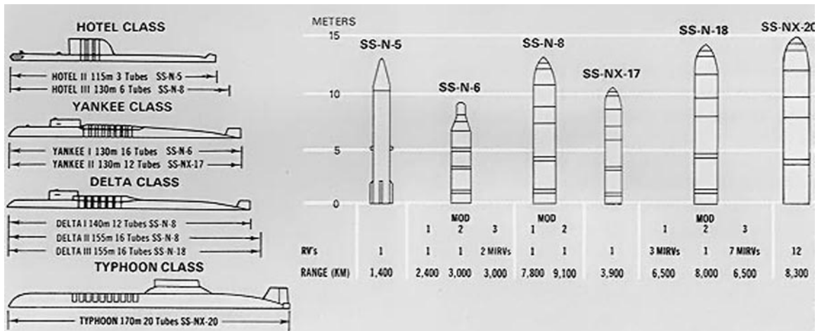
Figure 22. Nuclear Ballistic Missile Submarines and their missiles characteristics.
