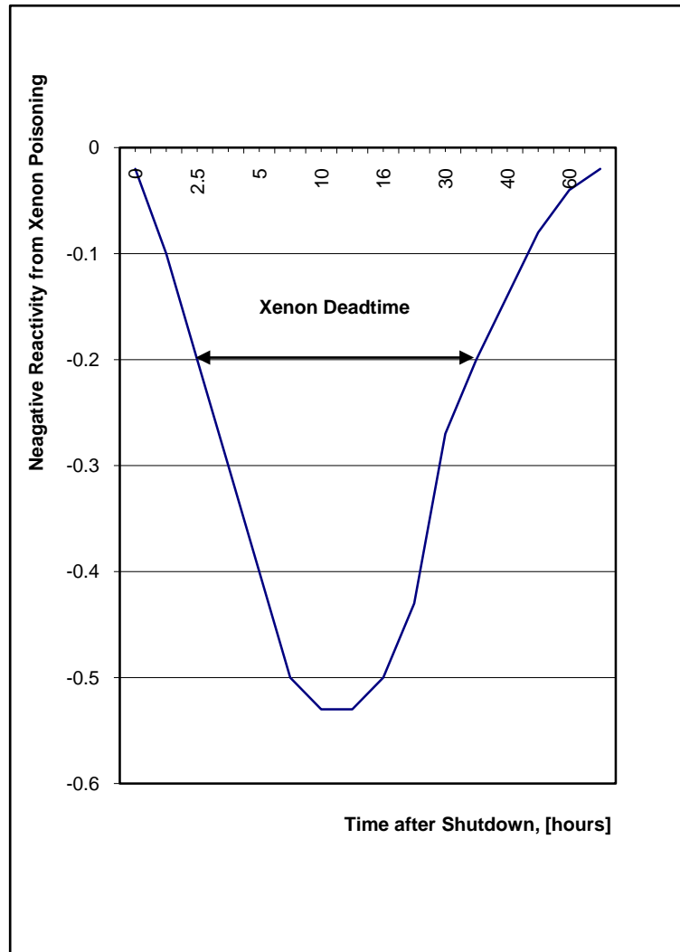
Figure 14. Negative reactivity due to xenon poisoning. Flux = 5 \times 10^{14} [n/(cm 2 .sec)].
