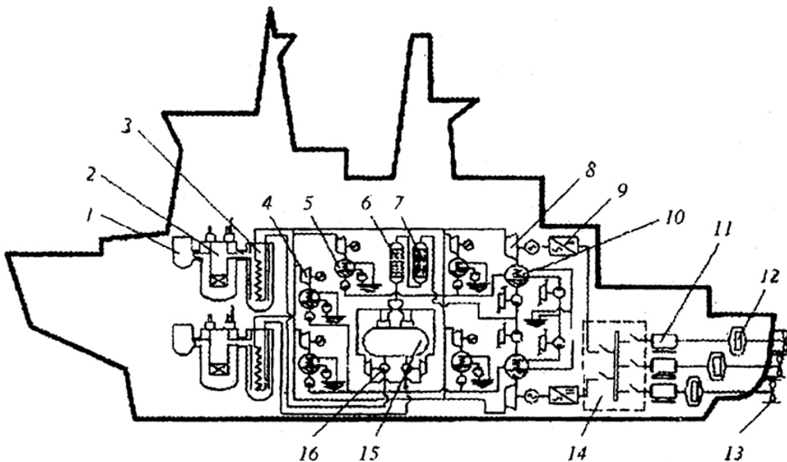
Figure 34. Nuclear reactor components of the icebreaker Arktika. 1: Circulation pumps, 2: Reactor vessel, 3: Steam generator, 4: Auxiliary turbo generator, 5: Condenser, 6: Ion exchange resins filter, 7: Mechanical filter, 8: Main turbo electrical generator, 9: Converter, 10: Main condenser, 11: Electrical propeller motor, 12: Intermediate bearing, 13: Screw propeller, 14: Circuit breaker for propeller motor, 15: Deaerator, 16: Turbo feed pump.
