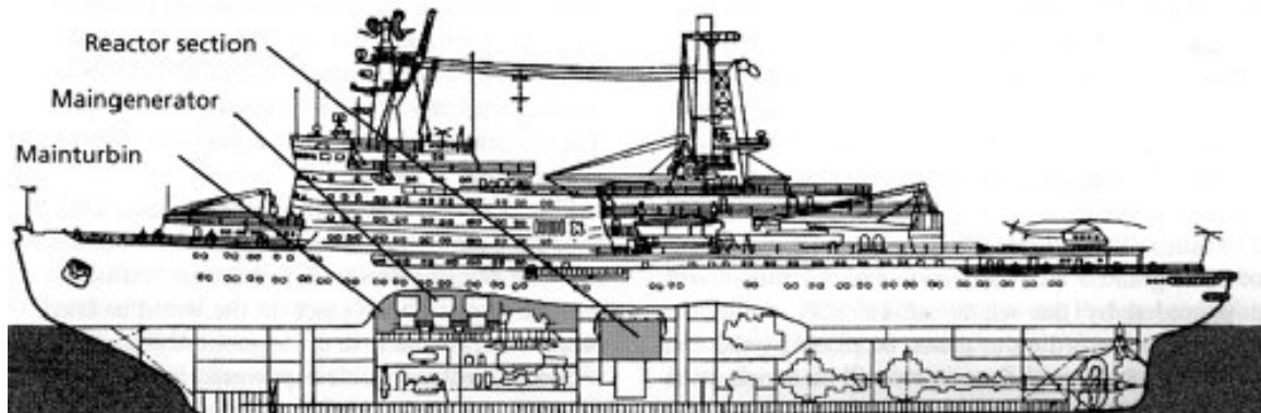
Figure 33. Schematic of Russian Nuclear icebreaker Arktika showing emplacement of nuclear reactor at its center.
