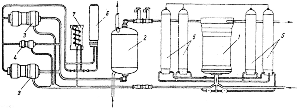
Figure 8. Components of OK-150 plant. 1: Reactor, 2: Steam generator, 3: Main circulation pumps, 4: Emergency cooling pump, 5: Pressurizers, 6: Filter, 7: Filter cooler.
