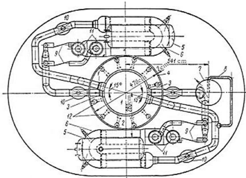
Figure 5. Loop type of naval reactor design for the nuclear ship Savannah. The reactor core is surrounded by the heat exchangers and the steam drums. The horizontal steam generator was replaced by a vertical tube steam generator and an integrated system in future designs. 1: Reactor core, 2: Water shield, 3: Coolant inlet, 4: Pb Shield layer, 5: Steam drum, 6: Heat exchanger, 7: Pressurizer, or volume compensator, 8: Equalizer line, 9: Cutoff channel, 10: Gate valve, 11: Coolant pumps, 12: Channels with apparatus [5].
