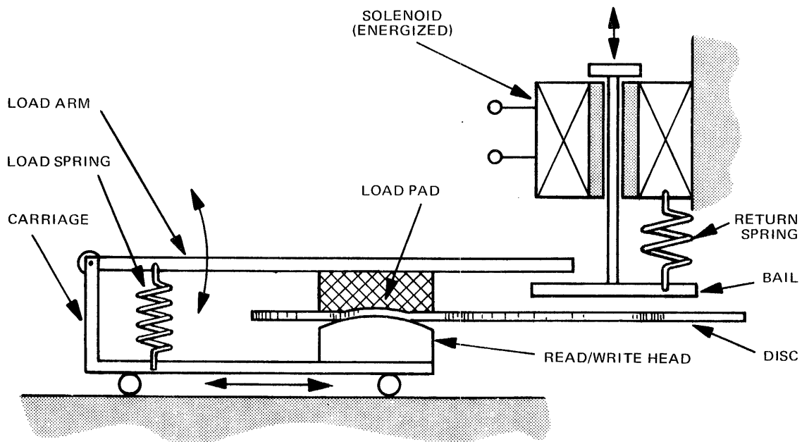
Figure 2. Head Load Mechanical Assembly
