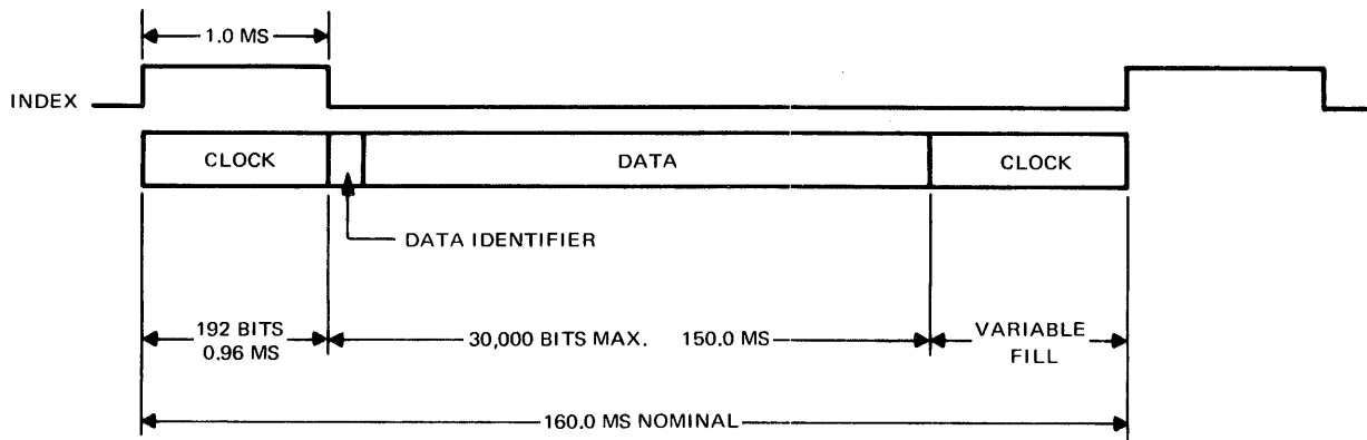
Figure 9. Index Recording Format
