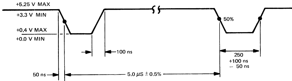
SEP DATA AND SEP CLOCK SIGNALS
