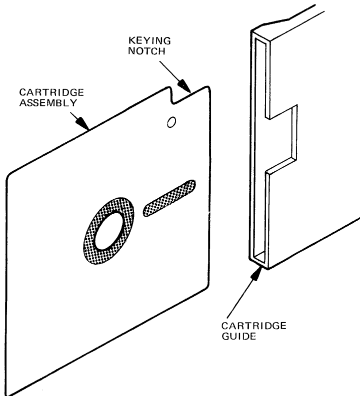
Figure 17. Cartridge Loading
