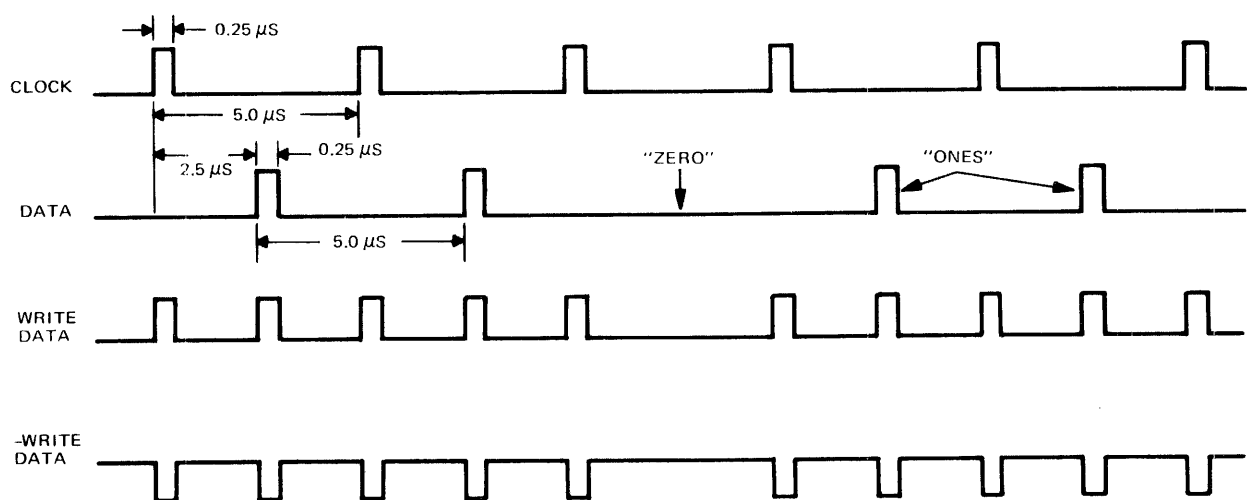
Figure 6. Write Data Timing Function
