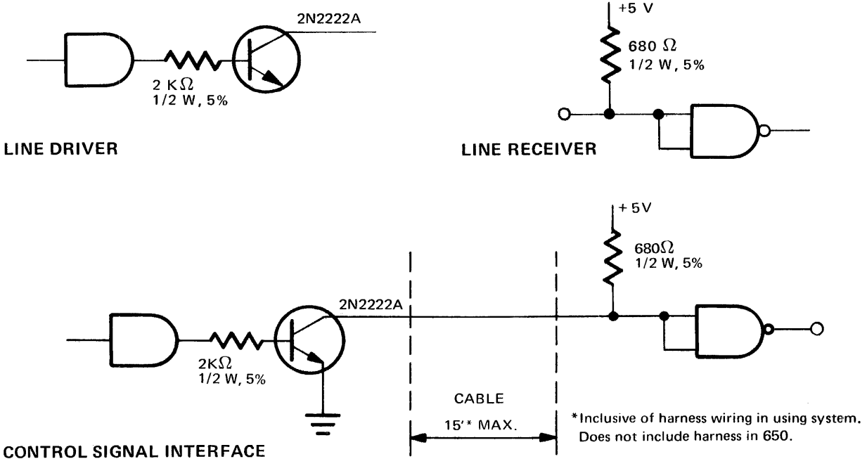
Figure 14. Control Line Driver and Line Receiver
