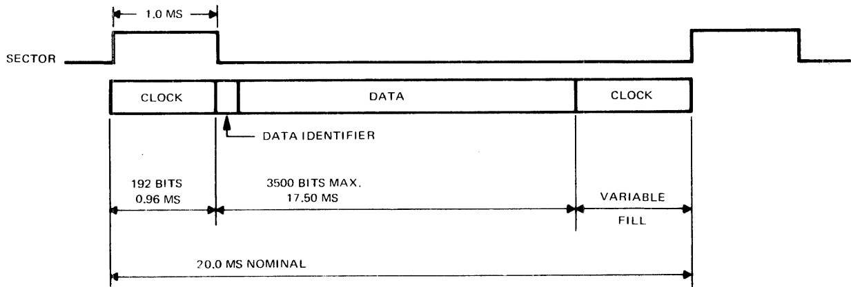
Figure 8. Sector Recording Format
