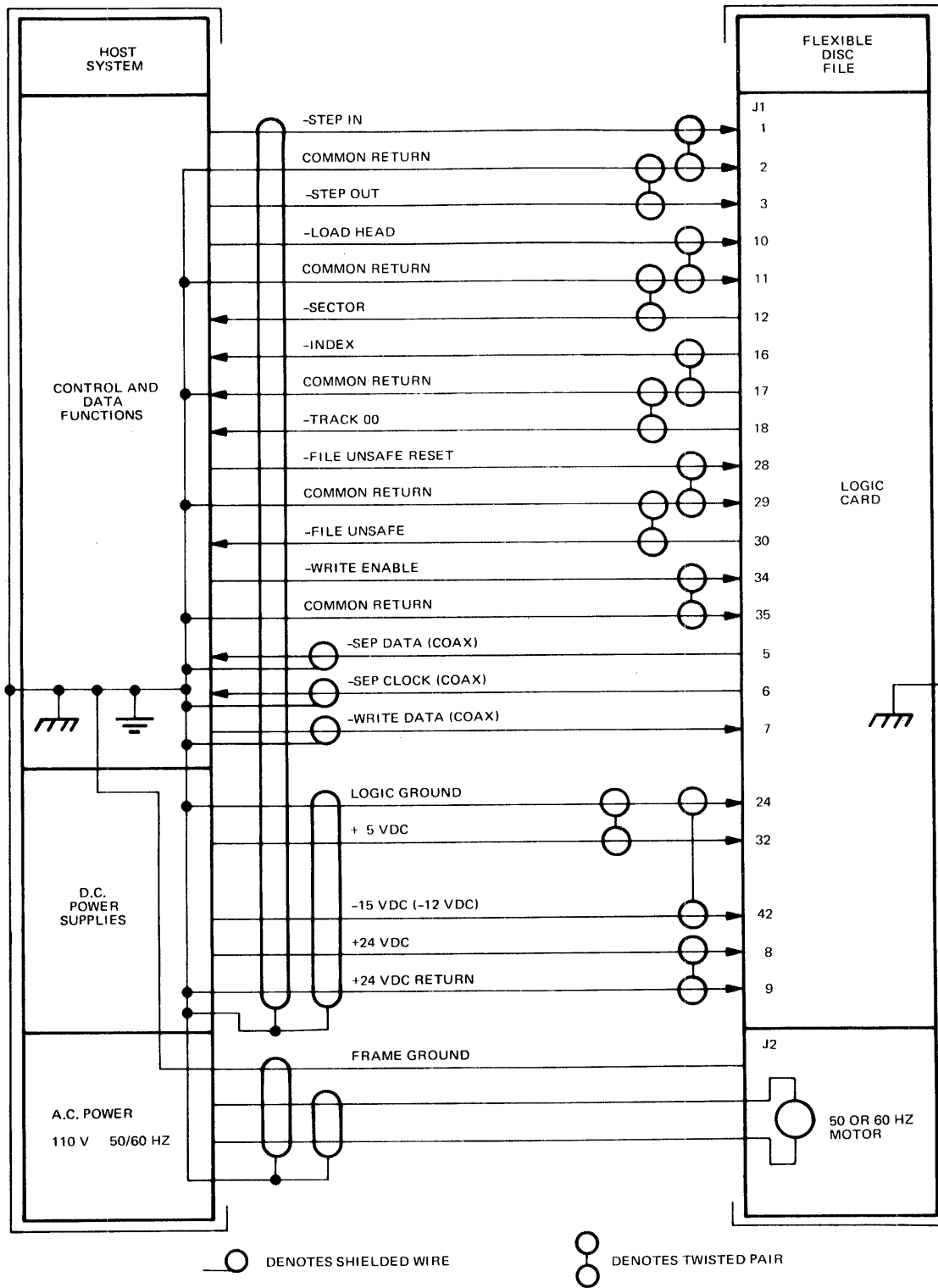
Figure 13. Flexible Disc Wiring Diagram
