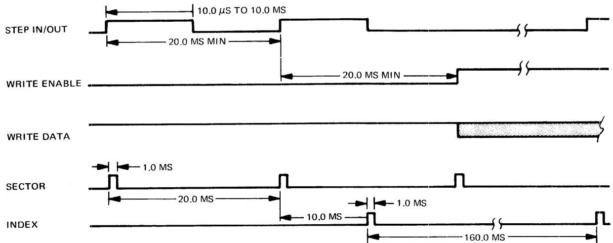
Figure 5. Typical Write Sequence
