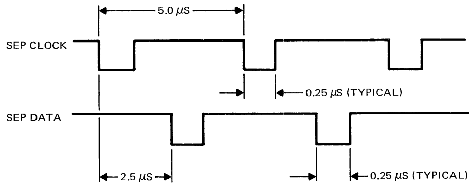
Figure 7. Separated Clock and Data
