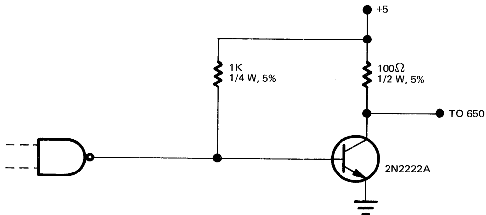
WRITE DATA DRIVER
