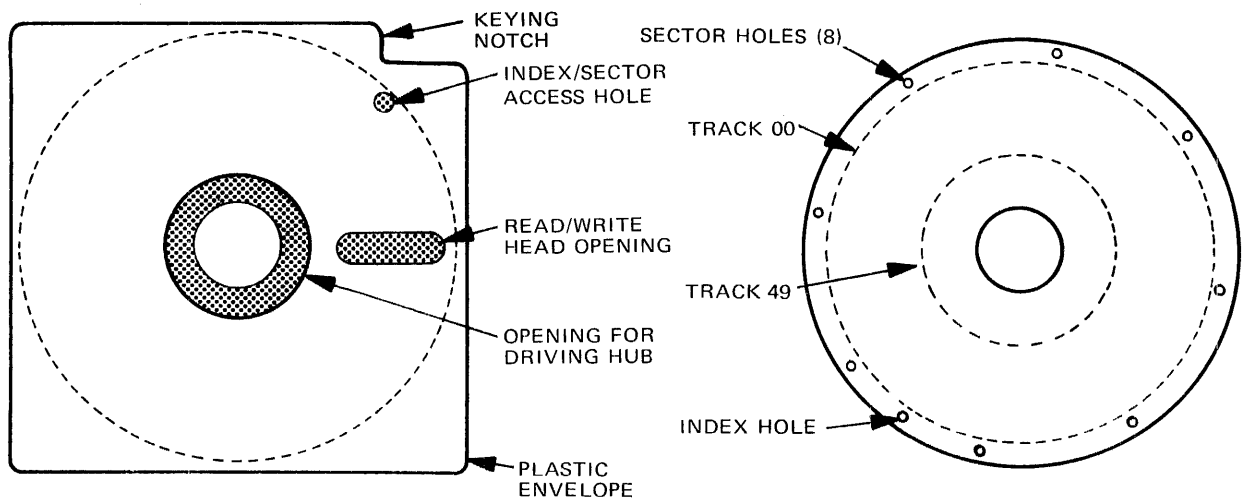
Figure 3. Disc Cartridge and Disc Configuration
