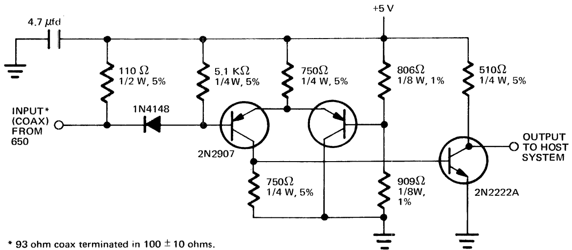
SEP DATA AND SEP CLOCK RECEIVERS
