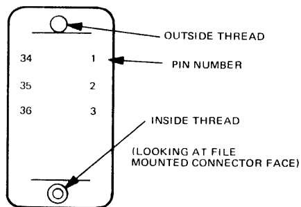
Figure 10. Signal Connector Keying
