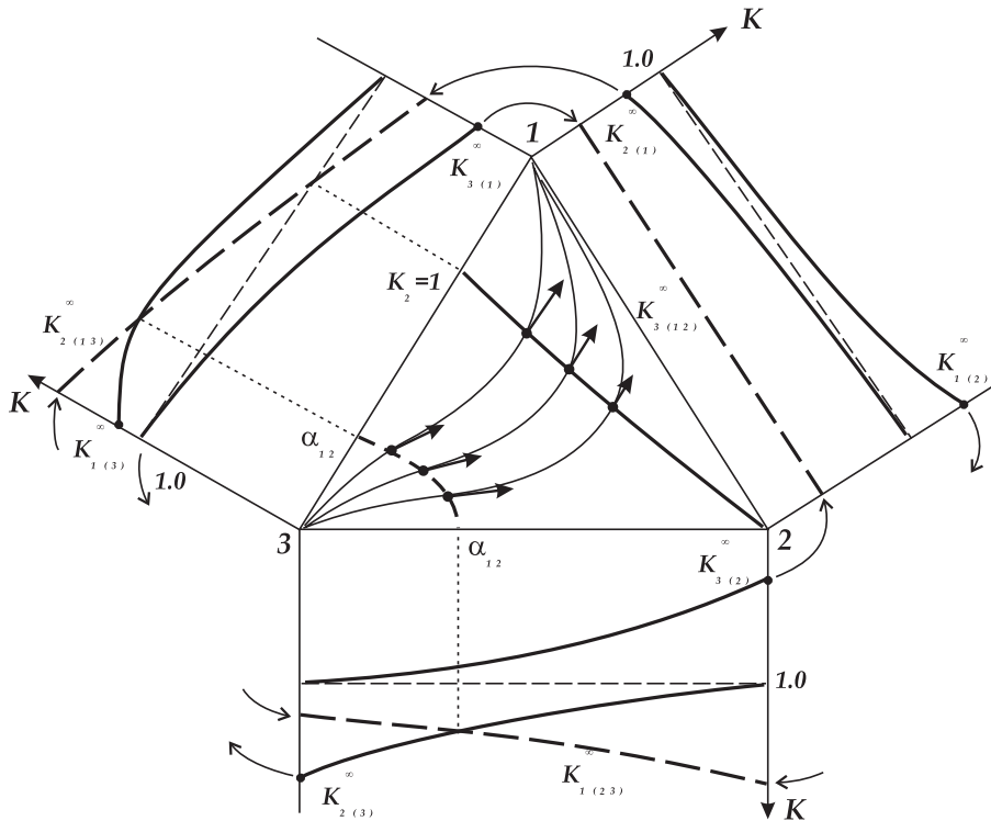
Figure 3.40: Univolatility and unidistribution line diagram and phase portrait of the residue curve map for a zeotropic mixture 1-2-3 where the binary constituents 1-3 are a mixture of Type 2' ( S-shaped residue curves ).
