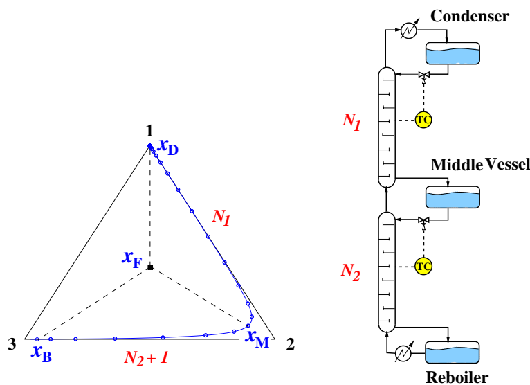
Figure 7.2: Closed middle vessel (three-vessel) batch distillation of ternary zeotropic mixture. Simultaneous separation of all three components. Steady state composition profile (solid line with open circles) and material balance lines (dashed).
