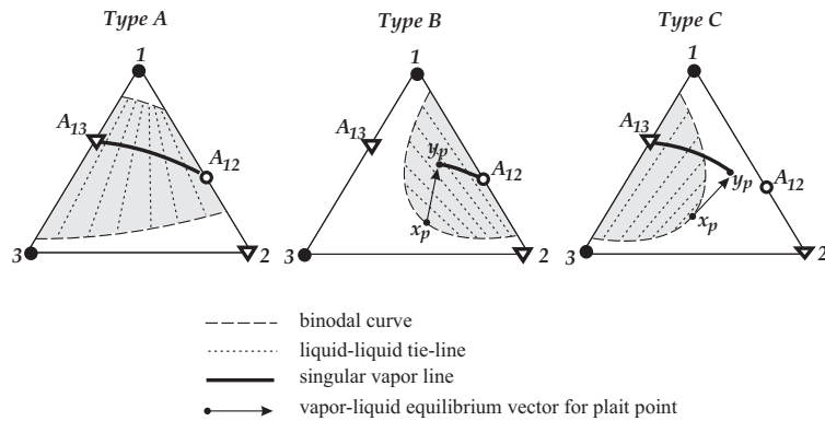
Figure 3.18: Three possible types of heterogeneity for a mixture with the boiling temperature structure of Serafimov's class 2.0-2b. The singular points are indicated by \bullet stable node, \circ unstable node, and \nabla saddle.
