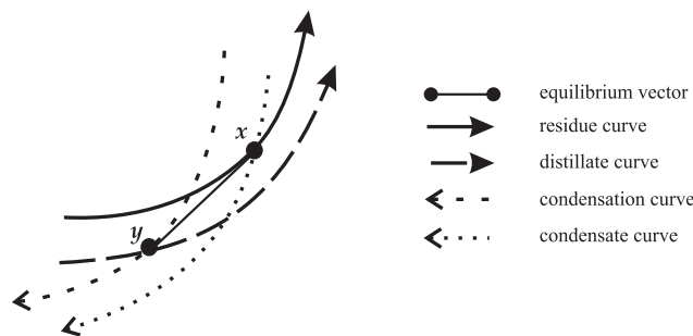
Figure 3.11: Vapor and liquid composition trajectories of open evaporation and open condensation going through the points x and y of an equilibrium vector in the composition space.
