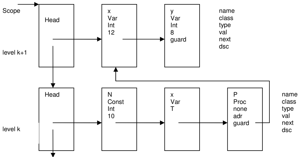
Figure 12.6. Symbol table representing two scopes.
