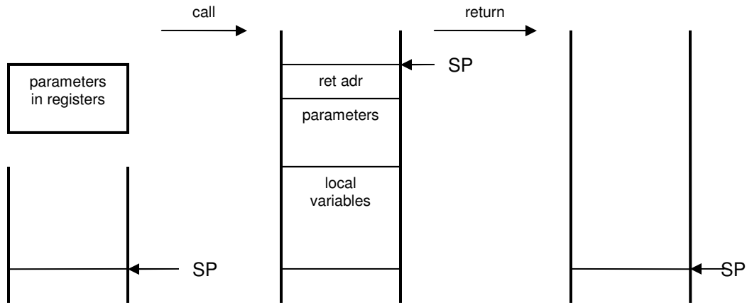
Figure 12.5. Parameter allocation.in registers
