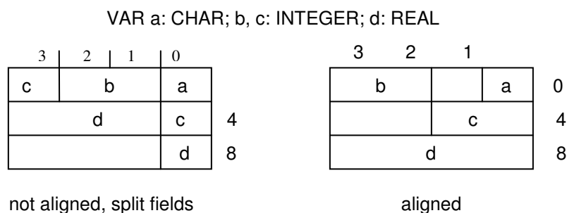
Figure 8.4. Alignment in address computation.
