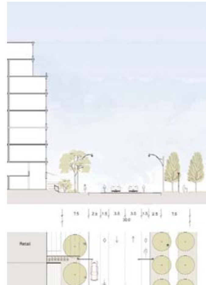
Bayview Avenue plan and section
