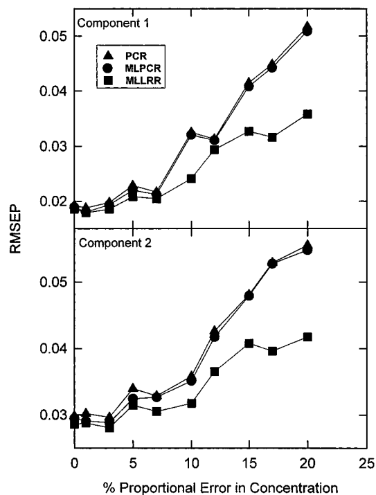
Figure 6. Comparison of calibration methods applied to simulated data with errors in both spectra and concentrations (data set 3).
