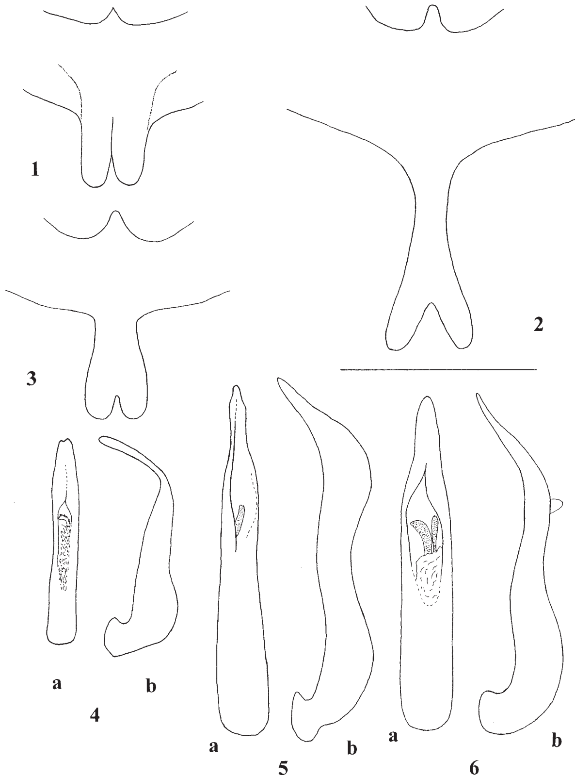
Figs 1-6. Apophyllia spp: 1, 4 — A. celebensis , 2, 5 — A. furcigera , 3, 6 — A. pectoralis , 1-3 — male metasternum, 4-6 — aedeagus (a — dorsal view, b — lateral view). Scale 1 mm.
