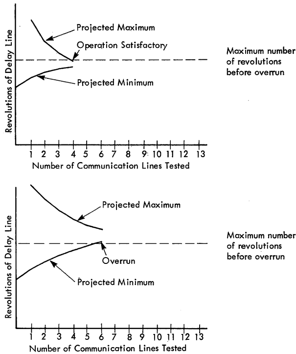
Figure 16. Projection of Delay Line Revolution Requirements
