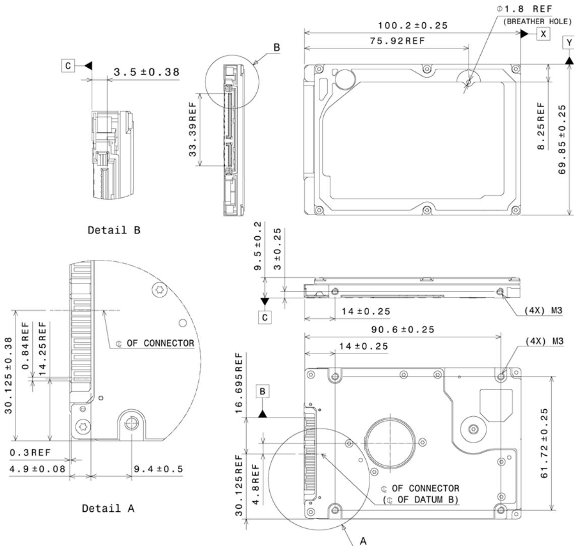
Figure 2. Mounting hole locations
