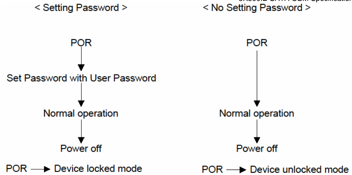
Figure 5 Initial Setting
