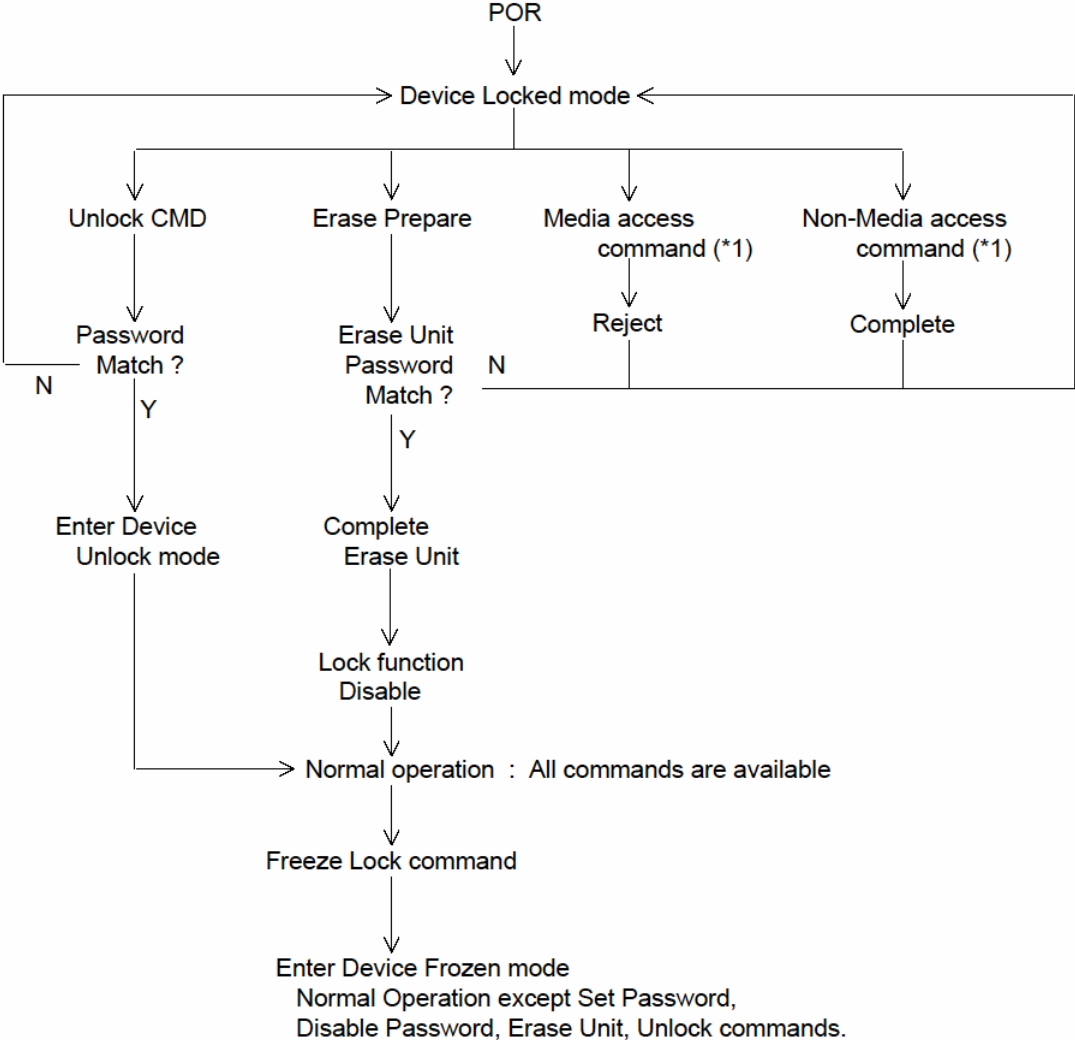
Figure 6 Usual Operation
