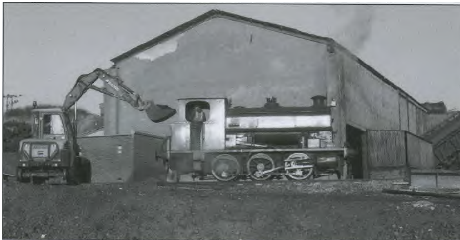
No.3, glinting in the morning sun, receives coal from a Mecalac at the Salt Mines. [I Pryce]
