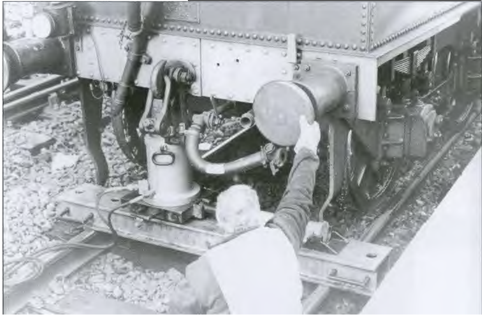
At Lisburn on 27 Aug 2005 the rear wheels of 186's tender are about to be re-railed. Those who have wrestled with traversing screw jacks must envy NIR this piece of kit! [C Friel]
