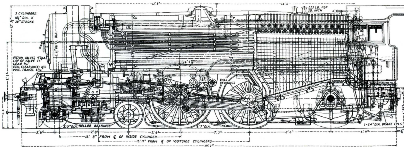
Sectional elevation drawing showing general arrangements of new three-cylinder 4-6-0 type express locomotive, Great Southern Railways of Ire. Built at the company's Inchicore works, Dublin. By Mr. E. C. Bredin, M.I.Mech.E., M.I.Loco.E., Chief Mechanical Engineer
