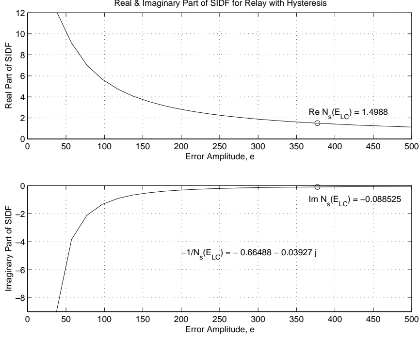
Figure 6: Complex-valued SIDF for Relay with Hysteresis
