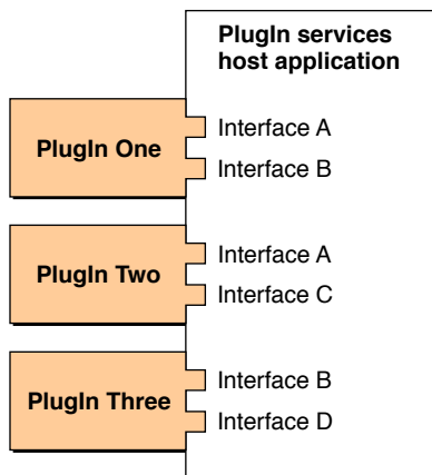
Figure 1 A CFPlugIn host with three plug-ins.
