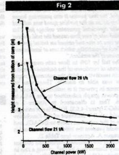
▲ Boundary of start of boiling in the Chernobyl fuel channels. Reactor power = 1.25 \times 10^5 channel power.
