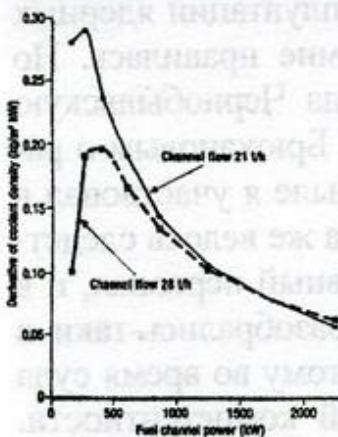
▲ Derivative of coolant density ( -\Delta \text{density}/\Delta \text{channel power} ) as a function of channel power.
