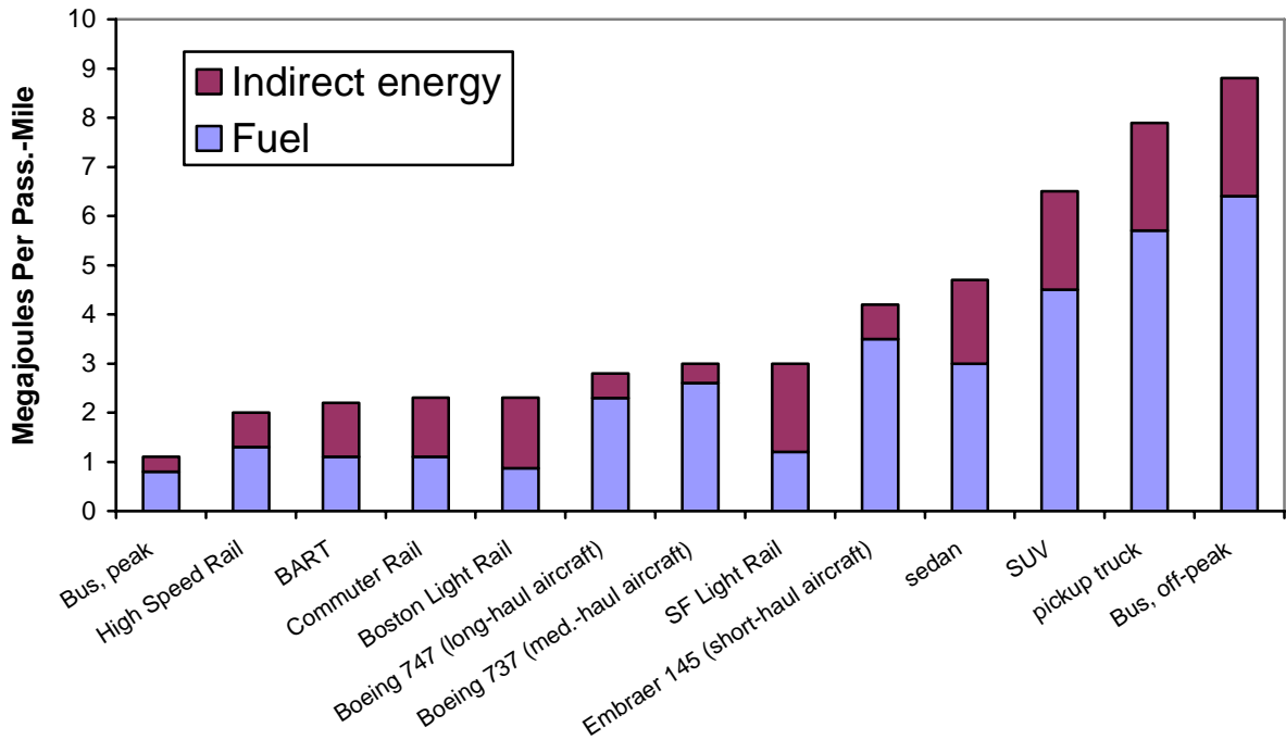
Figure 5.10.4-1 Lifecycle Energy Consumption and Emissions 39
