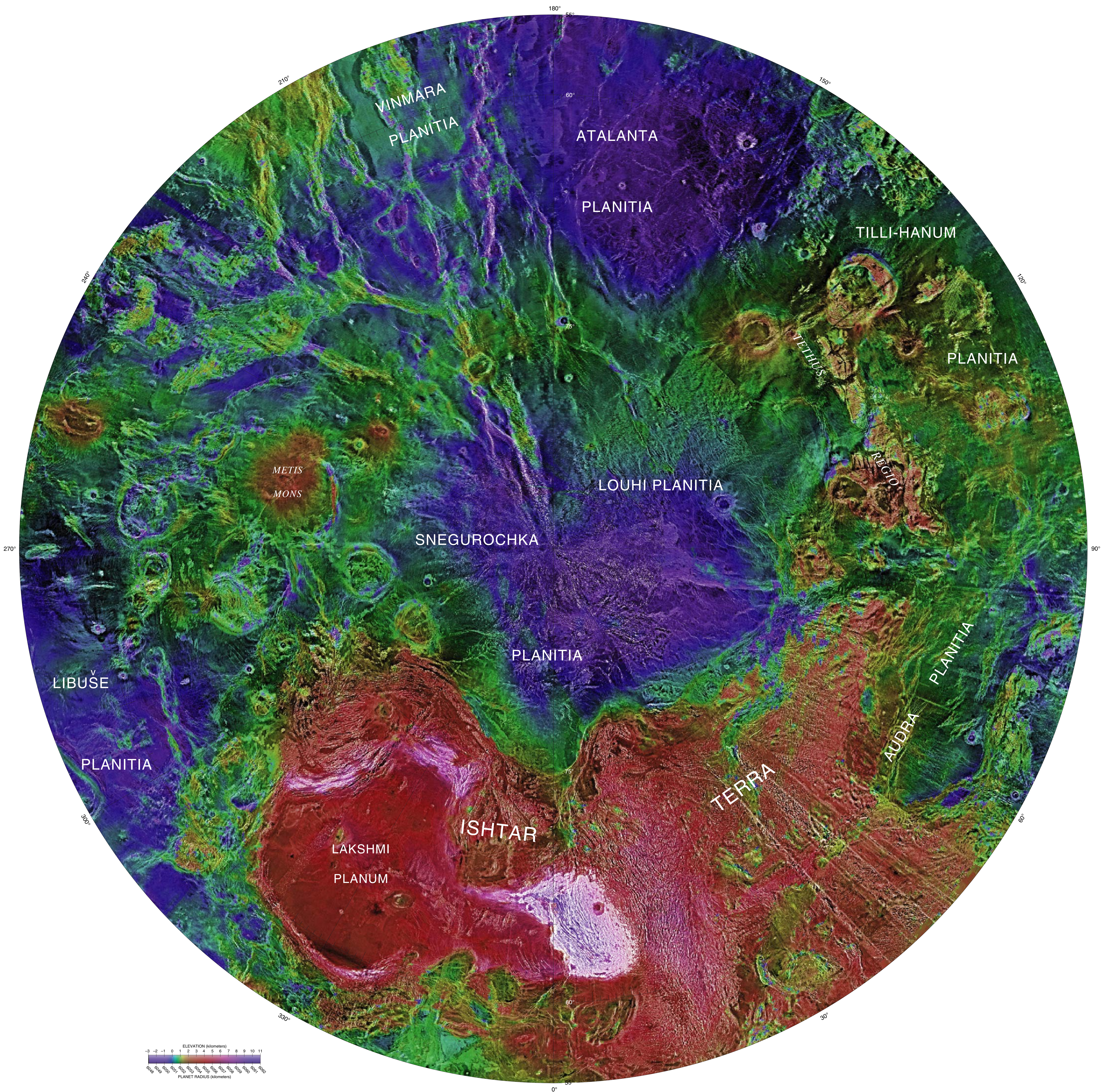
ALTIMETRIC RADAR IMAGE MAP OF THE ISHTAR TERRA REGION OF VENUS
