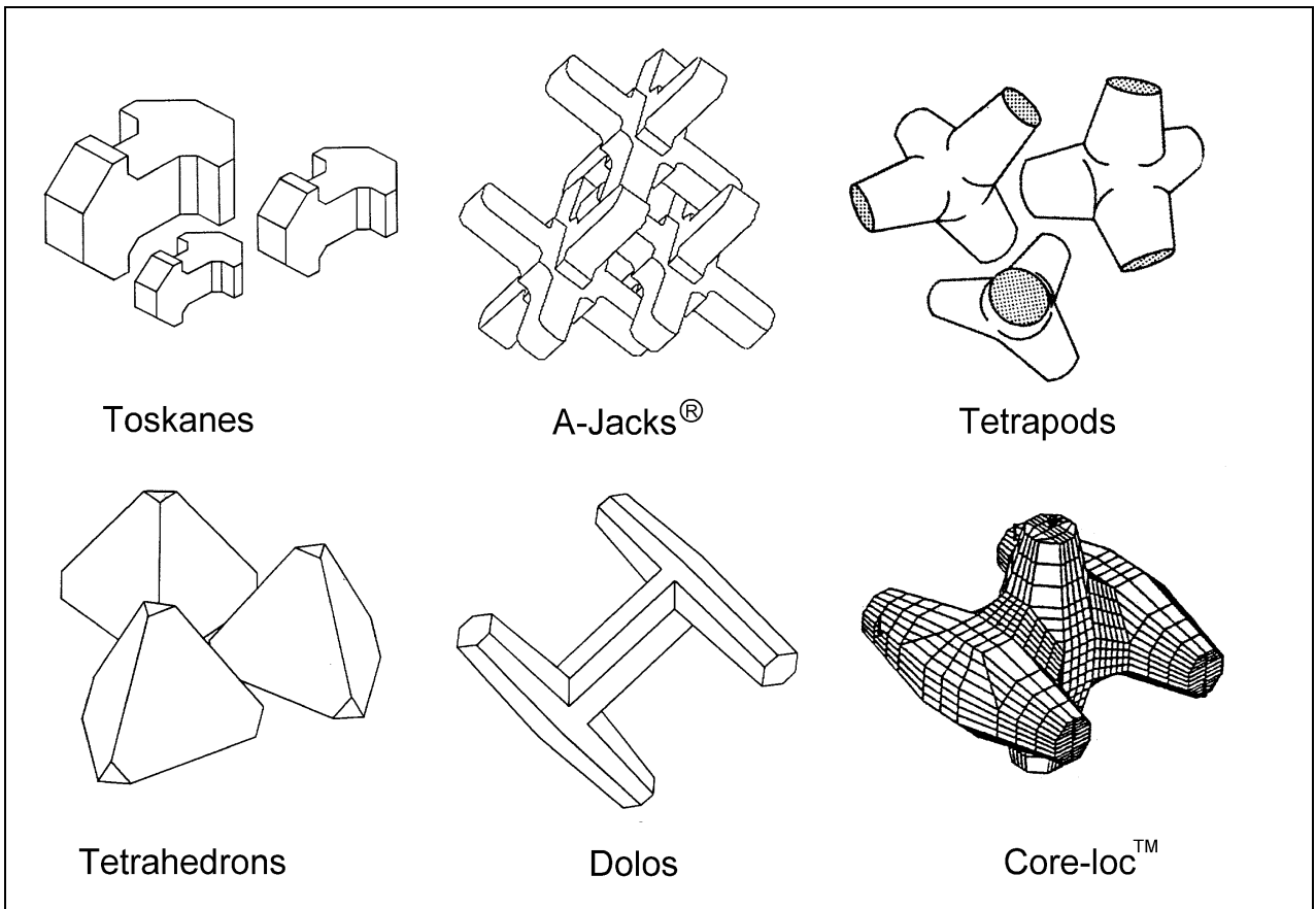
Figure 6.1. Armor units.
