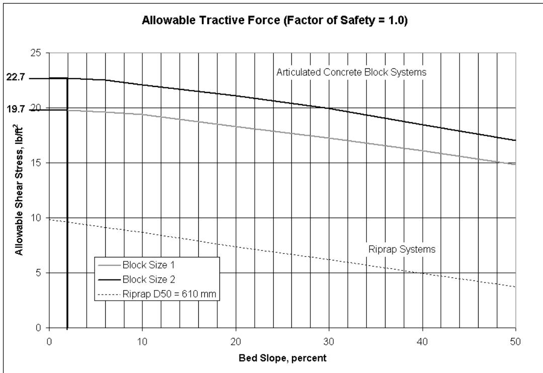
Figure 4.6. Plot of allowable shear stress vs. bed slope (English).
