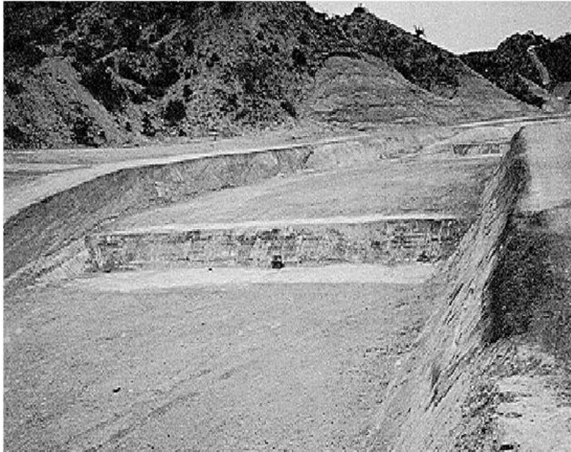
Figure 2.4. Soil cement bank protection and drop structures in Laughlin, NV. (7)
