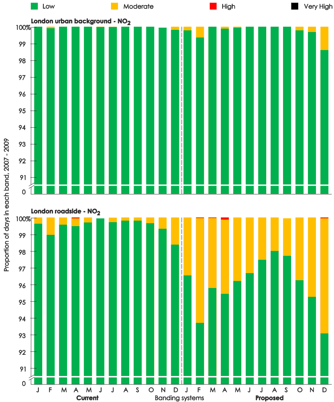
Figure A11-2: Comparison between the current and proposed banding systems for NO 2 The upper panel shows measurements from 28 background sites and the lower panel shows measurements from 34 kerb/roadside sites in London
