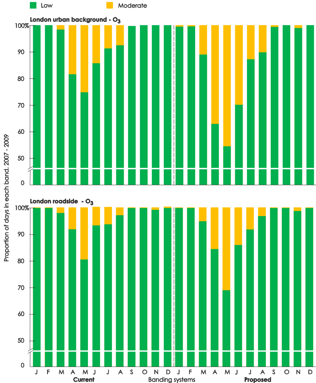
Figure A11-1: Comparison between the current and proposed banding systems for O 3 The upper panel shows measurements from 22 background sites and the lower panel shows measurements from 10 kerb/roadside sites in London
