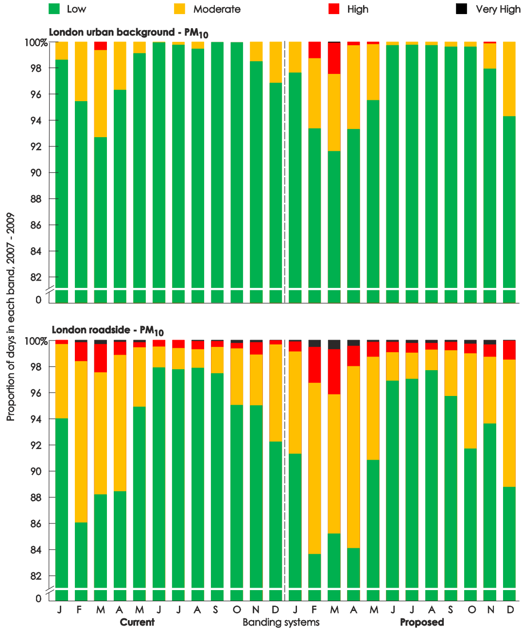
Figure A11-3: Comparison between the current and proposed banding systems for PM 10 The upper panel shows measurements from 17 background sites and the lower panel shows measurements from 28 kerb/roadside sites in London
