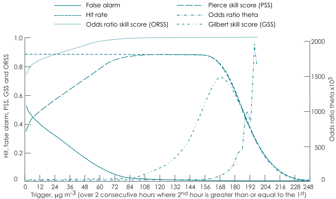
Figure A9-6: Evaluation of each possible trigger for O 3 High or above using metrics from Stephenson (2000)
