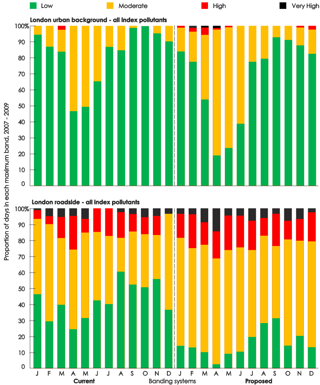
Figure A11-5: Comparison between the current and proposed banding systems for overall pollution
