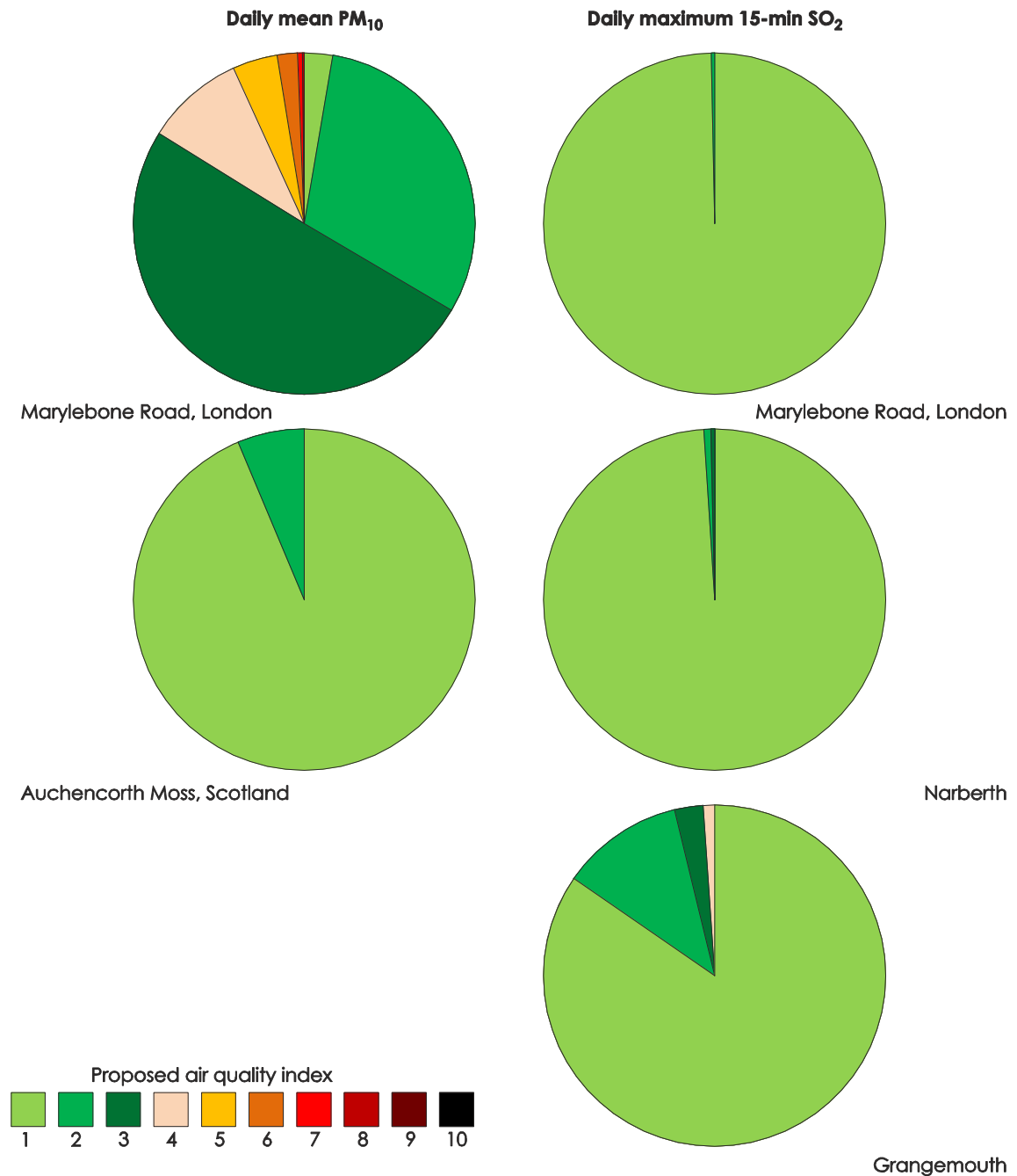
Figure 4-1: Proportion of days in each category in the proposed air quality index for PM 10 , SO 2 , NO 2 and O 3 using data for 2008 from a range of monitoring stations
