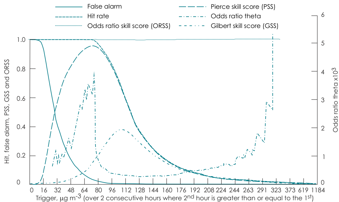
Figure A9-3: Evaluation of each possible trigger for PM 10 High or above using metrics from Stephenson (2000)
