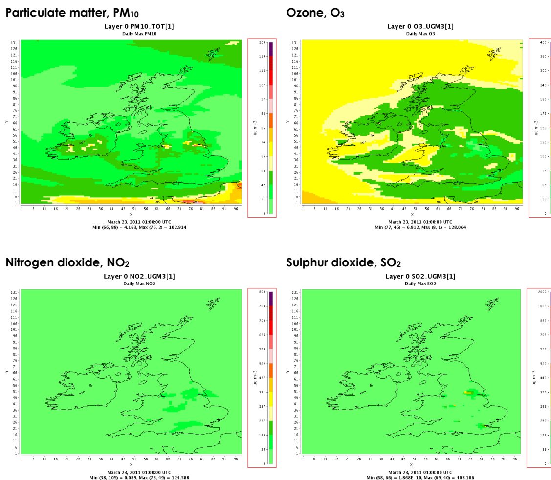
Figure A6-2: Example of index pollutants on 23 March 2011
