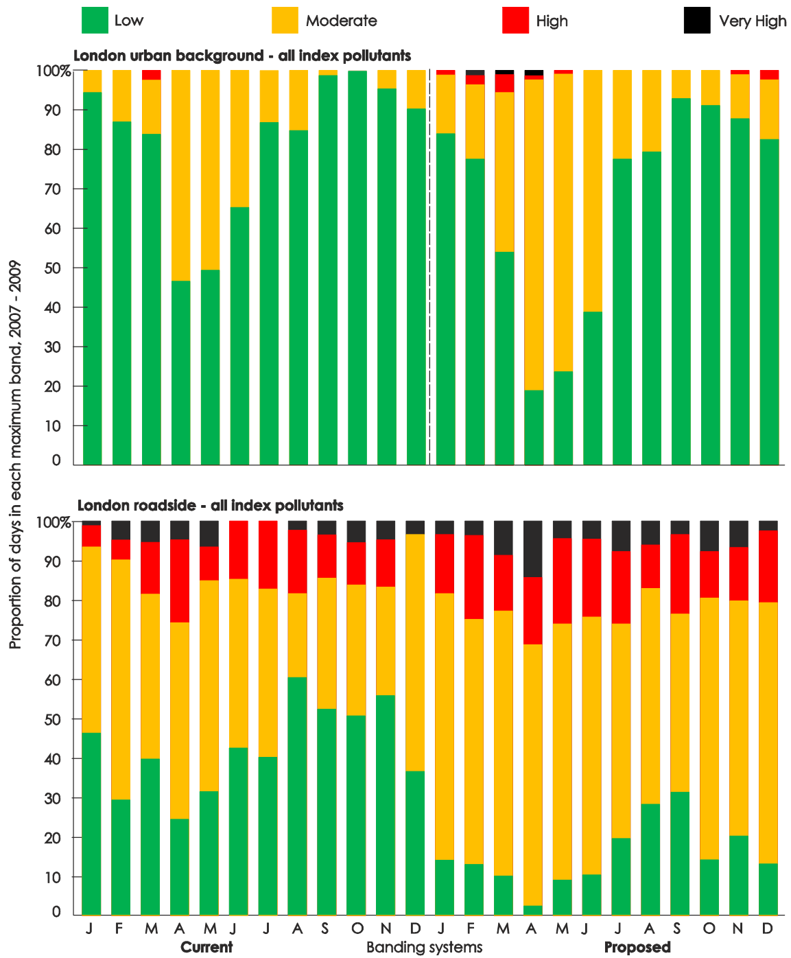
Figure 4-2: Comparison between the current and proposed banding systems for overall pollution The upper panel shows background air pollution from 32 sites and the lower panel shows air pollution from 40 kerb/roadside sites in London
