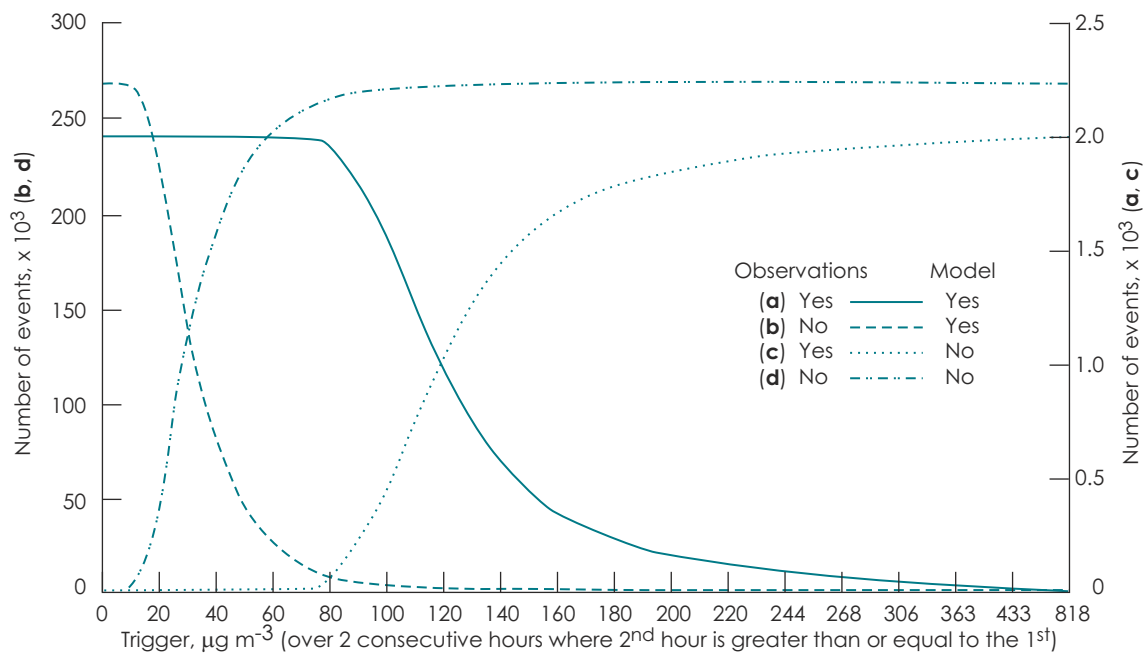
Figure A9-2: Contingency matrix outputs for PM 10 High or above for each possible trigger
