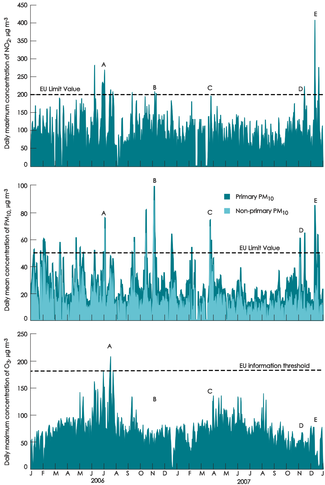
Figure A7-1: Daily concentration of NO 2 (upper panel), PM 10 (middle panel) and O 3 (lower panel) in London during 2006 and 2007
