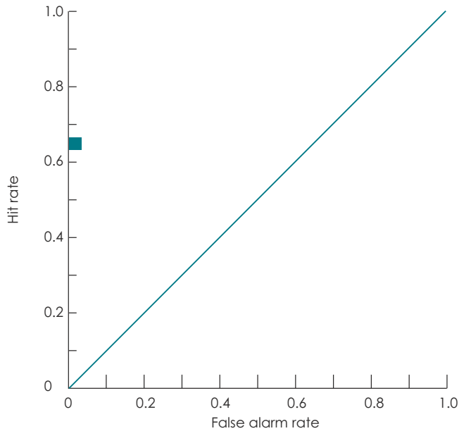
Figure A9-4: Evaluation of 107 µg m -3 trigger for PM 10 High and above using a ROC curve
