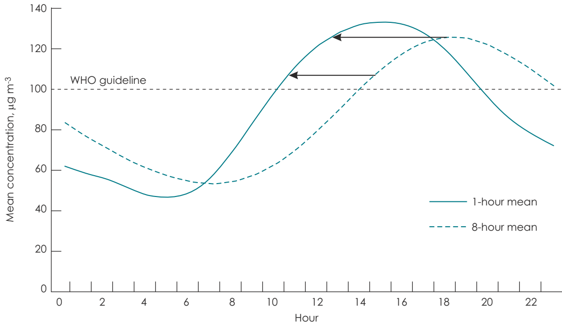
Figure A9-1: 1-hour and 8-hour mean concentrations on days when the WHO AQG was breached (data from London and Southeast England, the arrows indicate the delay between the 1- and 8-hour mean concentrations)
