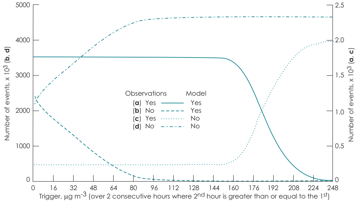
Figure A9-5: Contingency matrix outputs for O 3 High or above for each possible trigger
