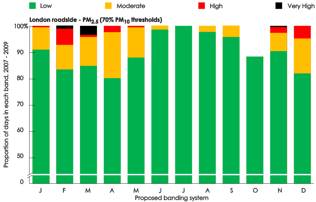
Figure A11-4: PM 2.5 at three London kerb/roadside sites using the proposed banding system (PM 2.5 thresholds are 70% of PM 10 thresholds)
