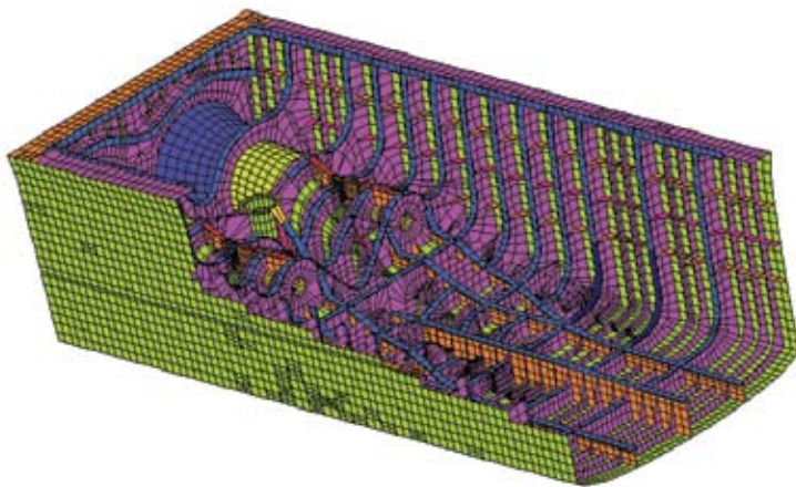
Finite Element Design Model
