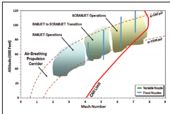
APTU Expanded CAH Envelope
