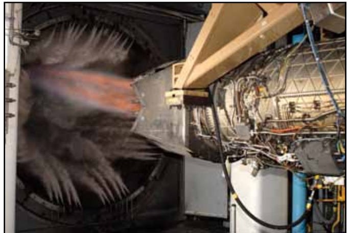
The F119 Engine for the F-22A Raptor being Tested in SL-2
