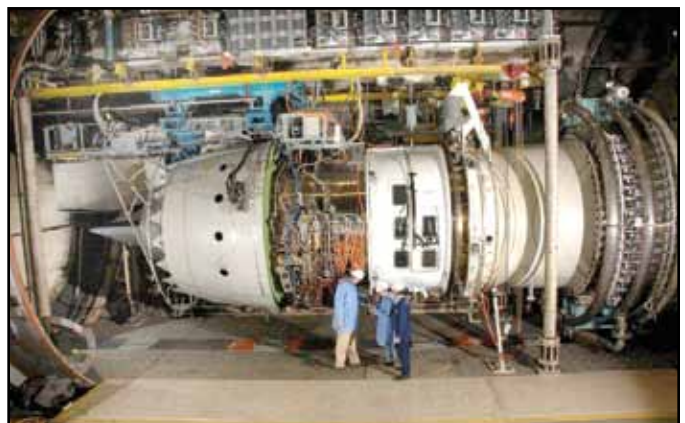
The Trent 1000 Engine for the Boeing 787 Installed in C-2
