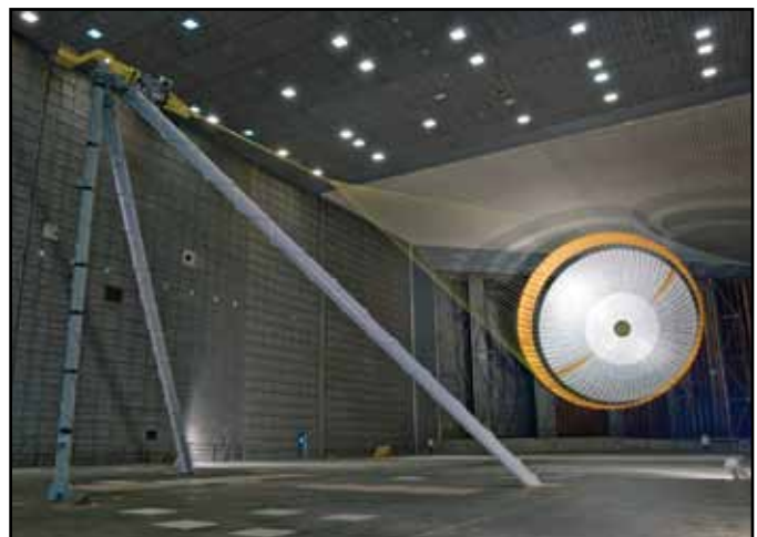
JPL Mars Science Laboratory Parachute Testing
