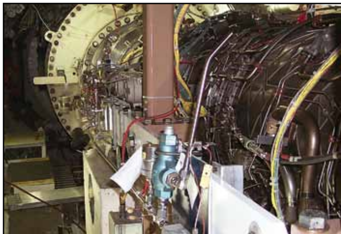
The F100 Engine Installed in T-4
