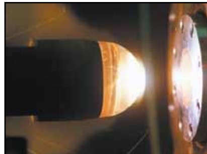
Leading-Edge Model in H2 Tunnel
