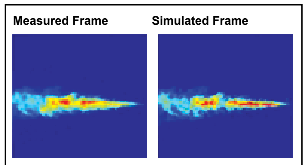
Measured and Simulated Tactical Missile Plumes
