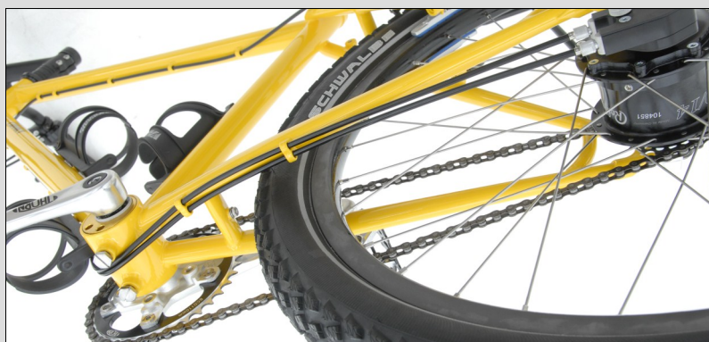
Above, you can see a worm's eye view of the superb cable routing to the EX box on the Nomad Mk2. The stainless steel eccentric screws and bosses can also be seen.
