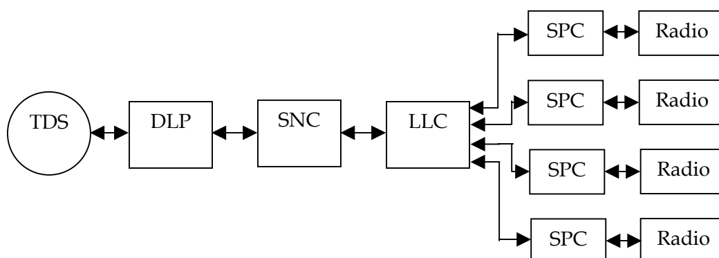
Figure 1: Link-22 system architecture
