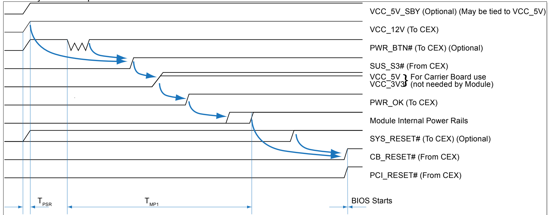
Figure 51: AT Style Power Up Boot
