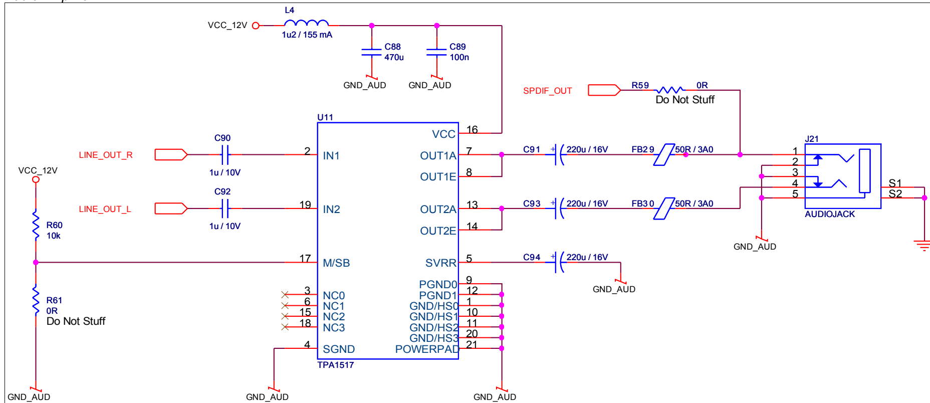
Figure 32: Audio Amplifier
