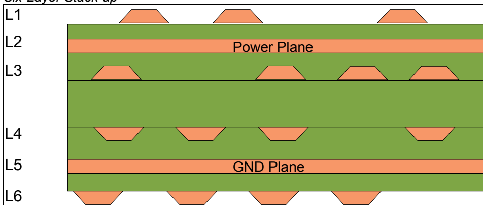
Figure 55: Six-Layer Stack-up
