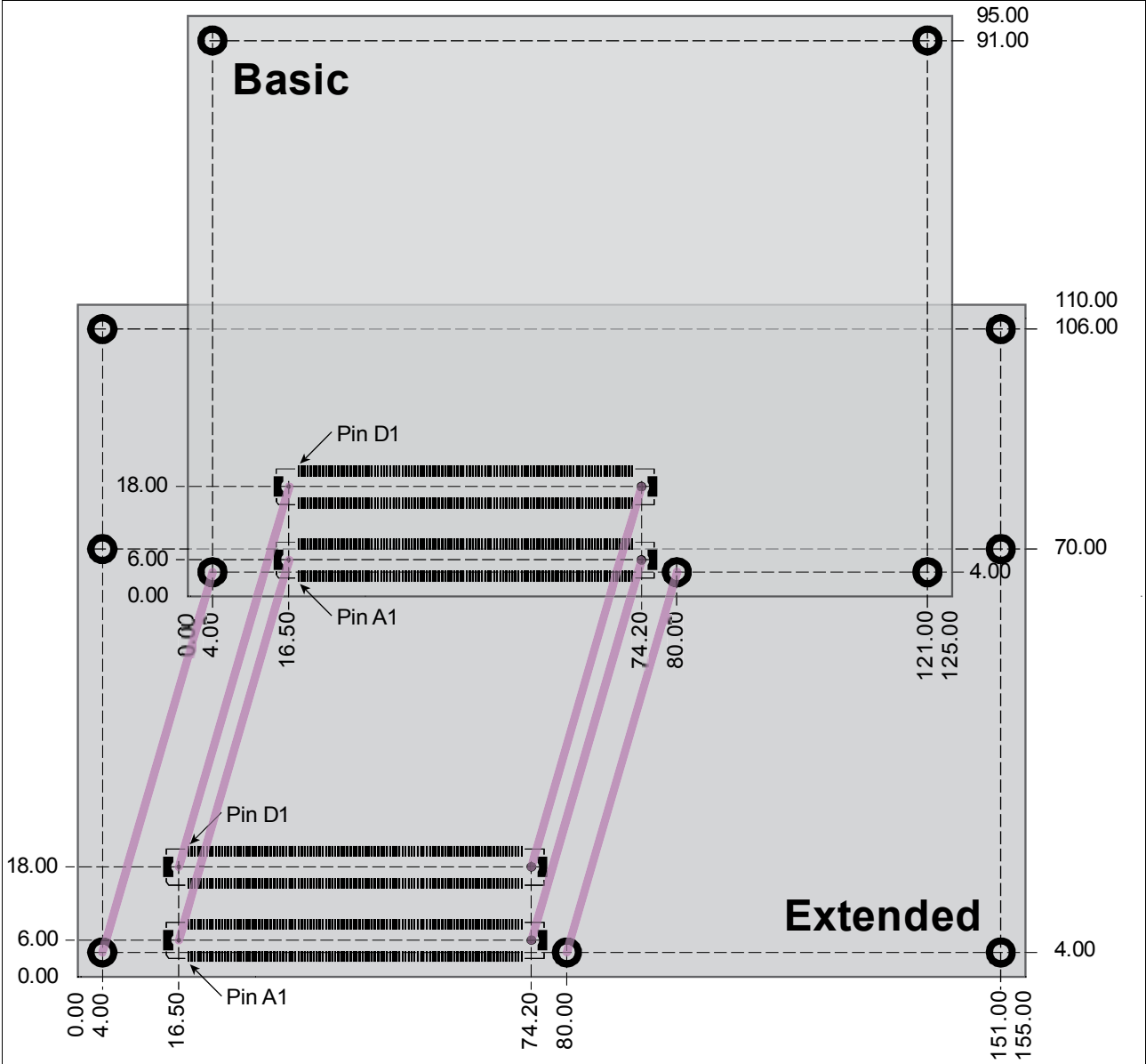
Figure 60: Mechanical comparison of available COM Express Form Factors
