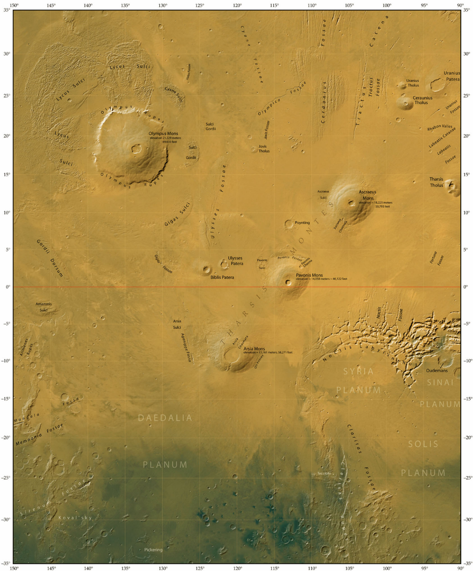
The Tharsis Quadrangle of Mars Shaded Relief with Albedo Color by Ralph Aeschliman Mercator projection
