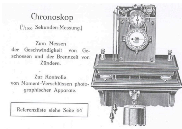
Figure 29: Löbner chronoscope, taken from the 1913 catalogue
