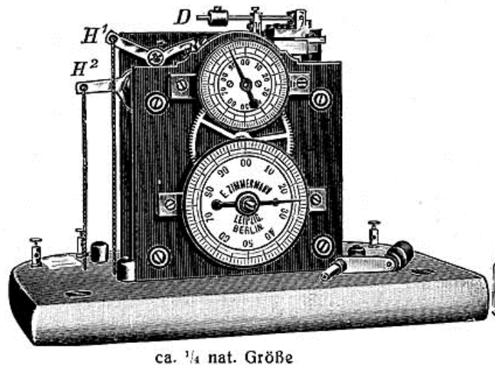
Figure 35: Differences between Hipp and Zimmermann chronoscope
