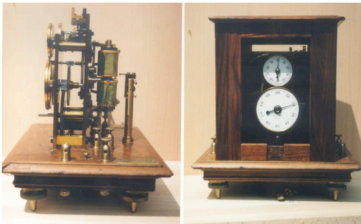
Figure 30: Löhnner chronoscope, private collection, with special unit for measuring the times of the electromagnet
