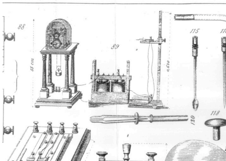
Figure 14: Hipp Chronoscope, "type 88," undated trade catalogue [84]
