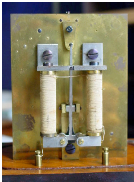
Figure 3 (b): Chronoscope (clockwork: backside) signed “M. Hipp in Reutlingen” (1849) Utrecht University Museum, Inventory No. ME-30 (Photograph by Jan Deimann)
